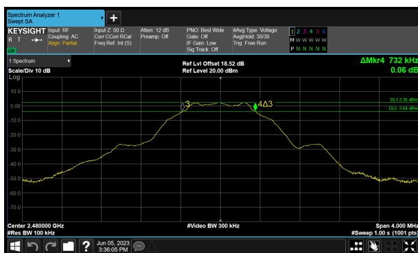
BT1 (1) 2480 MHz (CH39) 6 dB Bandwidth
