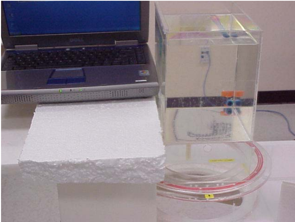
Photo 7. Right antenna bystander 5mm position
