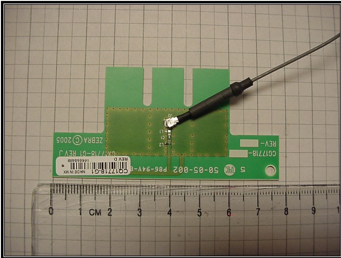
Photograph 5: Top of Antenna CQ17718-G1
