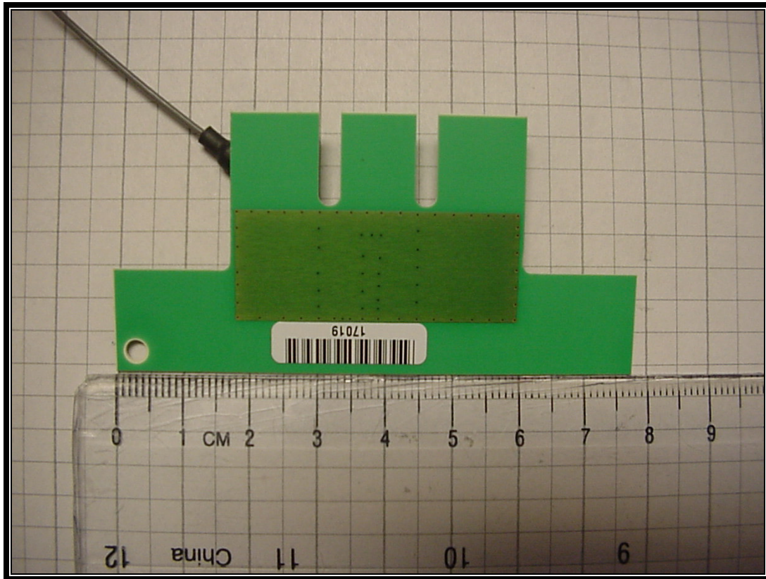
Photograph 6: Bottom of Antenna CQ17718-G1
