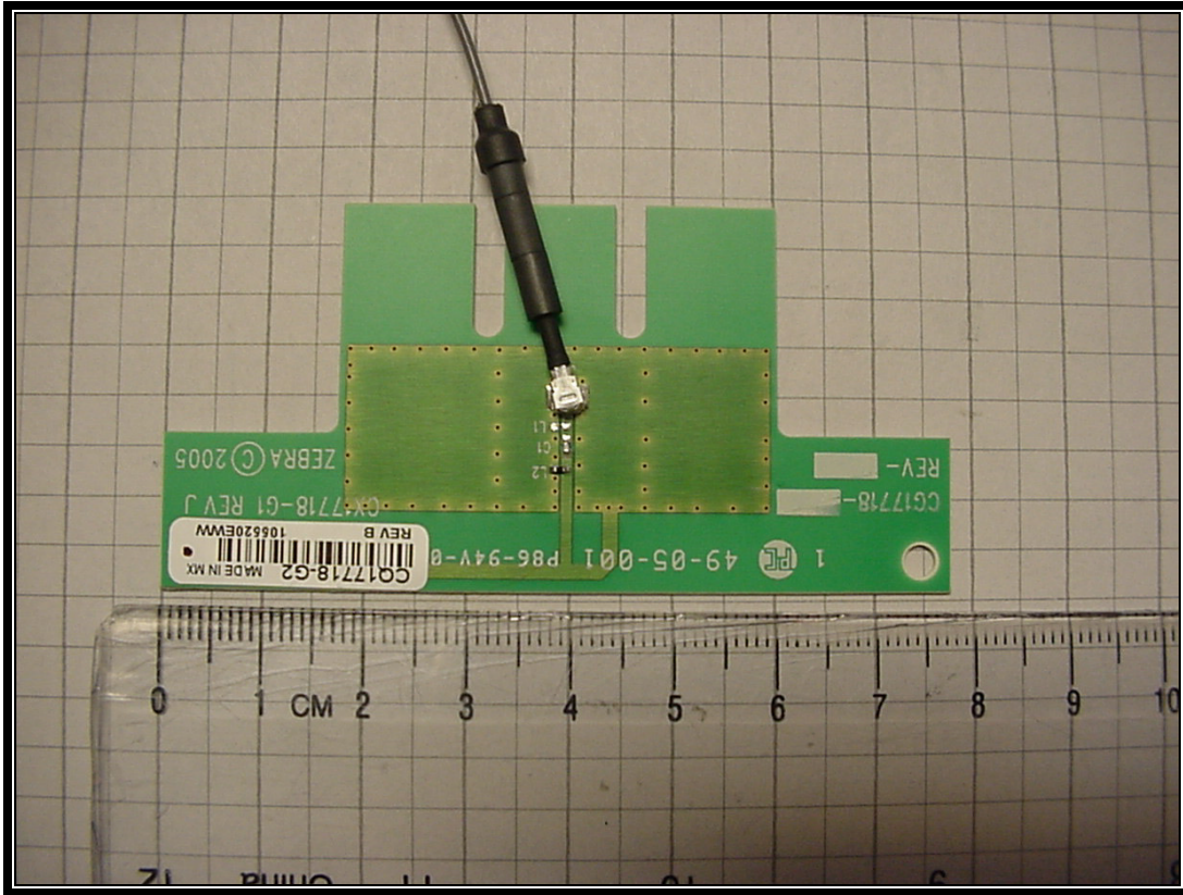
Photograph 7: Top of Antenna CQ17718-G2
