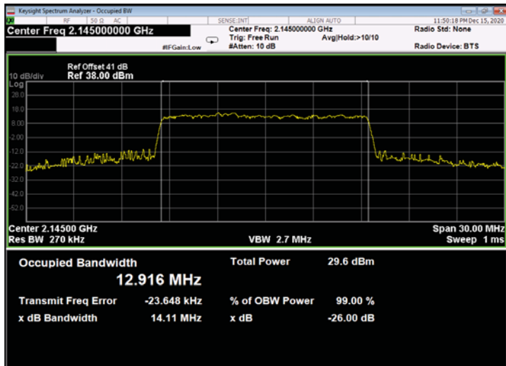
Figure 623: 64QAM 15MHz B.W.; 2145.0MHz, 60kHz - Output
