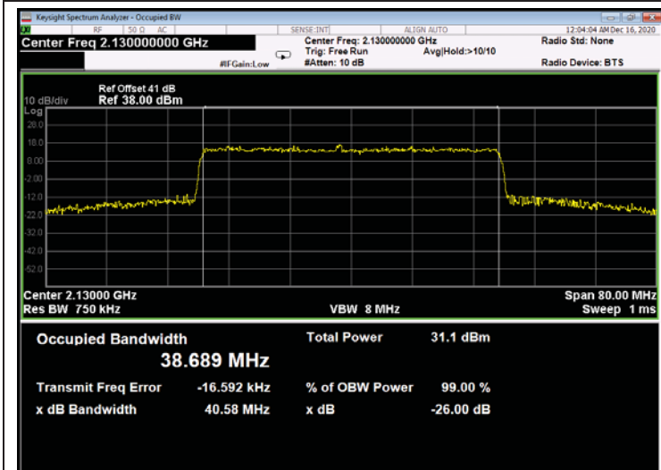
Figure 645: 64QAM 40MHz B.W.; 2130.0MHz, 15kHz – Output
