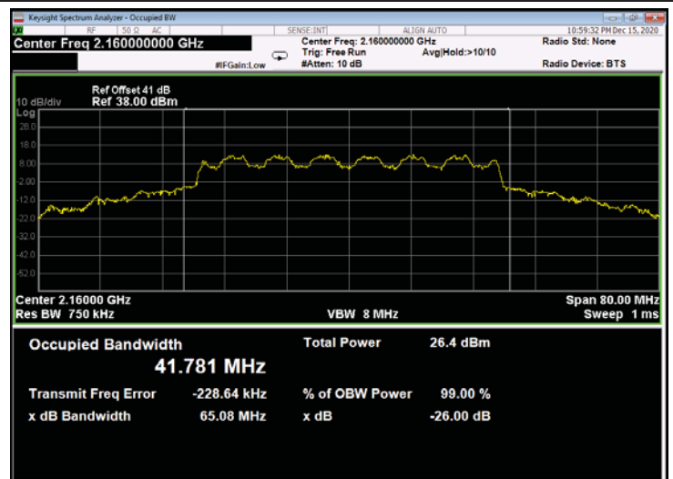
Figure 586: 16QAM 40MHz B.W.; 2160.0MHz, 30kHz - Output
