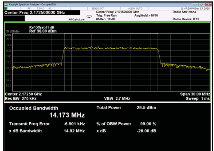
Figure 624: 64QAM 15MHz B.W.; 2172.5MHz, 15kHz - Output
