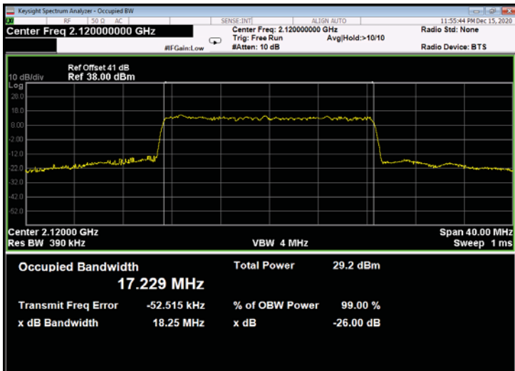
Figure 629: 64QAM 20MHz B.W.; 2120.0MHz, 60kHz - Output
