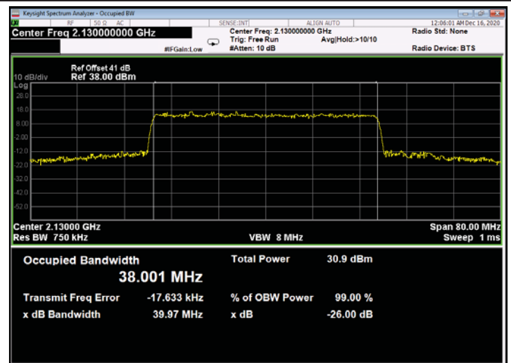
Figure 646: 64QAM 40MHz B.W.; 2130.0MHz, 30kHz - Output
