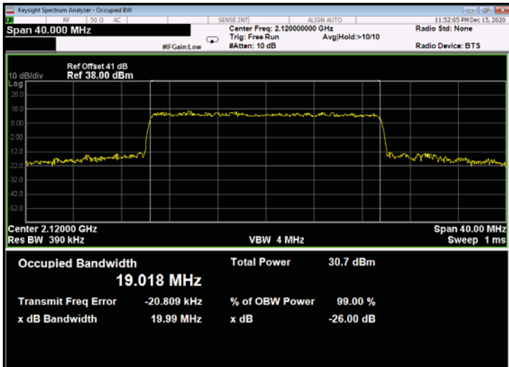
Figure 627: 64QAM 20MHz B.W.; 2120.0MHz, 15kHz - Output
