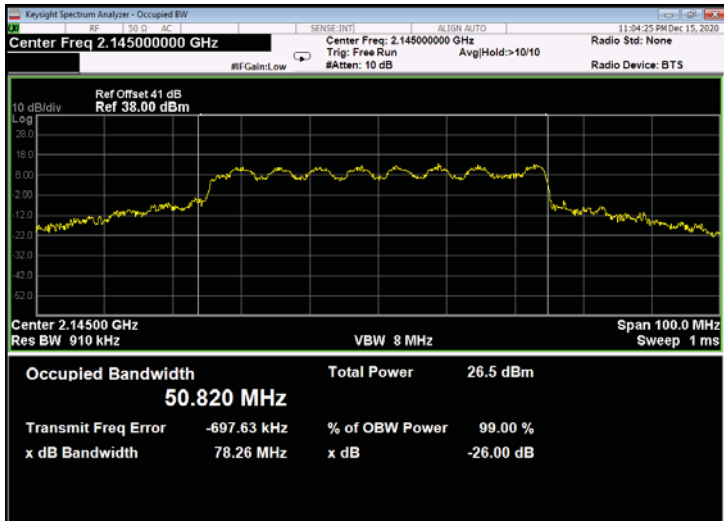
Figure 591: 16QAM 50MHz B.W.; 2145.0MHz, 15kHz - Output
