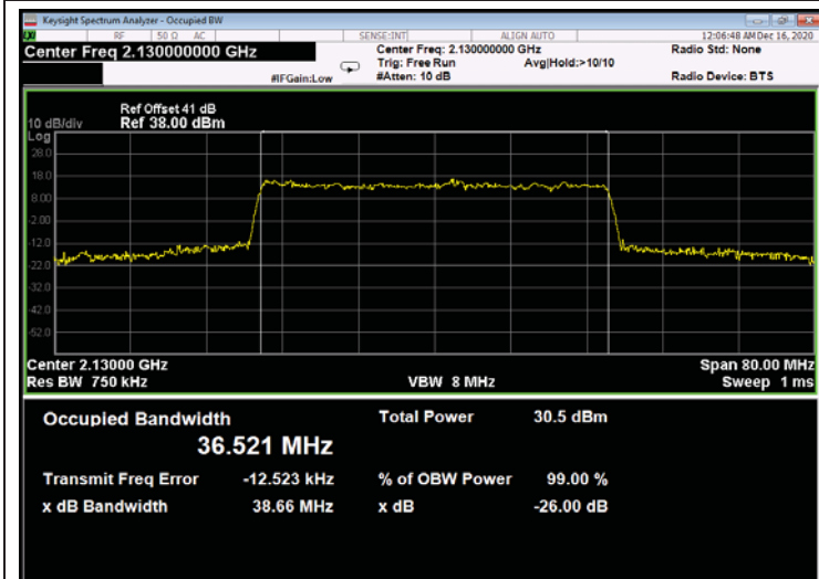
Figure 647: 64QAM 40MHz B.W.; 2130.0MHz, 60kHz - Output
