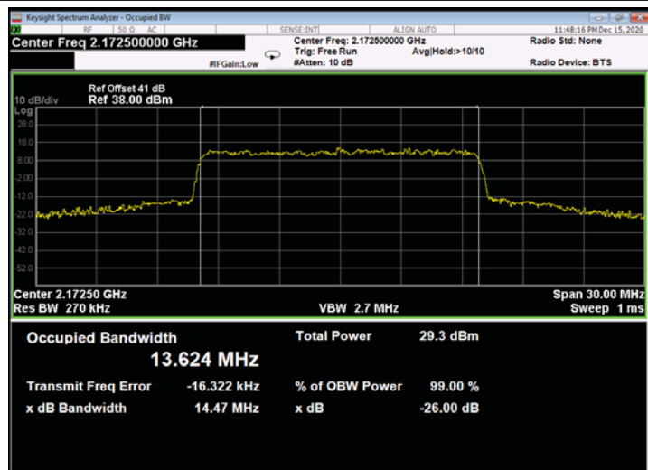
Figure 625: 64QAM 15MHz B.W.; 2172.5MHz, 30kHz - Output
