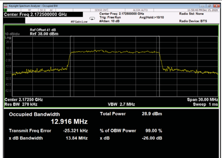
Figure 626: 64QAM 15MHz B.W.; 2172.5MHz, 60kHz - Output
