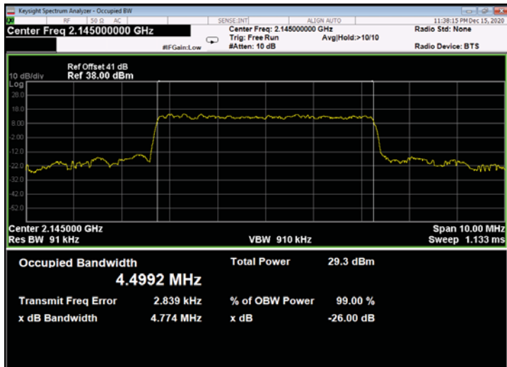
Figure 605: 64QAM 5MHz B.W.; 2145.0MHz, 15kHz - Output
