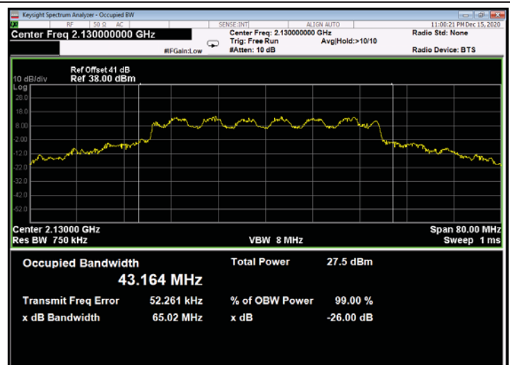
Figure 580: 16QAM 40MHz B.W.; 2130.0MHz, 30kHz - Output
