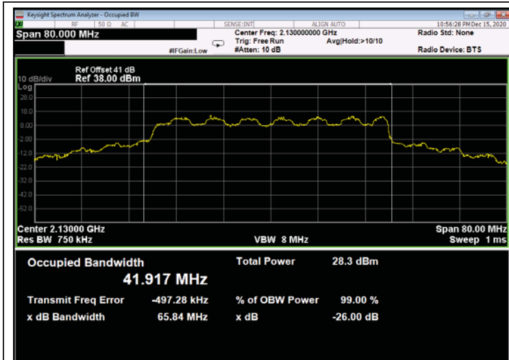
Figure 579: 16QAM 40MHz B.W.; 2130.0MHz, 15kHz - Output
