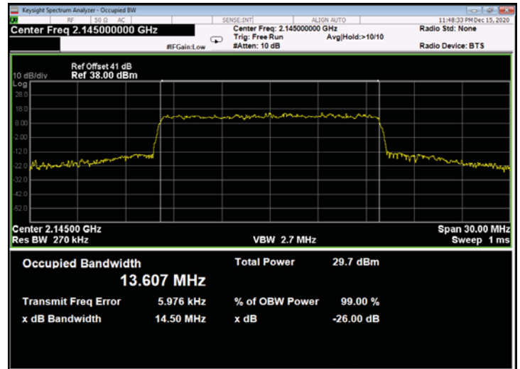
Figure 622: 64QAM 15MHz B.W.; 2145.0MHz, 30kHz - Output
