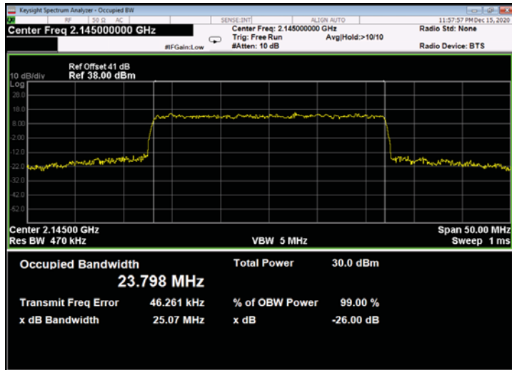
Figure 639: 64QAM 25MHz B.W.; 2145.0MHz, 15kHz - Output
