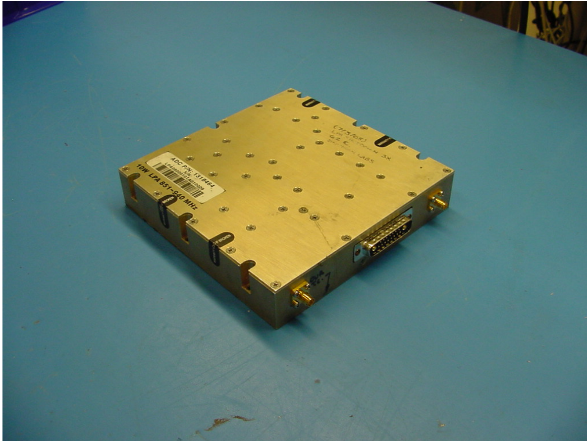
Digivance Street Coverage Solution (SCS) Bravo Tech Linear Power Amplifier - 10 Watt Right View
