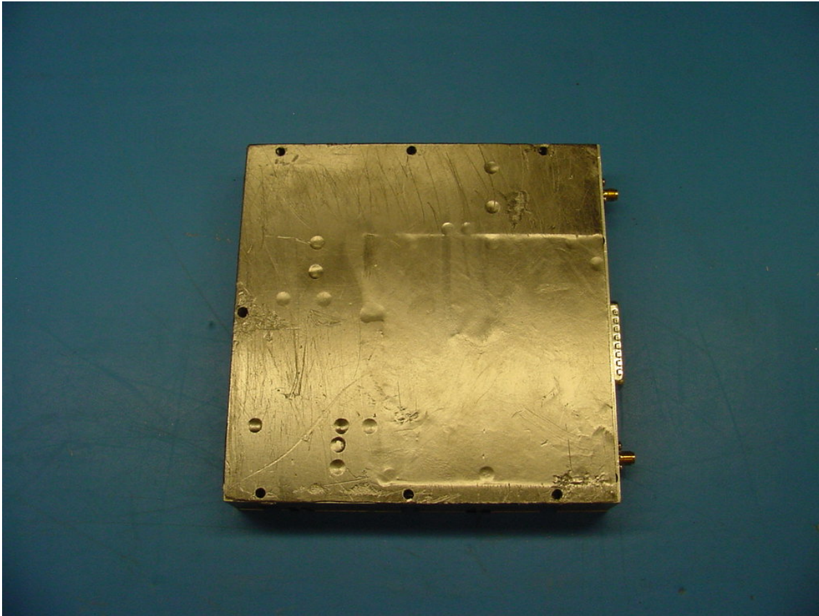
Digivance Street Coverage Solution (SCS) Bravo Tech Linear Power Amplifier - 10 Watt Bottom View
