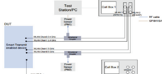
WLAN DBS Test setup - MIMO
