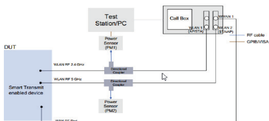
WLAN DBS Test Setup – SISO
