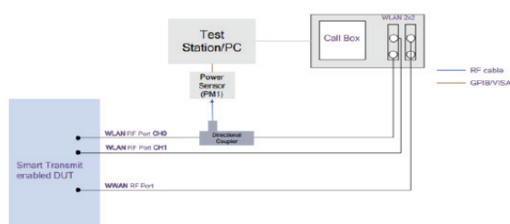
WLAN DBS Test setup - MIMO
