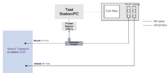
WLAN DBS Test Setup – SISO
