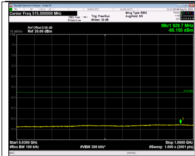
7-7-20MHz-20MHz-QPSK-QPSK-21152-21350-1RB#0-0 RB#0-30~1000MHz-PASS
