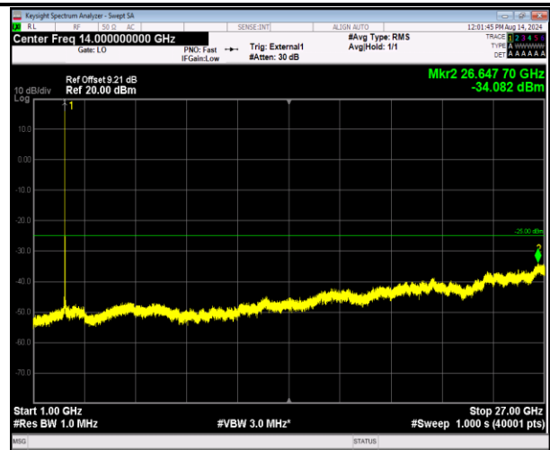
41-41-5MHz-20MHz-16QAM-16QAM-40648-40765-1RB#24 -ORB#0-1000~27000MHz-PASS
