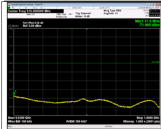
41-41-5MHz-20MHz-QPSK-QPSK-40273-40390-25RB#0 -100RB#0-30~1000MHz-PASS
