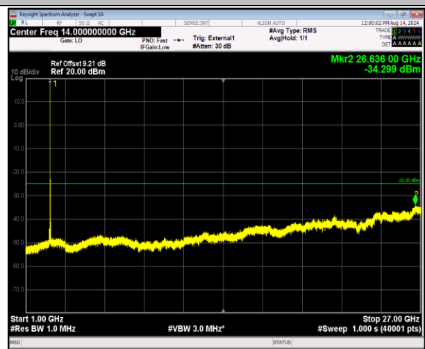
41-41-5MHz-20MHz-16QAM-16QAM-40648-40765-1RB#0- 0RB#0-1000~27000MHz-PASS
