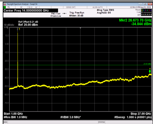
7-7-20MHz-20MHz-64QAM-64QAM-21152-21350-1RB#0-0 RB#0-1000~27000MHz-PASS
