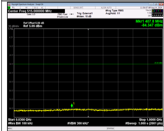
41-41-5MHz-20MHz-16QAM-16QAM-40273-40390-1RB# 0-1RB#99-30~1000MHz-PASS
