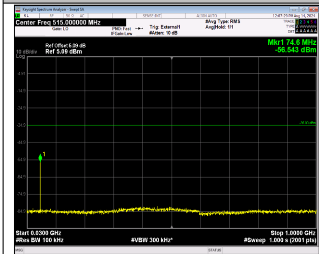
41-41-5MHz-20MHz-QPSK-QPSK-41023-41140-1RB#24-0-0RB#0-30~1000MHz-PASS
