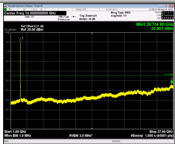
41-41-5MHz-20MHz-16QAM-16QAM-40273-40390-25RB#0 -100RB#0-1000~27000MHz-PASS
