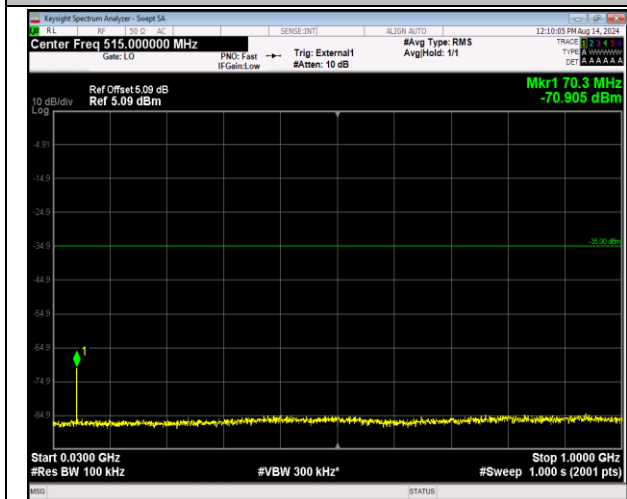
41-41-5MHz-20MHz-16QAM-16QAM-41023-41140-1RB# 0-1RB#99-30~1000MHz-PASS
