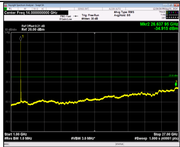
7-7-20MHz-20MHz-64QAM-64QAM-21001-21199-1RB#0-1 RB#99-1000~27000MHz-PASS
