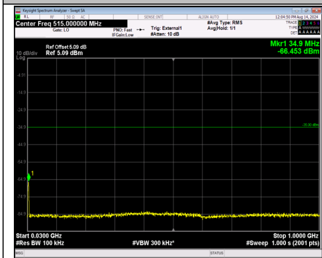
41-41-5MHz-20MHz-16QAM-16QAM-40648-40765-25RB# #0-100RB#0-30~1000MHz-PASS
