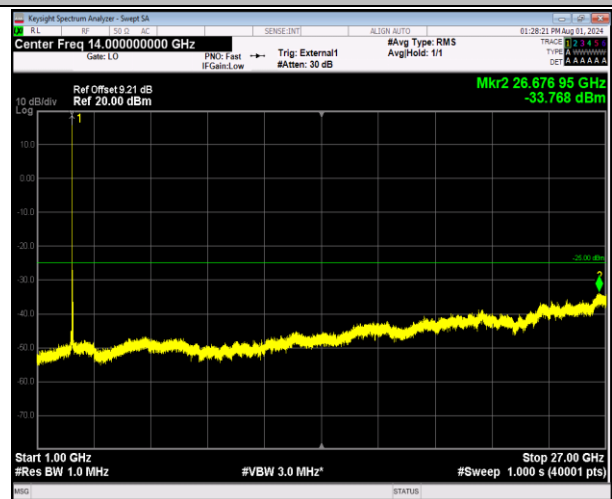
41-41-5MHz-20MHz-64QAM-64QAM-40648-40765-1RB#0- ORB#0-1000~27000MHz-PASS
