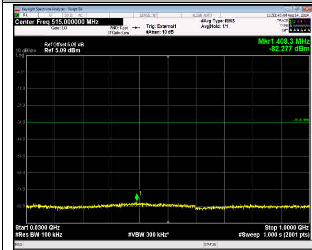
41-41-5MHz-20MHz-16QAM-16QAM-40273-40390-1RB# 0-0RB#0-30~1000MHz-PASS
