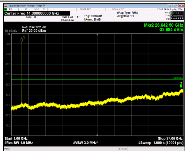
41-41-5MHz-20MHz-16QAM-16QAM-40648-40765-1RB#0- 1RB#99-1000~27000MHz-PASS
