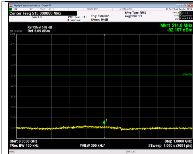
41-41-5MHz-20MHz-16QAM-16QAM-40273-40390-1RB# 24-ORB#0-30~1000MHz-PASS
