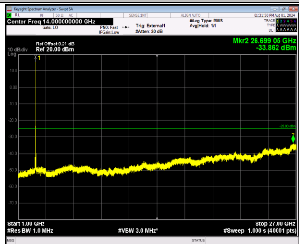
41-41-5MHz-20MHz-64QAM-64QAM-41023-41140-1RB#0- ORB#0-1000~27000MHz-PASS
