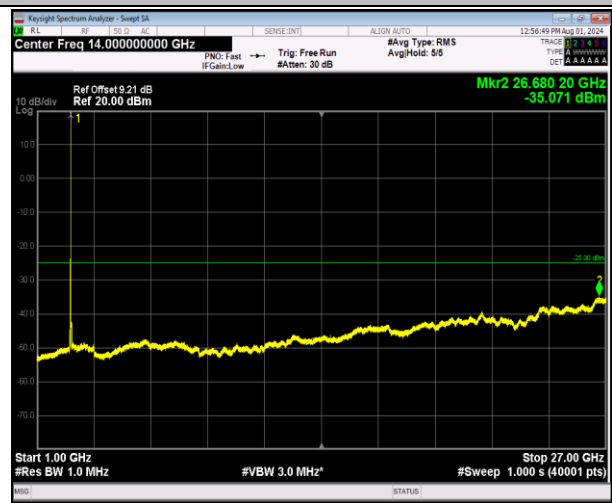
7-7-20MHz-20MHz-64QAM-64QAM-21152-21350-1RB#99- 0RB#0-1000~27000MHz-PASS
