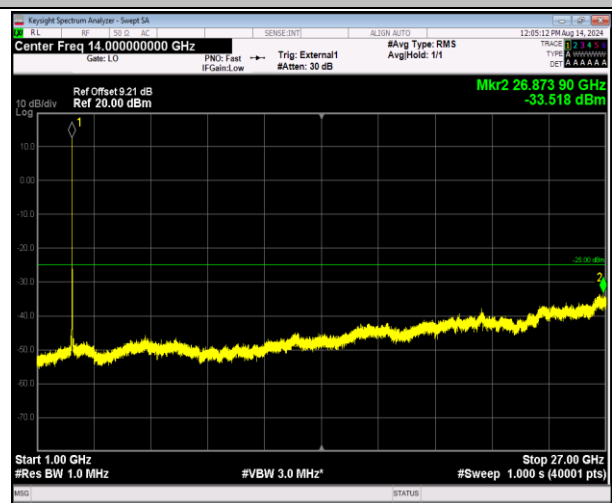
41-41-5MHz-20MHz-16QAM-16QAM-40648-40765-25RB#0 -100RB#0-1000~27000MHz-PASS
