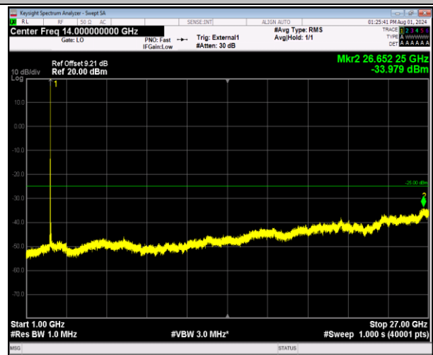
41-41-5MHz-20MHz-64QAM-64QAM-40273-40390-1RB#24 -0RB#0-1000~27000MHz-PASS
