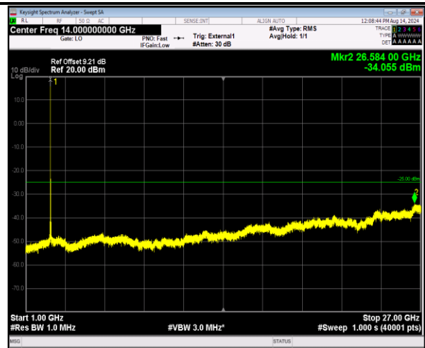
41-41-5MHz-20MHz-16QAM-16QAM-41023-41140-1RB#24 -ORB#0-1000~27000MHz-PASS
