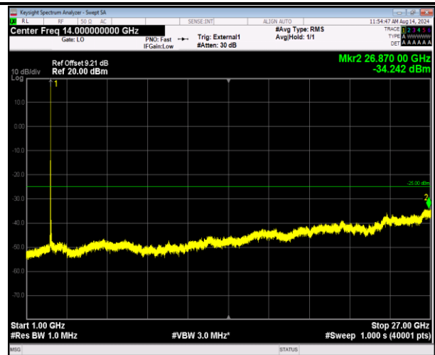
41-41-5MHz-20MHz-16QAM-16QAM-40273-40390-1RB#24 -ORB#0-1000~27000MHz-PASS
