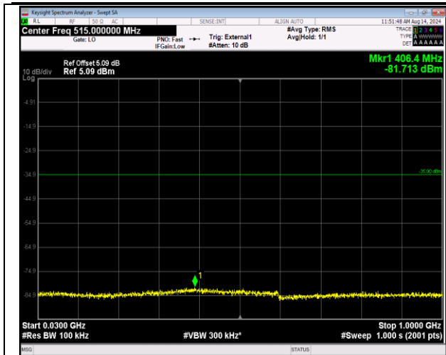
41-41-5MHz-20MHz-QPSK-QPSK-40273-40390-1RB#0-0RB#0-30~1000MHz-PASS
