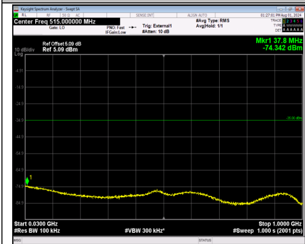
41-41-5MHz-20MHz-64QAM-64QAM-40273-40390-25RB #0-100RB#0-30~1000MHz-PASS
