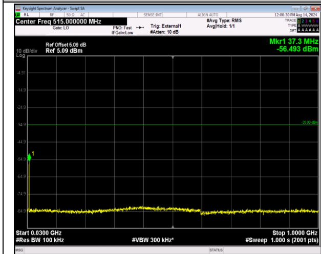
41-41-5MHz-20MHz-QPSK-QPSK-40648-40765-1RB#24-0-0RB#0-30~1000MHz-PASS
