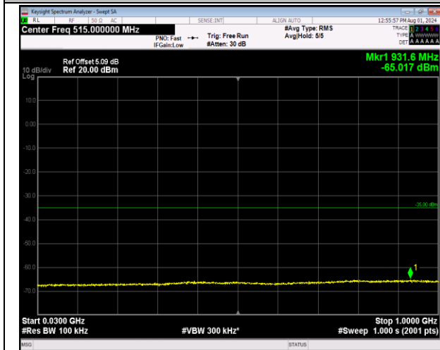
7-7-20MHz-20MHz-64QAM-64QAM-21152-21350-1RB#0 -ORB#0-30~1000MHz-PASS
