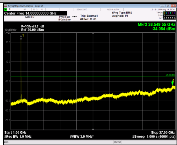
41-41-5MHz-20MHz-16QAM-16QAM-41023-41140-25RB#0 -100RB#0-1000~27000MHz-PASS
