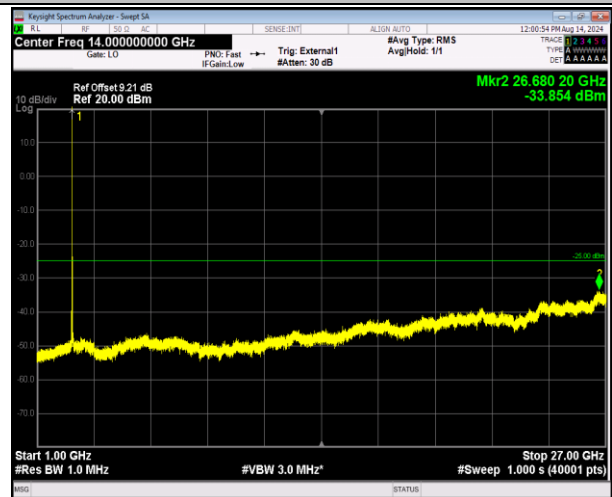
41-41-5MHz-20MHz-QPSK-QPSK-40648-40765-1RB#24-0RB#0-1000~27000MHz-PASS
