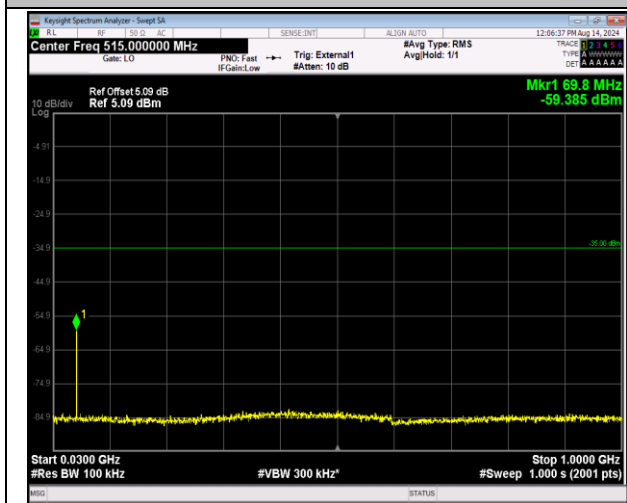
41-41-5MHz-20MHz-16QAM-16QAM-41023-41140-1RB# 0-0RB#0-30~1000MHz-PASS
