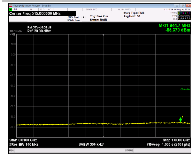
7-7-20MHz-20MHz-16QAM-16QAM-21001-21199-100RB #0-100RB#0-30~1000MHz-PASS
