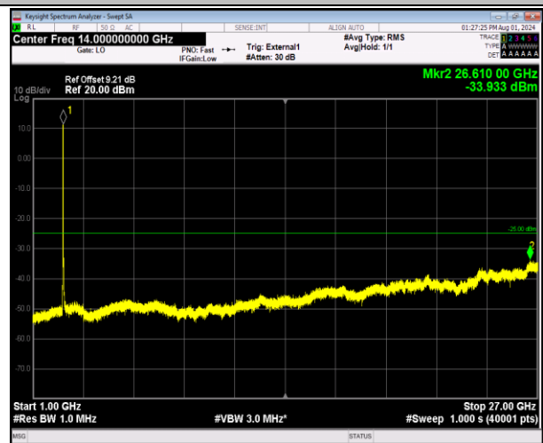
41-41-5MHz-20MHz-64QAM-64QAM-40273-40390-25RB#0 -100RB#0-1000~27000MHz-PASS
