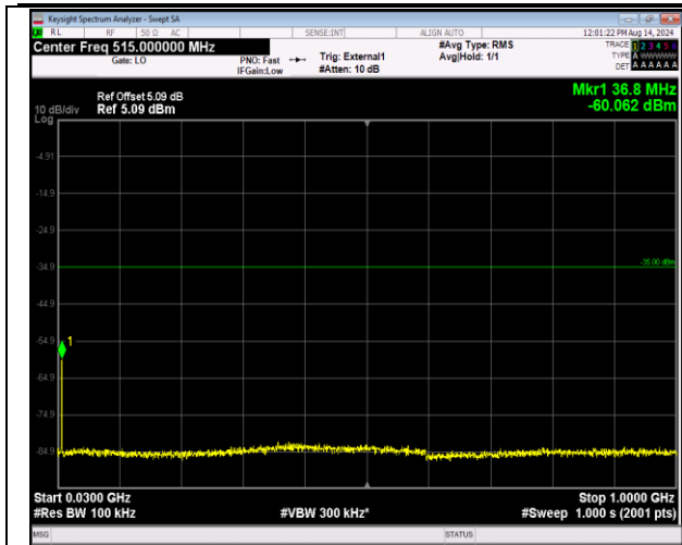
41-41-5MHz-20MHz-16QAM-16QAM-40648-40765-1RB# 24-ORB#0-30~1000MHz-PASS
