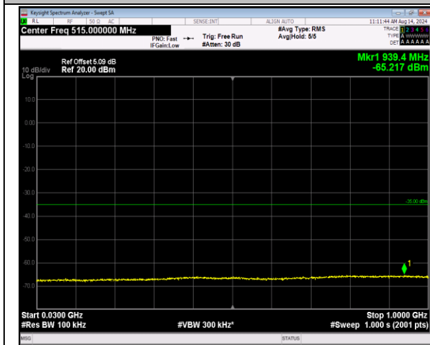
7-7-20MHz-20MHz-16QAM-16QAM-21152-21350-1RB#0 -0RB#0-30~1000MHz-PASS
