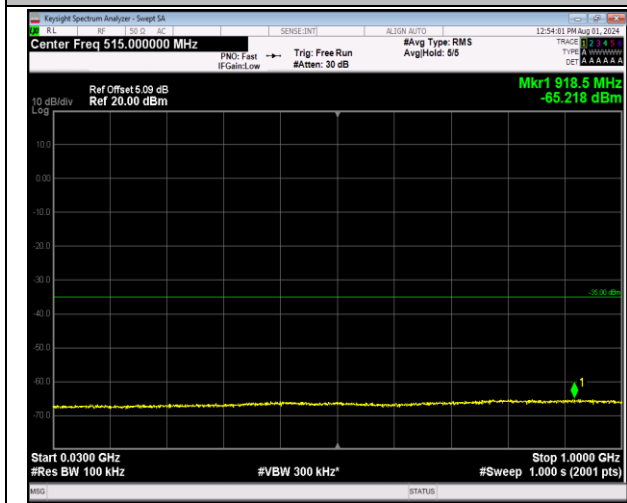
7-7-20MHz-20MHz-64QAM-64QAM-21001-21199-1RB#9 9-0RB#0-30~1000MHz-PASS
