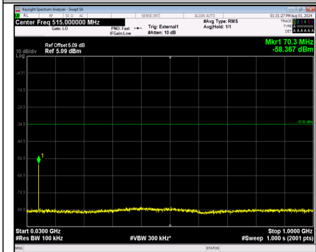
41-41-5MHz-20MHz-64QAM-64QAM-41023-41140-1RB# 0-ORB#0-30~1000MHz-PASS
