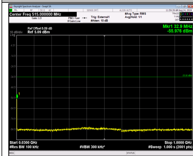
41-41-5MHz-20MHz-16QAM-16QAM-40648-40765-1RB# 0-0RB#0-30~1000MHz-PASS
