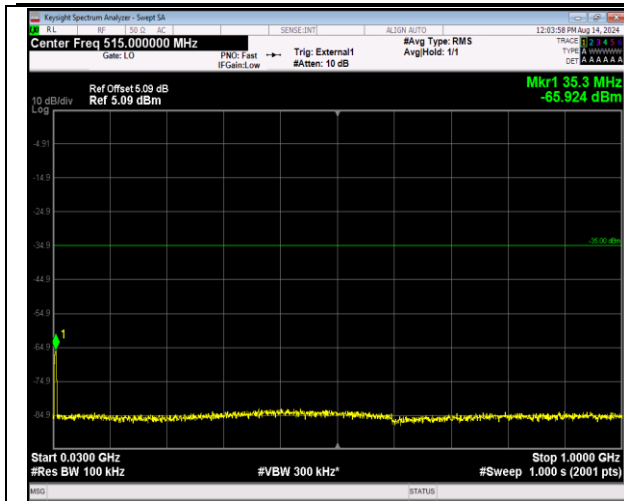
41-41-5MHz-20MHz-QPSK-QPSK-40648-40765-25RB#0 -100RB#0-30~1000MHz-PASS
