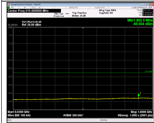
7-7-20MHz-20MHz-64QAM-64QAM-21152-21350-1RB#9 9-0RB#0-30~1000MHz-PASS
