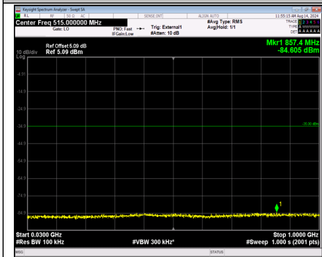
41-41-5MHz-20MHz-QPSK-QPSK-40273-40390-1RB#0-01RB#99-30~1000MHz-PASS
