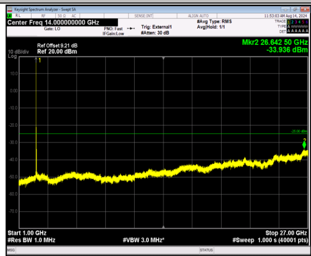
41-41-5MHz-20MHz-16QAM-16QAM-40273-40390-1RB#0- 0RB#0-1000~27000MHz-PASS
