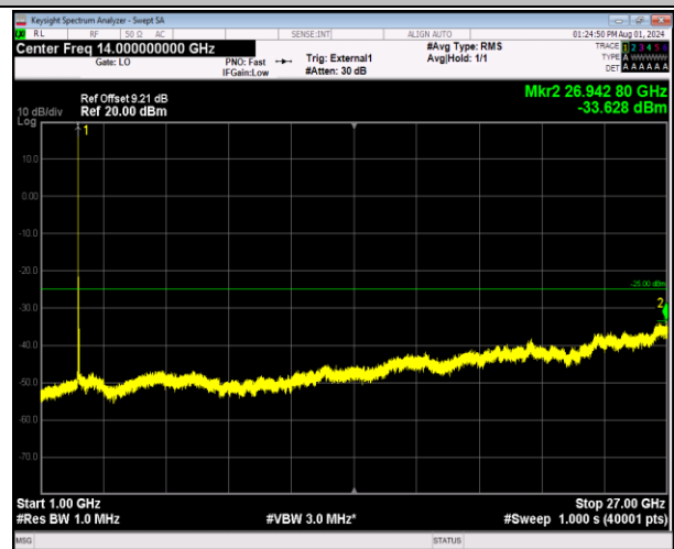
41-41-5MHz-20MHz-64QAM-64QAM-40273-40390-1RB#0- ORB#0-1000~27000MHz-PASS
