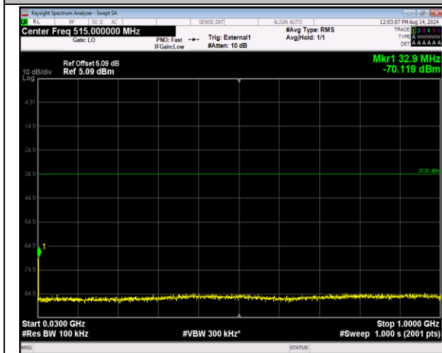
41-41-5MHz-20MHz-16QAM-16QAM-40648-40765-1RB# 0-1RB#99-30~1000MHz-PASS
