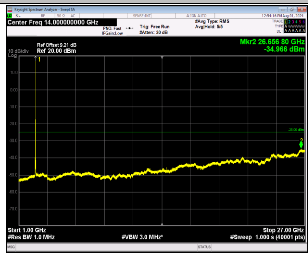
7-7-20MHz-20MHz-64QAM-64QAM-21001-21199-1RB#99- 0RB#0-1000~27000MHz-PASS
