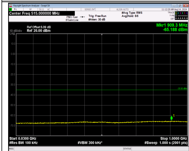
7-7-20MHz-20MHz-QPSK-QPSK-21152-21350-1RB#99-99 ORB#0-30~1000MHz-PASS
