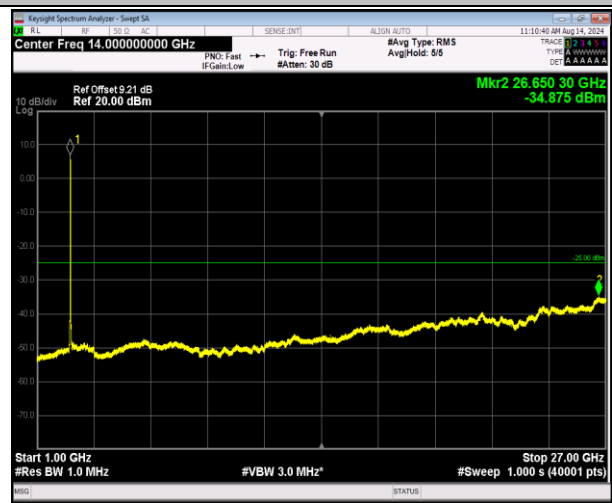
7-7-20MHz-20MHz-16QAM-16QAM-21001-21199-100RB#0 -100RB#0-1000~27000MHz-PASS
