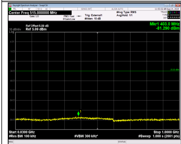
41-41-5MHz-20MHz-QPSK-QPSK-40273-40390-1RB#24-0-0RB#0-30~1000MHz-PASS
