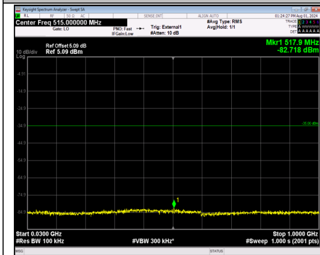
41-41-5MHz-20MHz-64QAM-64QAM-40273-40390-1RB# 0-ORB#0-30~1000MHz-PASS
