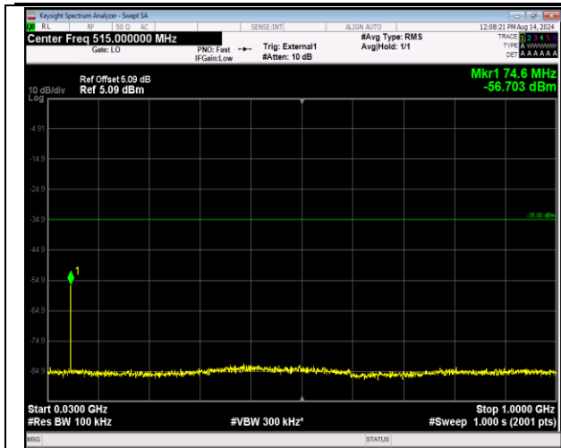
41-41-5MHz-20MHz-16QAM-16QAM-41023-41140-1RB# 24-ORB#0-30~1000MHz-PASS
