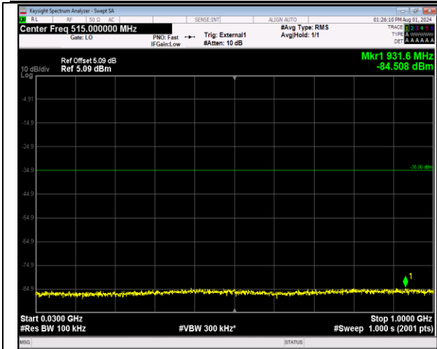
41-41-5MHz-20MHz-64QAM-64QAM-40273-40390-1RB# 0-1RB#99-30~1000MHz-PASS
