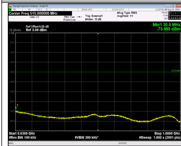
41-41-5MHz-20MHz-16QAM-16QAM-40273-40390-25RB #0-100RB#0-30~1000MHz-PASS
