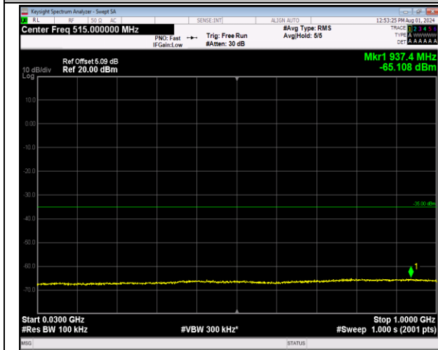
7-7-20MHz-20MHz-64QAM-64QAM-21001-21199-1RB#0 -ORB#0-30~1000MHz-PASS
