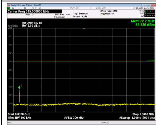
41-41-5MHz-20MHz-16QAM-16QAM-41023-41140-25RB #0-100RB#0-30~1000MHz-PASS
