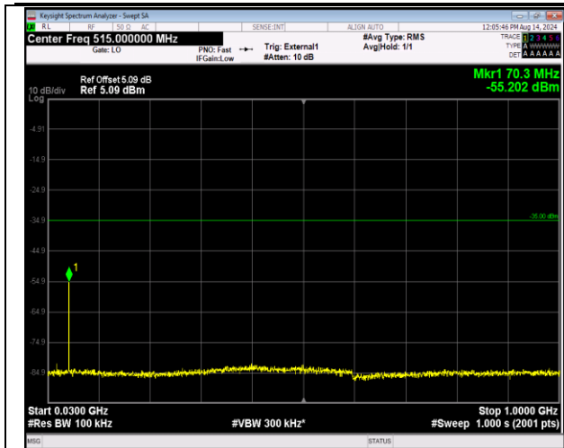
41-41-5MHz-20MHz-QPSK-QPSK-41023-41140-1RB#0-0RB#0-30~1000MHz-PASS
