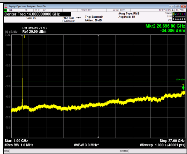
41-41-5MHz-20MHz-16QAM-16QAM-41023-41140-1RB#0- 0RB#0-1000~27000MHz-PASS
