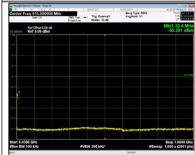
41-41-5MHz-20MHz-64QAM-64QAM-40648-40765-1RB# 0-ORB#0-30~1000MHz-PASS
