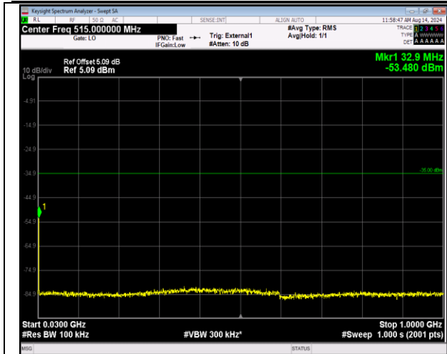
41-41-5MHz-20MHz-QPSK-QPSK-40648-40765-1RB#0-0RB#0-30~1000MHz-PASS
