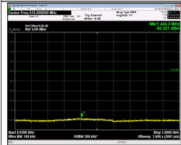
41-41-5MHz-20MHz-64QAM-64QAM-40273-40390-1RB# 24-0RB#0-30~1000MHz-PASS
