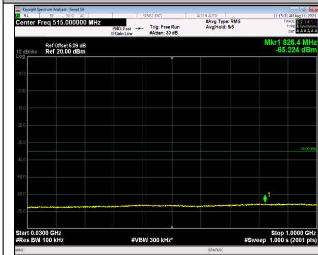
7-7-20MHz-20MHz-16QAM-16QAM-21152-21350-100RB #0-100RB#0-30~1000MHz-PASS
