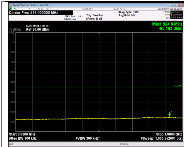
7-7-20MHz-20MHz-64QAM-64QAM-21001-21199-1RB#0 -1RB#99-30~1000MHz-PASS
