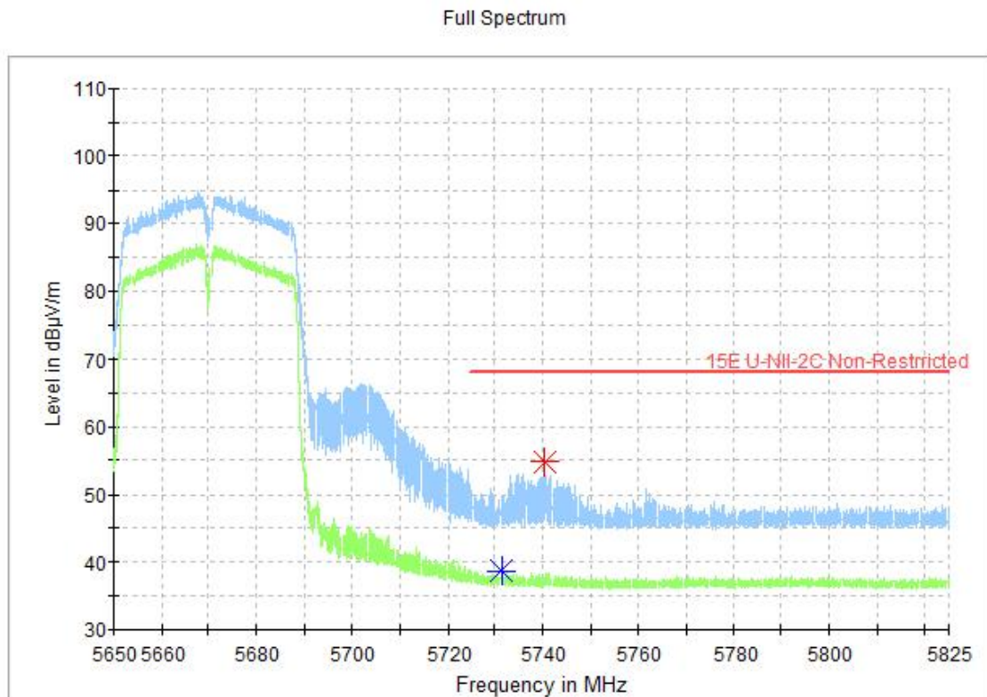
Fig.12 Band Edges (802.11n-HT40 Ch134, 5670MHz)
