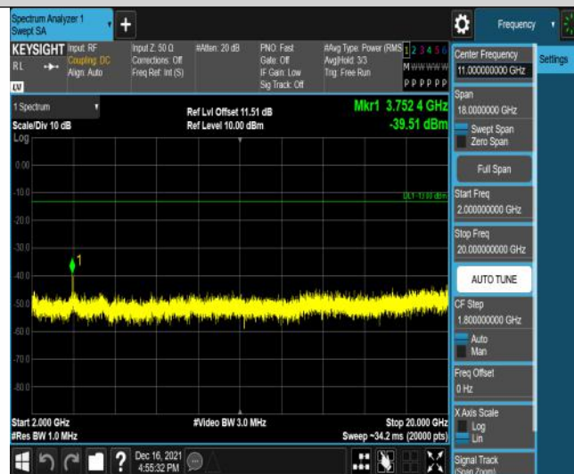
Band2-15MHz-16QAM-18900-75RB#0-Range3:2000~20000MHz
