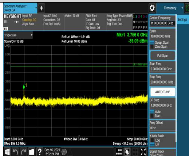
Band2-20MHz-QPSK-18900-100RB#0-Range3:2000~20000MHz
