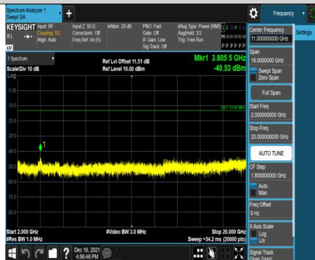
Band2-15MHz-16QAM-19125-75RB#0-Range3:2000~20000MHz
