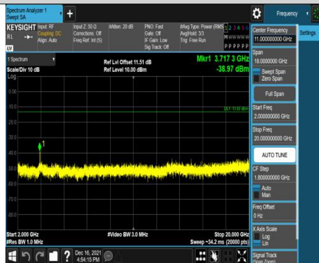
Band2-15MHz-16QAM-18675-75RB#0-Range3:2000~20000MHz
