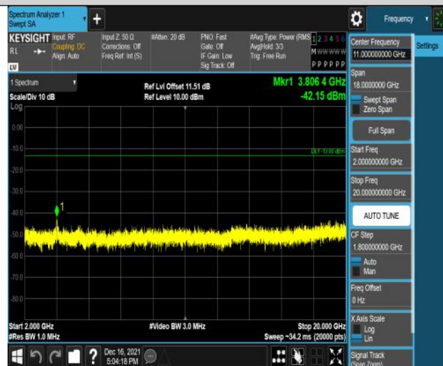
Band2-20MHz-16QAM-19100-100RB#0-Range3:2000~20000MHz
