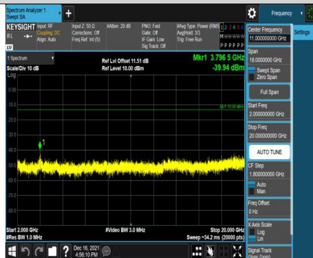
Band2-15MHz-QPSK-19125-75RB#0-Range3:2000~20000MHz
