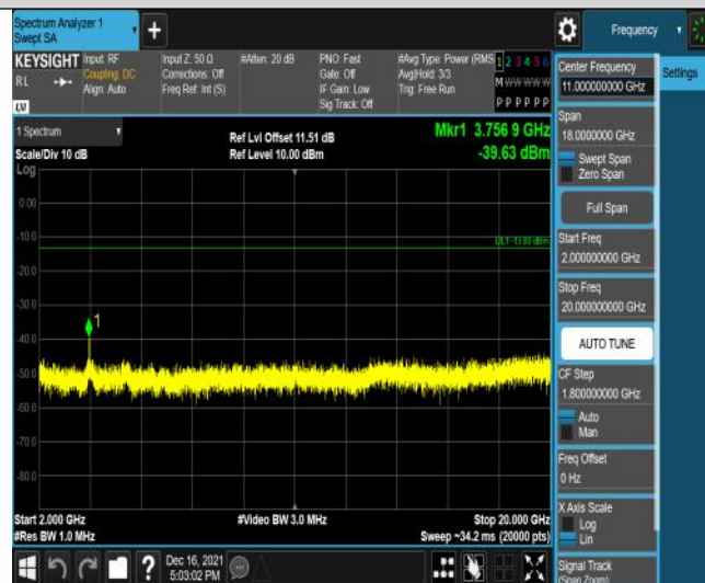
Band2-20MHz-16QAM-18900-100RB#0-Range3:2000~20000MHz
