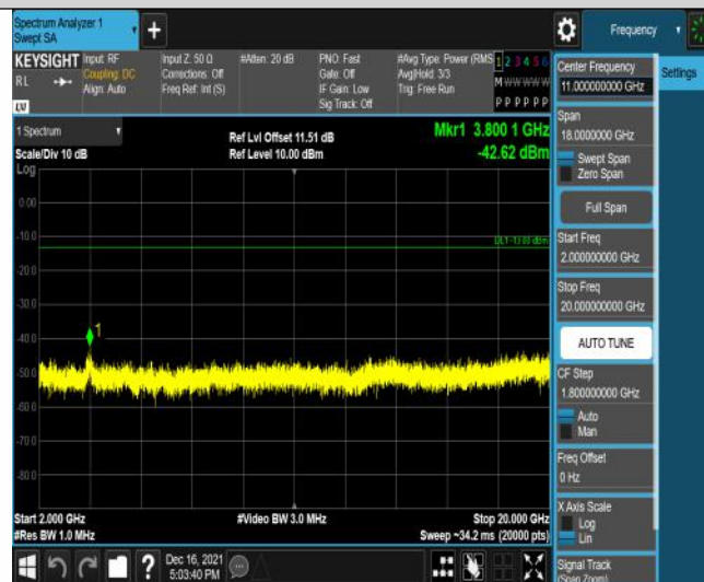
Band2-20MHz-QPSK-19100-100RB#0-Range3:2000~20000MHz
