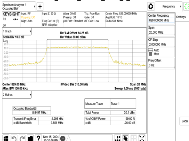
Band5_10MHz_64QAM_RB50_0_CH20450
