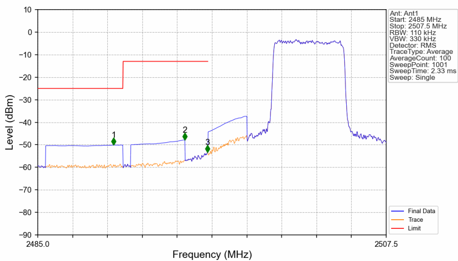
Band7_5MHz_16QAM_LCH_2502.5MHz_RB_25_0_NTNV
