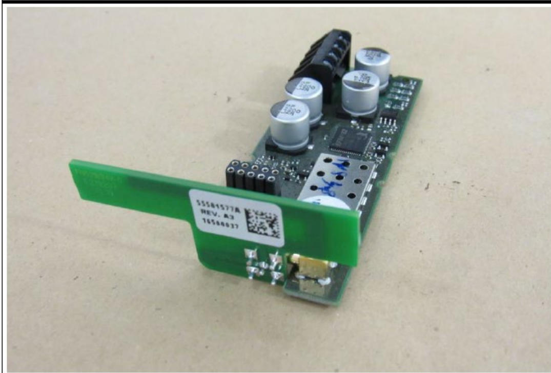
radio module with internal antenna
