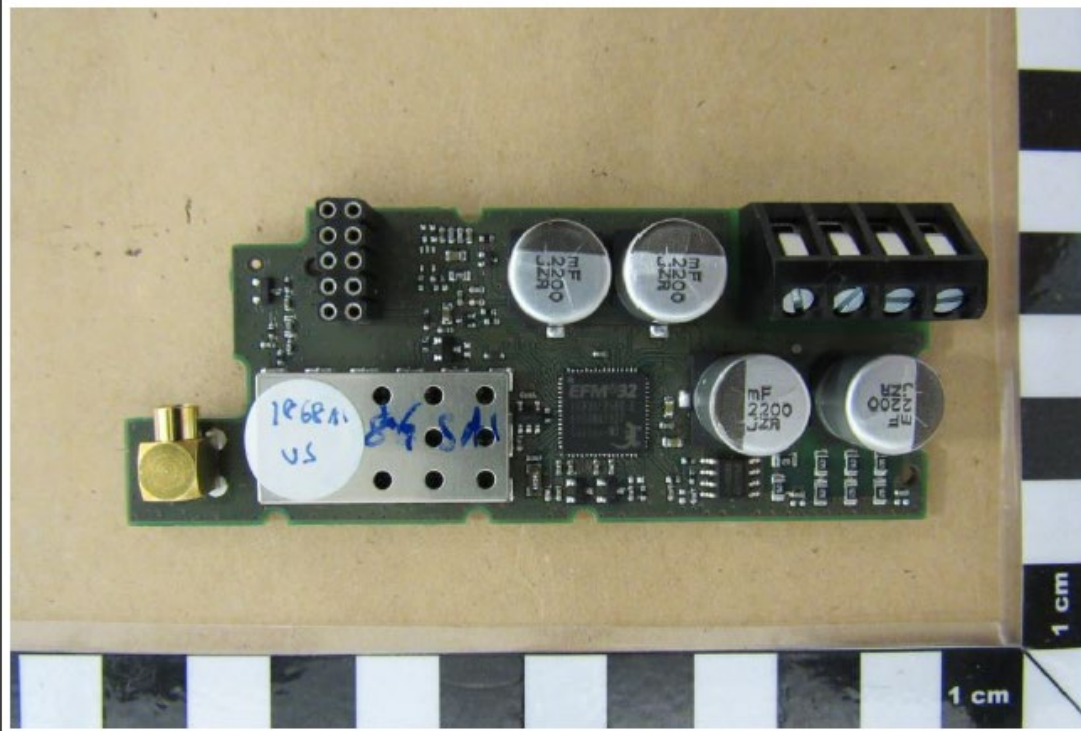
5550 1868 A3 (radio module, top view)
