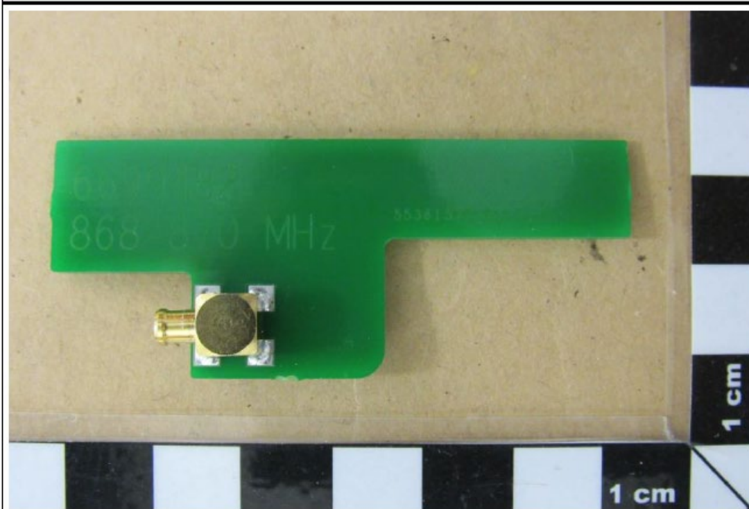
internal antenna (6699482 B3), bottom view
