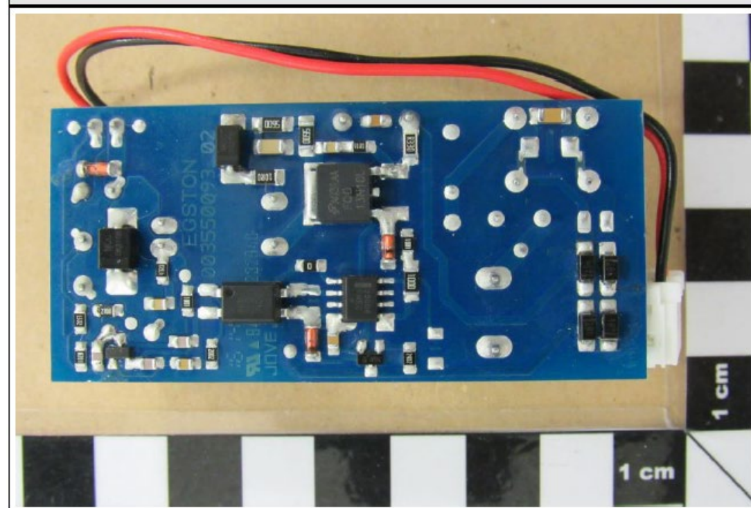
24 VAC smps supply bottom view (60200004000000 A4)
