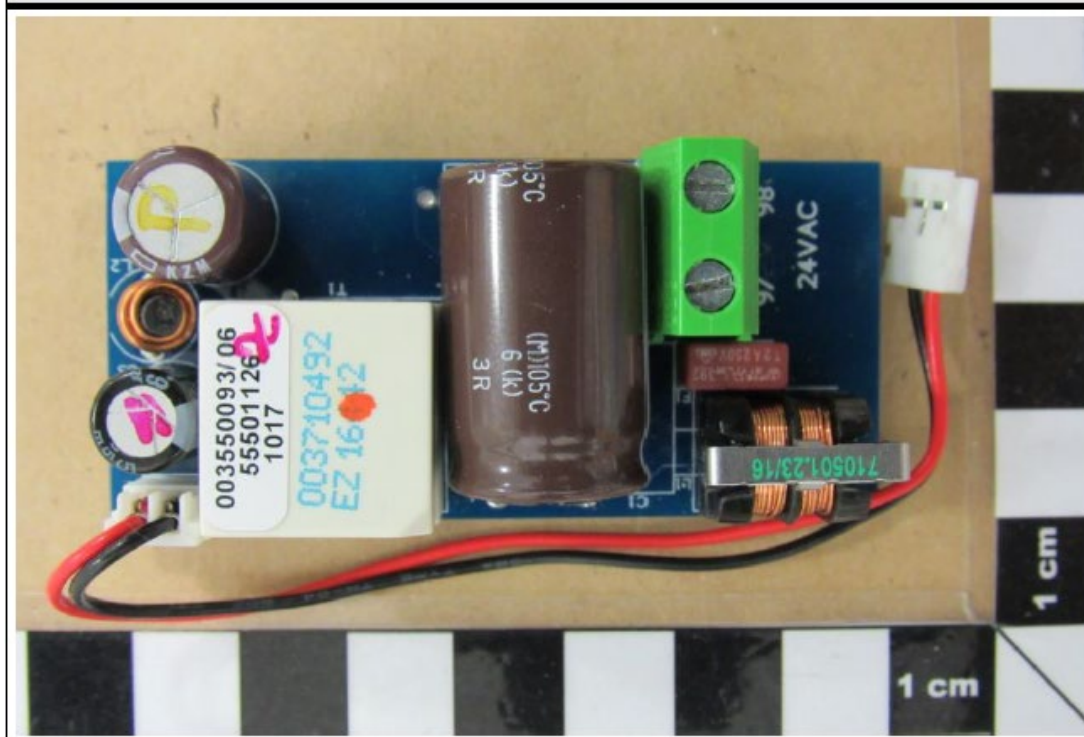
24 VAC smps supply top view (60200004000000 A4)
