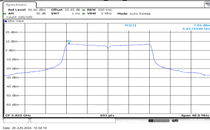
11A-CDD_Ant4_5825
