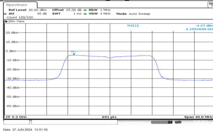
11A-CDD_Ant4_5200
