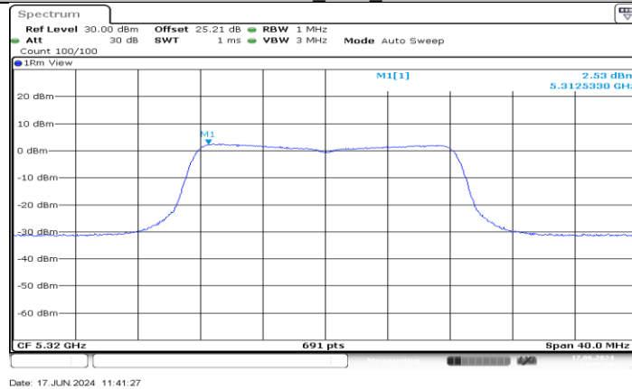
11A-CDD_Ant4_5320
