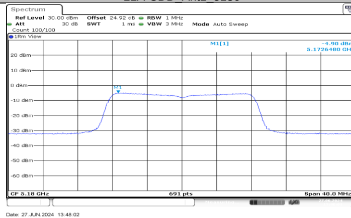
11A-CDD Ant2 5180
