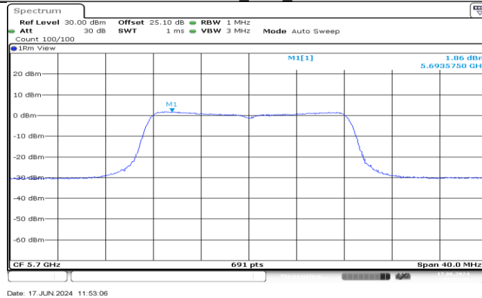
11A-CDD_Ant4_5700
