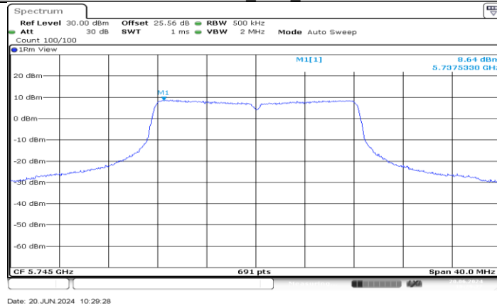
11A-CDD_Ant3_5745
