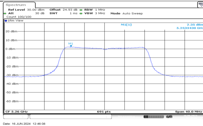
11A-CDD_Ant4_5260
