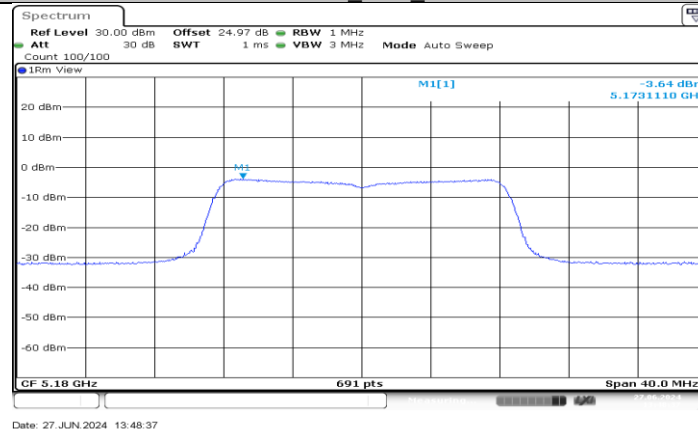
11A-CDD Ant3 5180
