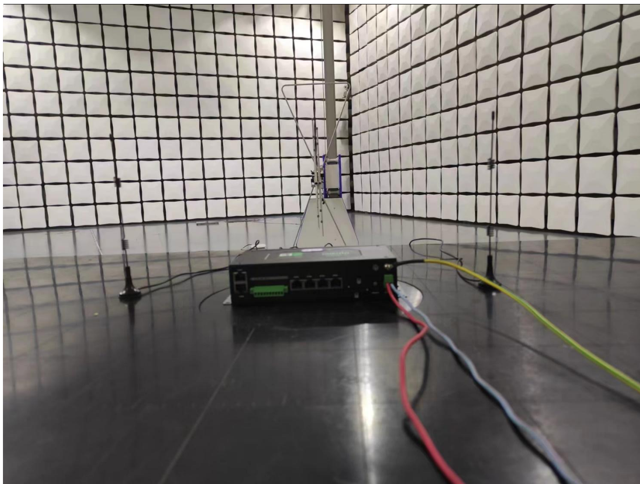
30MHz~1GHz
