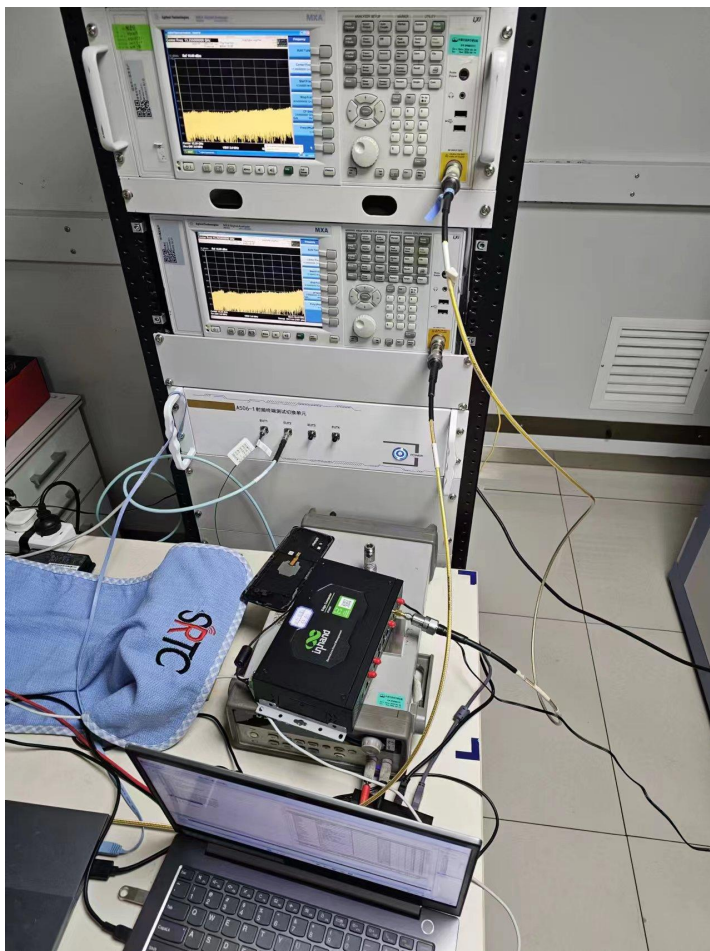
RF Conducted Test setup (WIFI)
