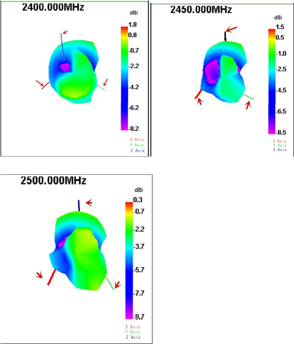
方向图/Directional map:
