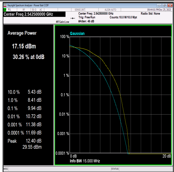
41(2535-2655)-15MHz-16QAM-40115-75RB#0-PASS
