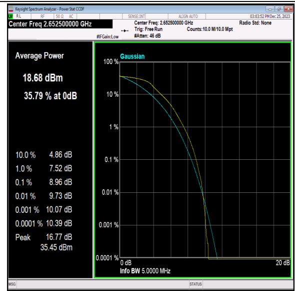
41(2535-2655)-5MHz-64QAM-41215-25RB#0-PASS
