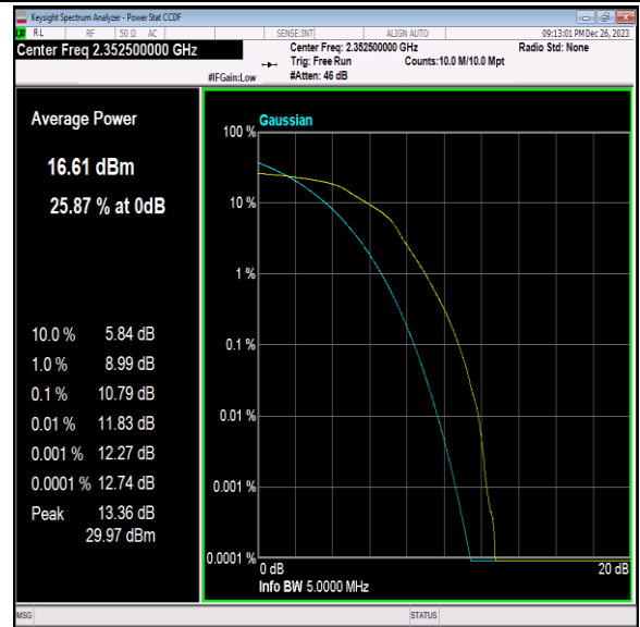
40(2350-2360)-5MHz-16QAM-39175-25RB#0-PASS
