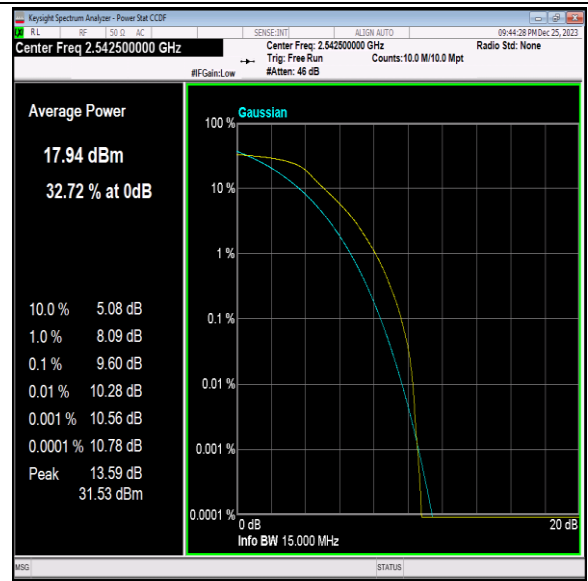
41(2535-2655)-15MHz-64QAM-40115-75RB#0-PASS
