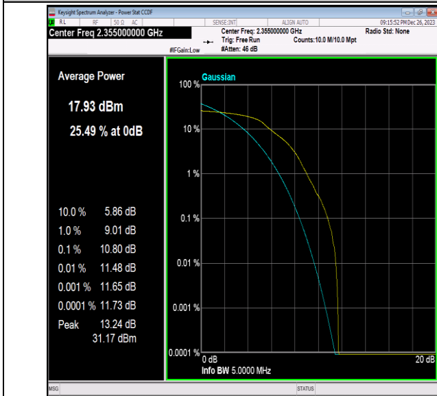
40(2350-2360)-5MHz-64QAM-39200-1RB#0-PASS
