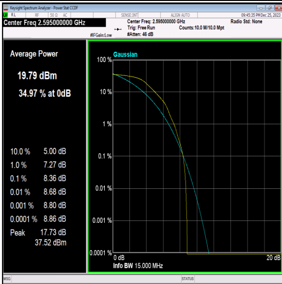
41(2535-2655)-15MHz-64QAM-40640-1RB#0-PASS
