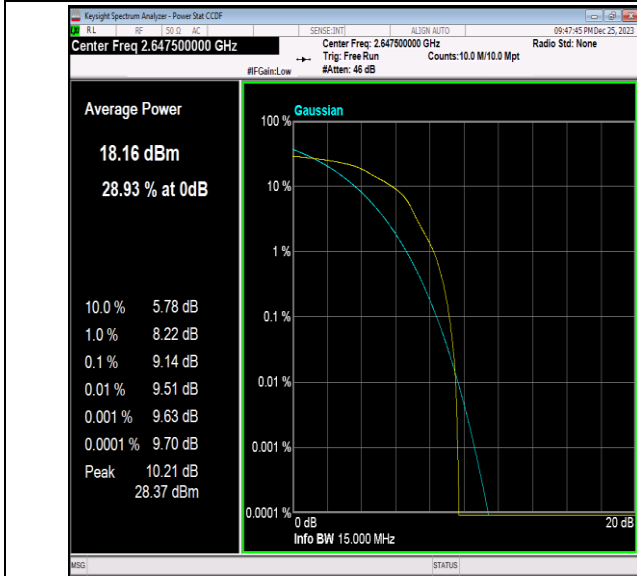
41(2535-2655)-15MHz-16QAM-41165-1RB#0-PASS
