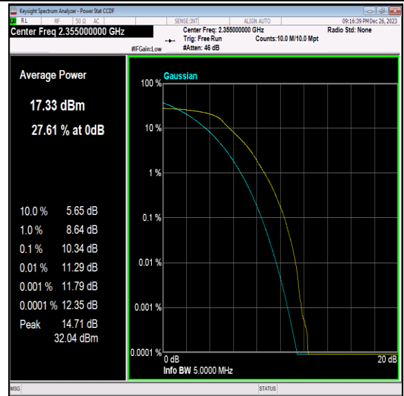
40(2350-2360)-5MHz-QPSK-39200-25RB#0-PASS
