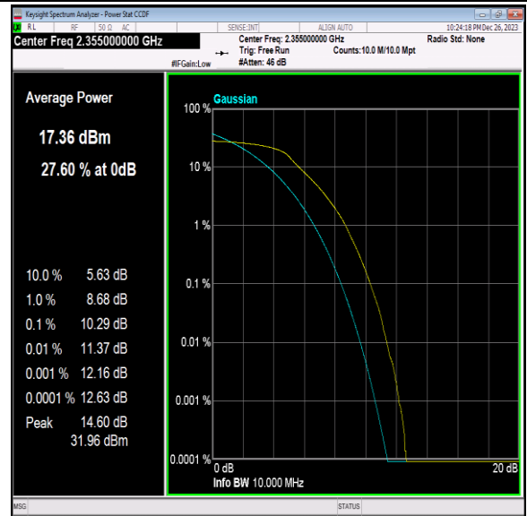
40(2350-2360)-10MHz-64QAM-39200-50RB#0-PASS
