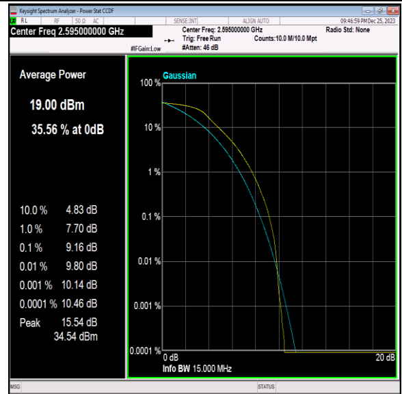
41(2535-2655)-15MHz-64QAM-40640-75RB#0-PASS
