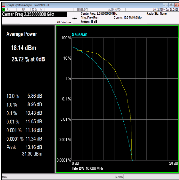
40(2350-2360)-10MHz-64QAM-39200-1RB#0-PASS
