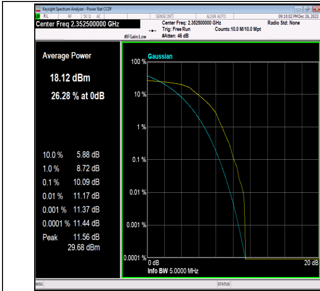
40(2350-2360)-5MHz-QPSK-39175-1RB#0-PASS
