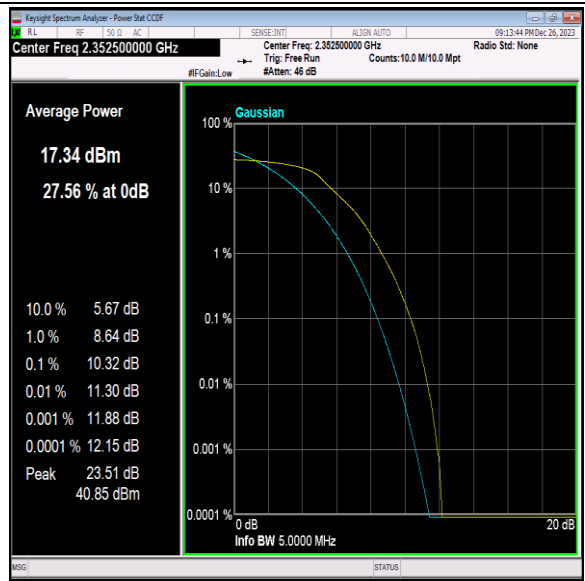
40(2350-2360)-5MHz-64QAM-39175-25RB#0-PASS
