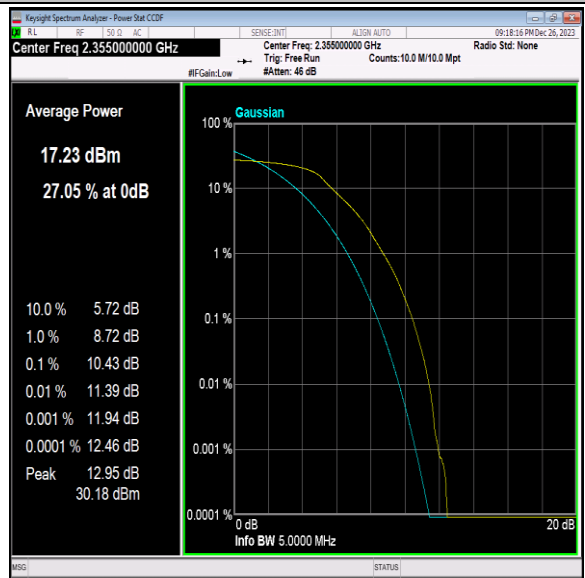
40(2350-2360)-5MHz-64QAM-39200-25RB#0-PASS
