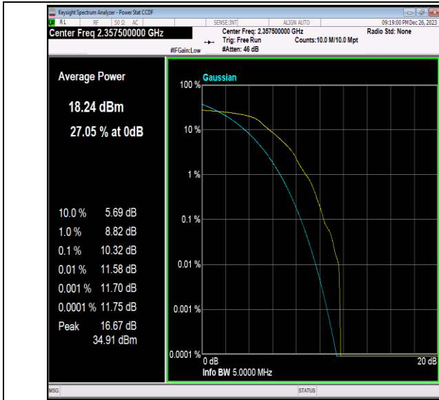
40(2350-2360)-5MHz-QPSK-39225-1RB#0-PASS
