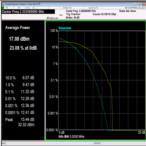
40(2350-2360)-5MHz-16QAM-39175-1RB#0-PASS
