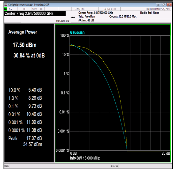
41(2535-2655)-15MHz-16QAM-41165-75RB#0-PASS
