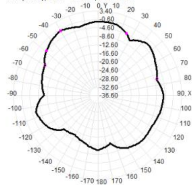
Total(H-XY), Max= -1.34dBi, CirD=13.90
