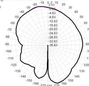
2480.0MHz Total(E2-YZ), Max= 2.82dBi
