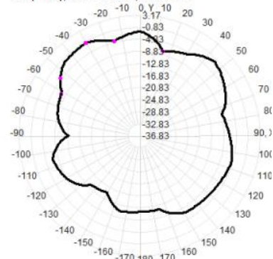
Total(H-XY), Max= -1.30dBi, CirD=13.97
