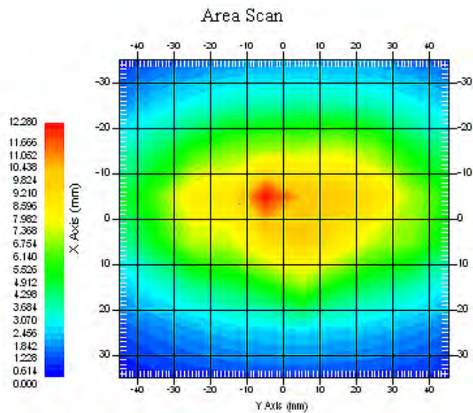
835 MHz System Validation with Head Tissue
