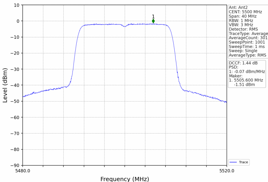
802.11ac(VHT20)_LCH_5500MHz_MIMO_NTNV
