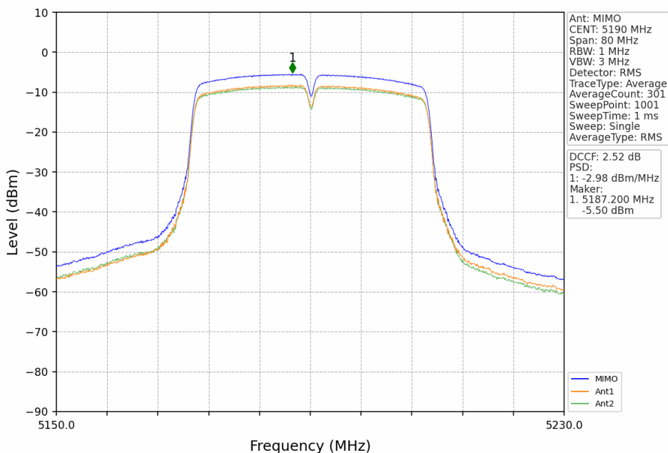
802.11ac(VHT40)_LCH_5190MHz_MIMO_NTNV
