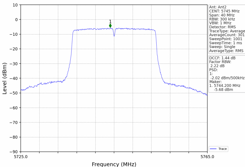
802.11n(HT20)_LCH_5745MHz_MIMO_NTNV
