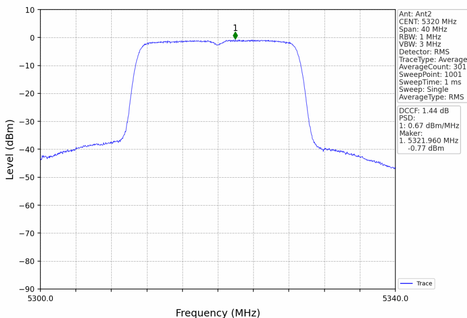
802.11ac(VHT20)_HCH_5320MHz_MIMO_NTNV
