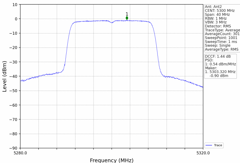
802.11ac(VHT20)_MCH_5300MHz_MIMO_NTNV
