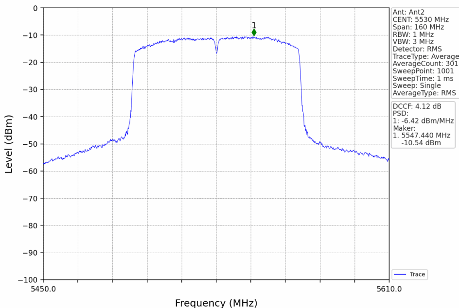
802.11ac(VHT80)_LCH_5530MHz_MIMO_NTNV
