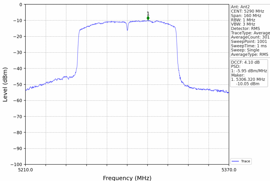
802.11ac(VHT80)_MCH_5290MHz_MIMO_NTNV
