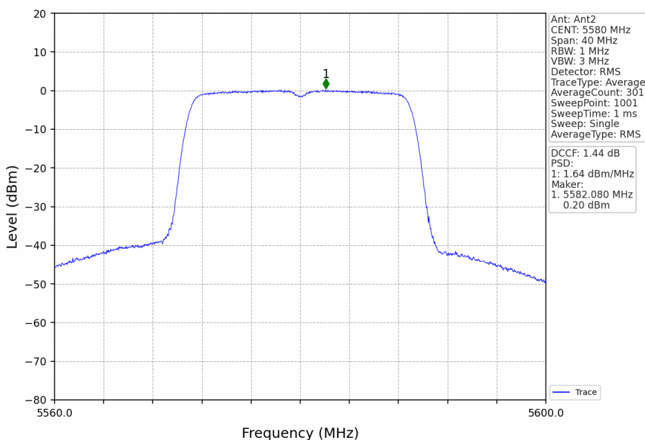
802.11ac(VHT20)_MCH_5580MHz_MIMO_NTNV
