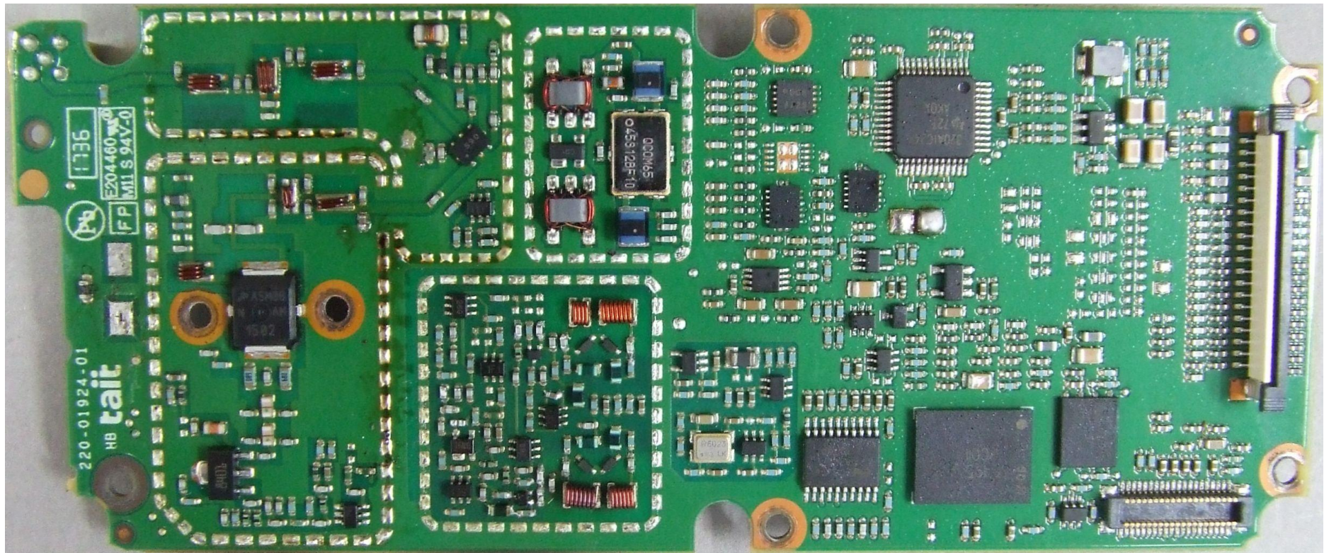
Photograph 03: Rx-Tx PCB - top (without shields)
