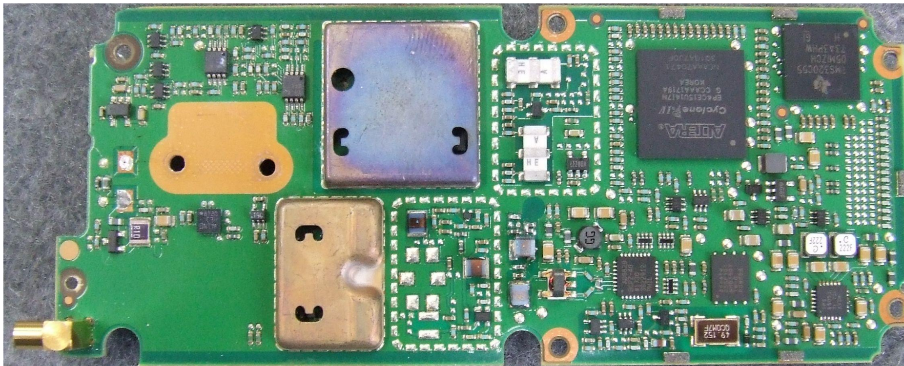
Photograph 04: Rx-Tx PCB - bottom (with shields)
