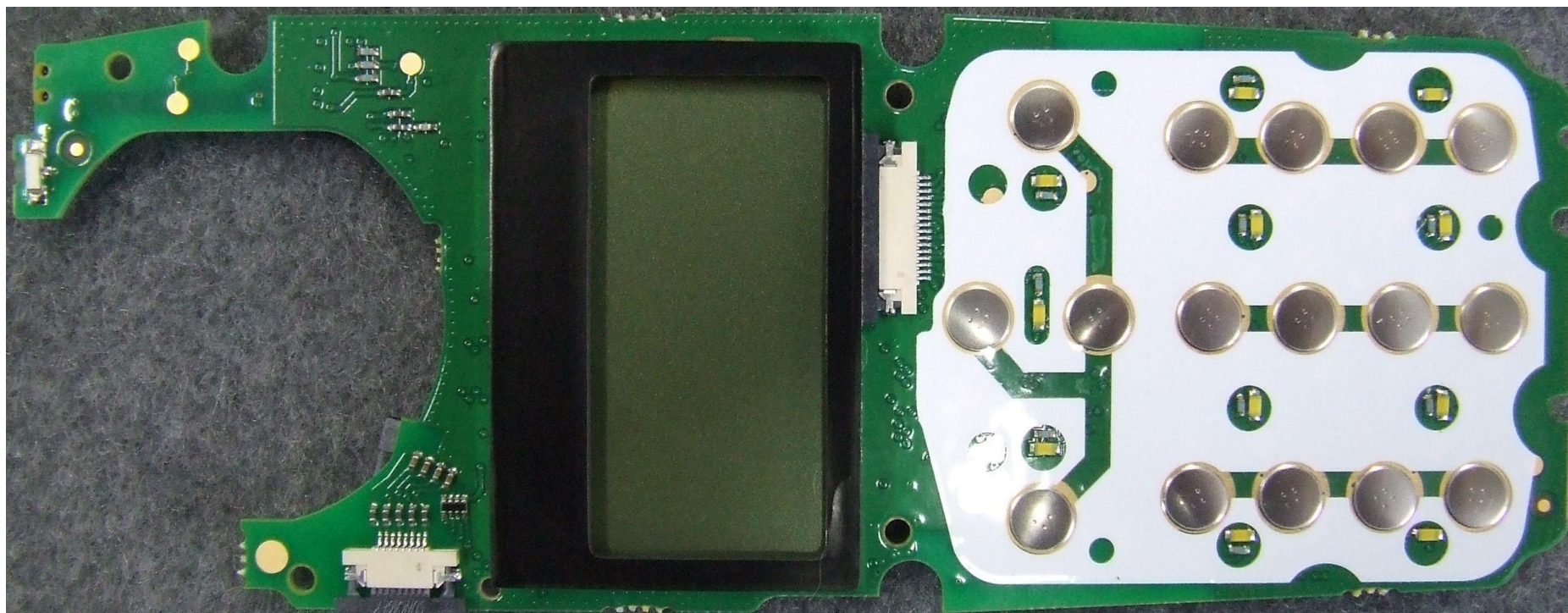
Photograph 07: Control PCB - bottom
