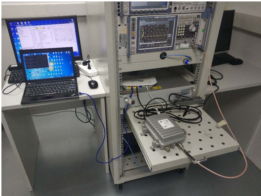
Conducted Test-Lora
