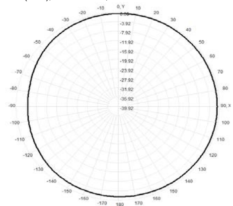
Total(H-XY), Max= -0.40dBi, CirD=4.21
