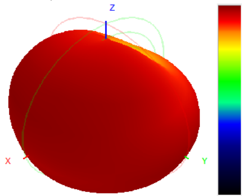
860.0MHz H+V, Eff: 49.9%
