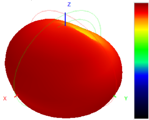
880.0MHz H+V, Eff: 59.9%
