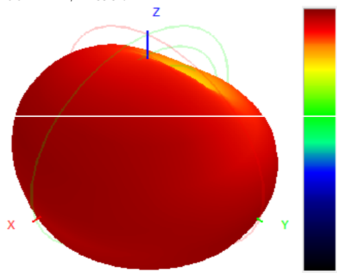
870.0MHz H+V, Eff: 58.5%
