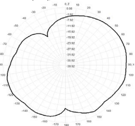
890.0MHz Total(E1-XZ), Max= -0.01dBi
