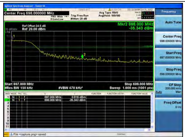
Band71 / 15MHz / High CH / QPSK / FULL RB
