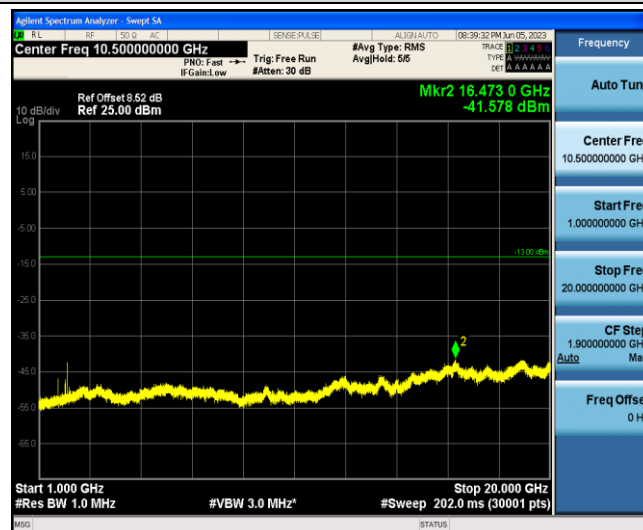
Band2-15MHz-QPSK-19125-1-0-Low-1000-20000--41.58-PASS
