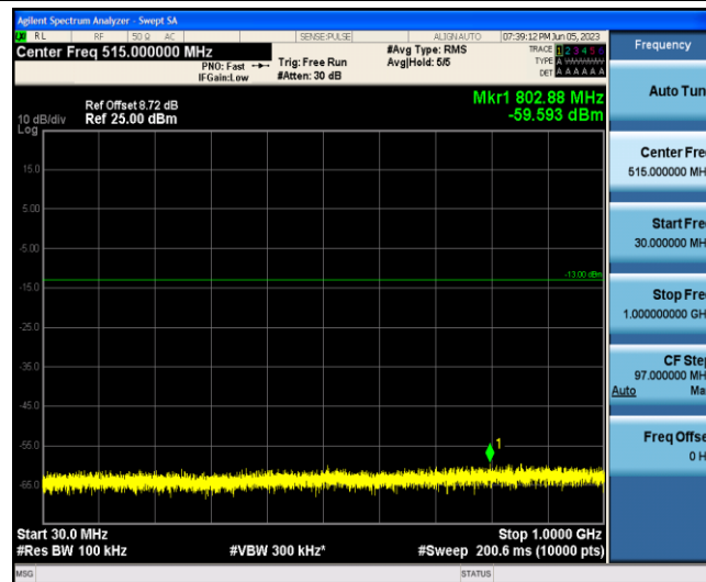
Band2-3MHz-QPSK-18615-1-0-Low-30-1000--59.59-PASS
