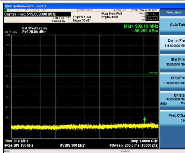
Band2-10MHz-QPSK-18900-1-0-Low-30-1000--59.29-PASS
