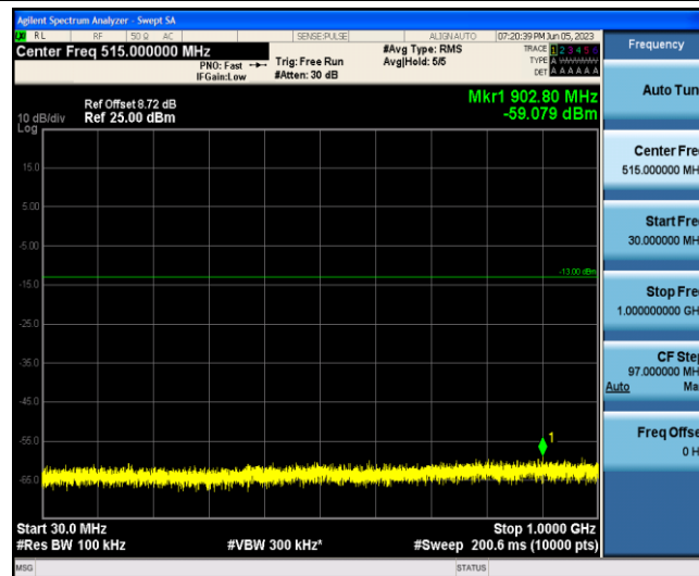
Band2-1.4MHz-16QAM-18607-1-0-Low-30-1000--59.08-PASS
