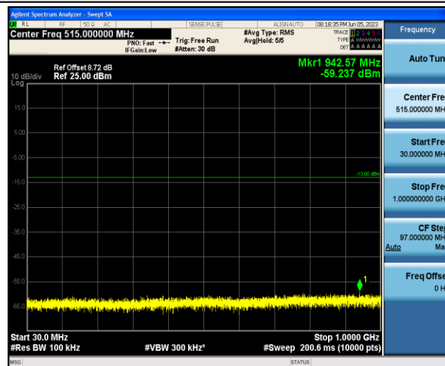
Band2-10MHz-16QAM-18900-1-0-Low-30-1000--59.24-PASS
