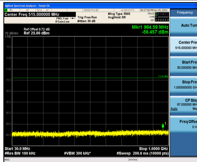
Band2-15MHz-QPSK-18675-1-0-Low-30-1000--59.46-PASS
