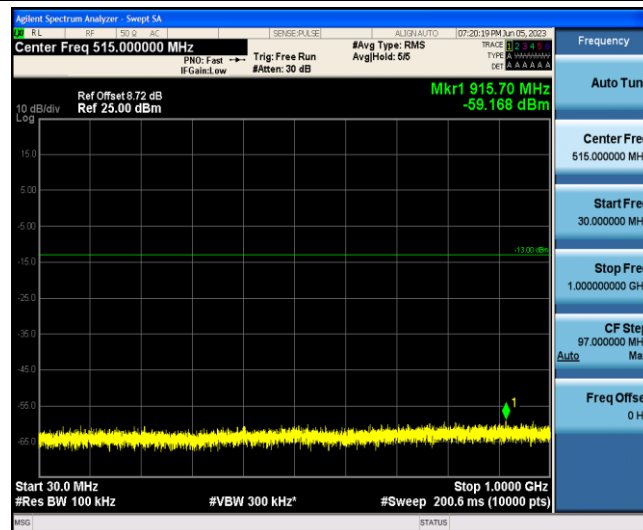
Band2-1.4MHz-QPSK-18607-1-0-Low-30-1000--59.17-PASS
