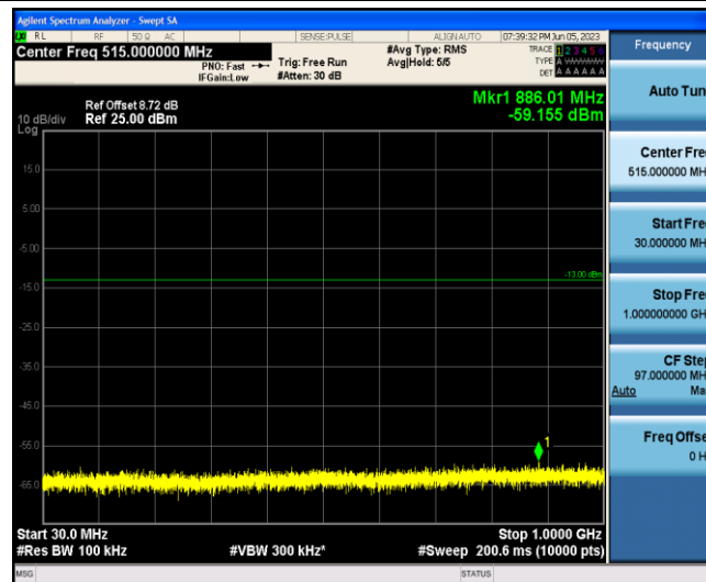
Band2-3MHz-16QAM-18615-1-0-Low-30-1000--59.16-PASS
