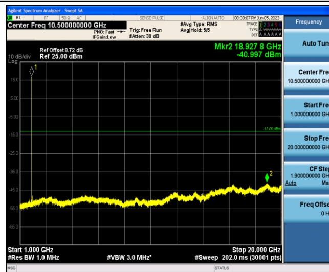
Band2-15MHz-QPSK-18675-1-0-Low-1000-20000--41-PASS
