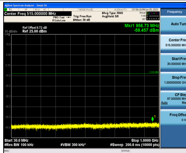
Band2-5MHz-16QAM-18625-1-0-Low-30-1000--59.46-PASS
