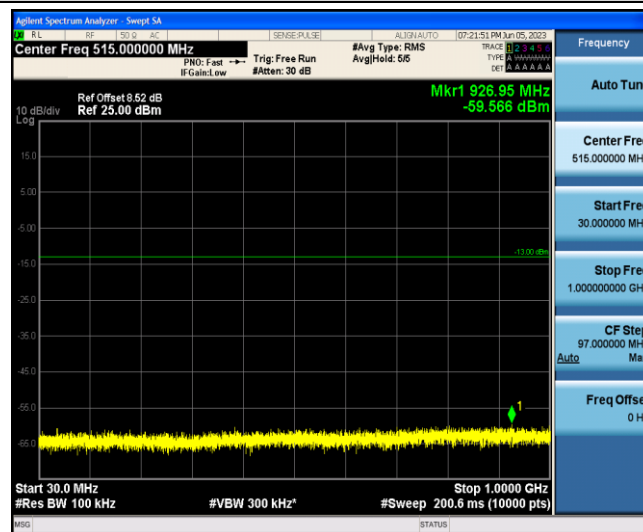
Band2-1.4MHz-QPSK-19193-1-0-Low-30-1000--59.57-PASS
