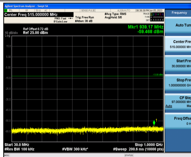
Band2-15MHz-QPSK-18900-1-0-Low-30-1000--59.47-PASS
