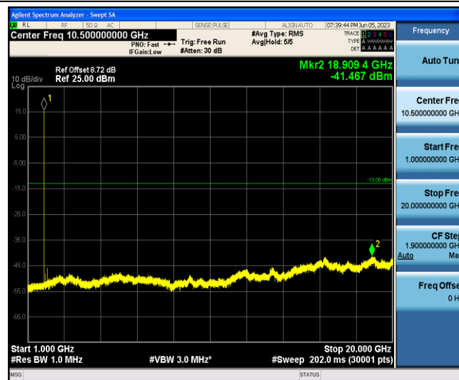
Band2-3MHz-16QAM-18615-1-0-Low-1000-20000--41.47-PASS
