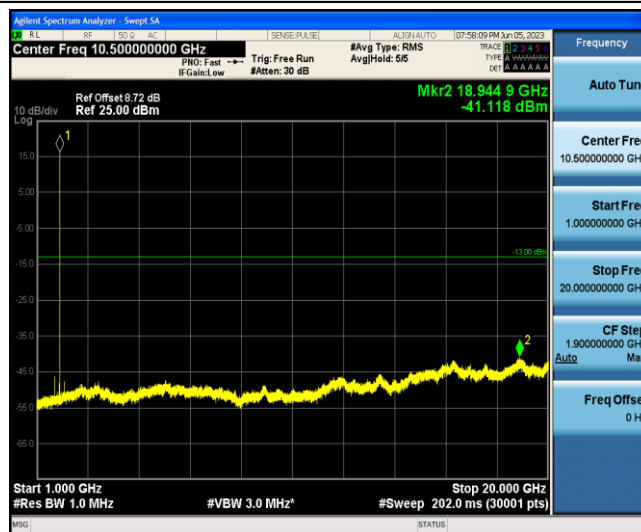
Band2-5MHz-QPSK-18625-1-0-Low-1000-20000--41.12-PASS
