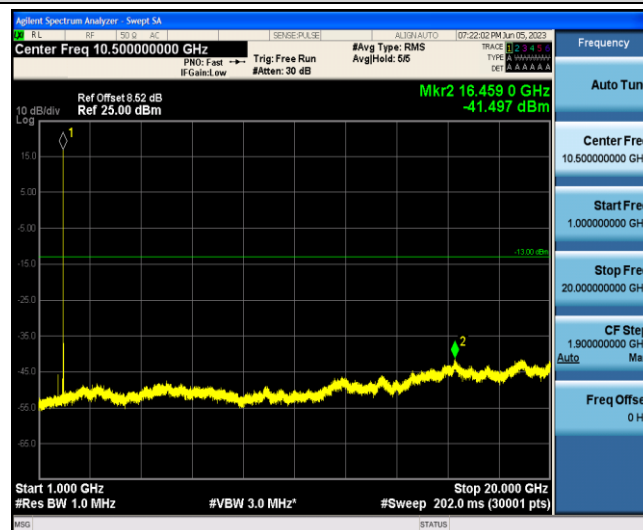
Band2-1.4MHz-QPSK-19193-1-0-Low-1000-20000--41.5-PASS
