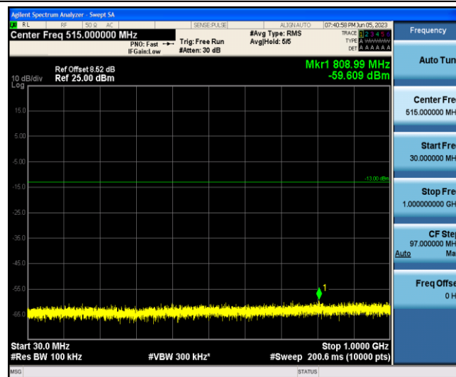
Band2-3MHz-16QAM-19185-1-0-Low-30-1000--59.61-PASS
