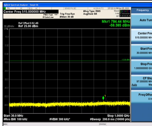
Band2-1.4MHz-16QAM-19193-1-0-Low-30-1000--59.39-PASS
