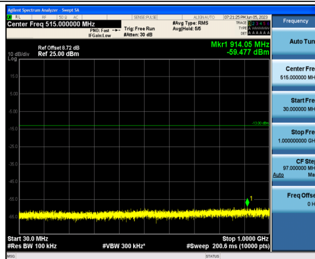
Band2-1.4MHz-16QAM-18900-1-0-Low-30-1000--59.48-PASS
