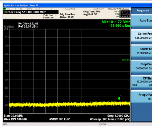
Band2-15MHz-QPSK-19125-1-0-Low-30-1000--59.66-PASS
