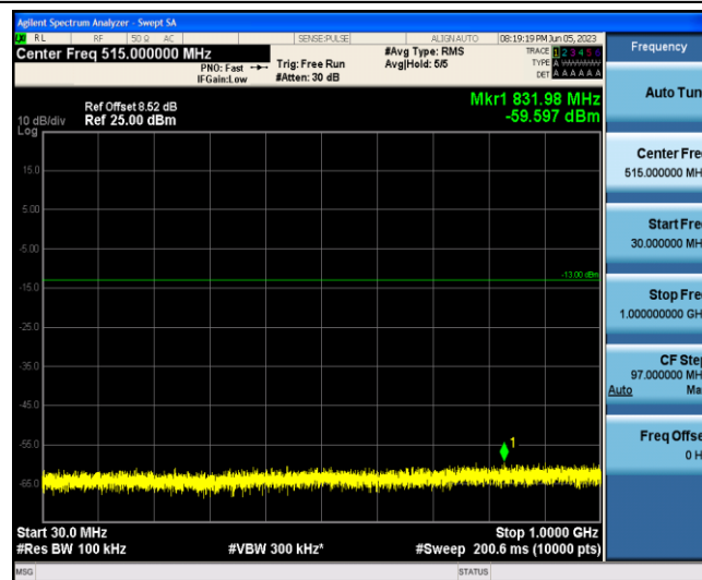
Band2-10MHz-16QAM-19150-1-0-Low-30-1000--59.6-PASS
