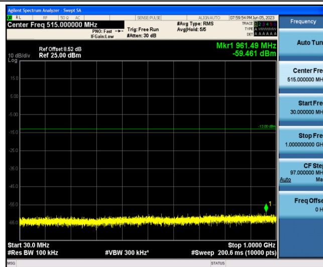
Band2-5MHz-16QAM-19175-1-0-Low-30-1000--59.46-PASS
