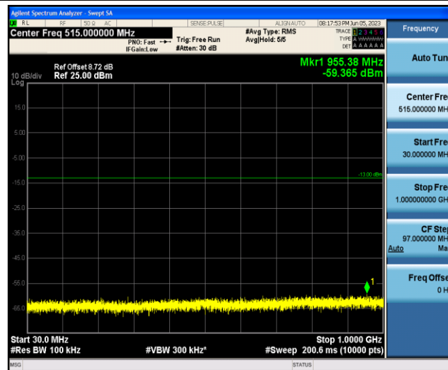
Band2-10MHz-16QAM-18650-1-0-Low-30-1000--59.37-PASS
