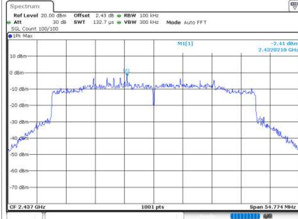
PSD NVNT ax40 2437MHz Ant2
