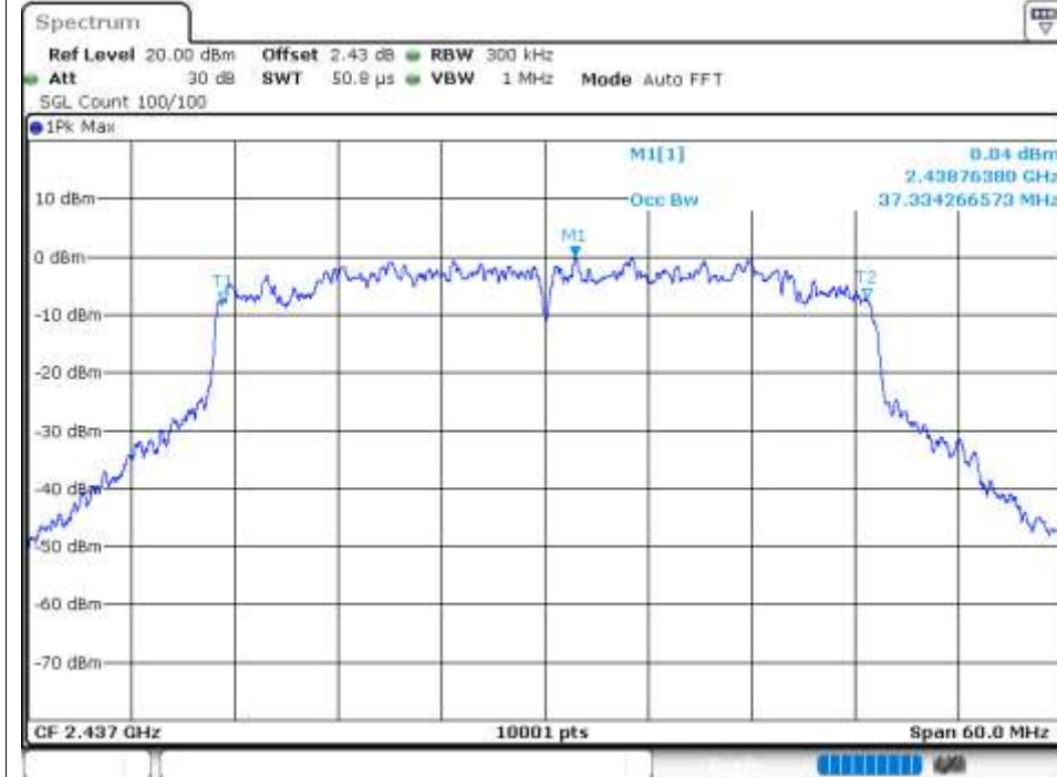
OBW NVNT ax40 2437MHz Ant2
