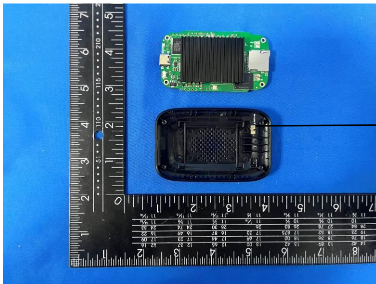
BT PIFA Antenna
