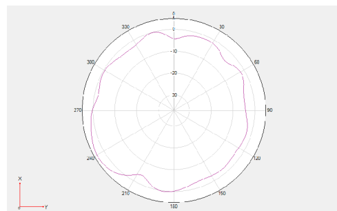
Theta =90 freq=5500MHz
