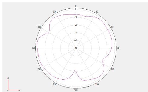
Phi =0 freq=5500MHz
