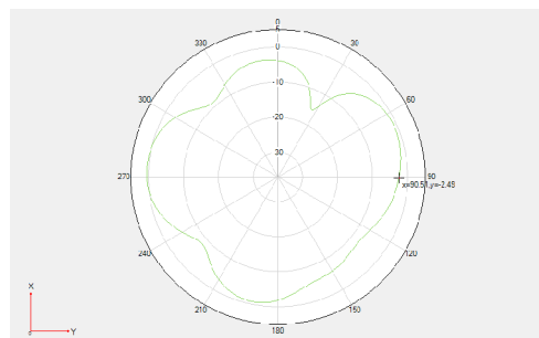
Theta =90 freq=2500MHz
