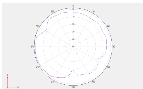
Phi =0 freq=5850MHz
