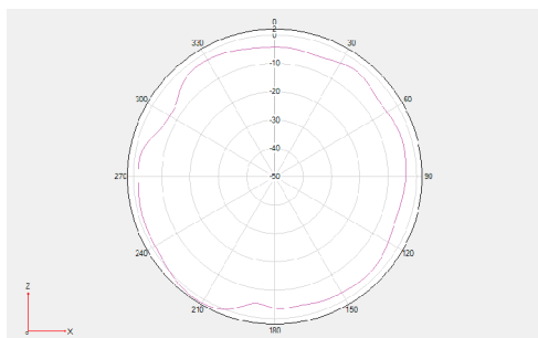
Phi =0 freq=2500MHz
