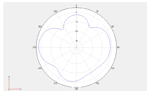
Theta =90 freq=2450MHz
