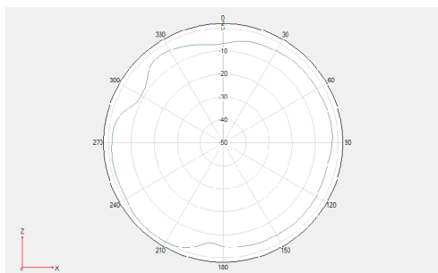
Phi =0 freq=2450MHz
