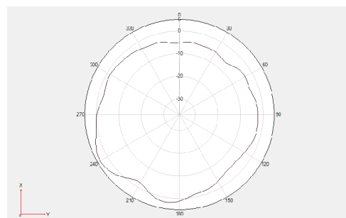
Theta =90 freq=5850MHz
