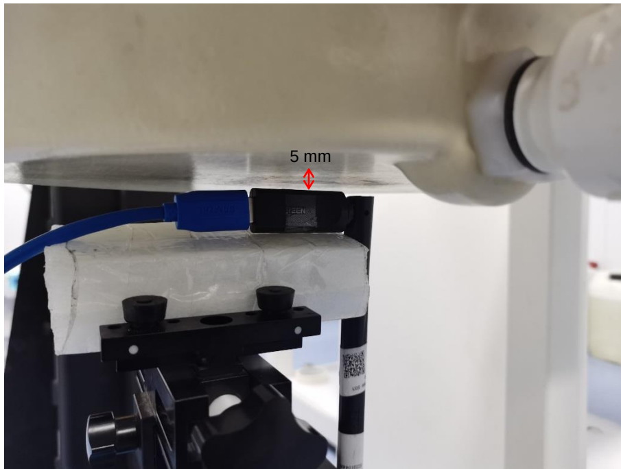
Vertical-Back-fold (5mm)
