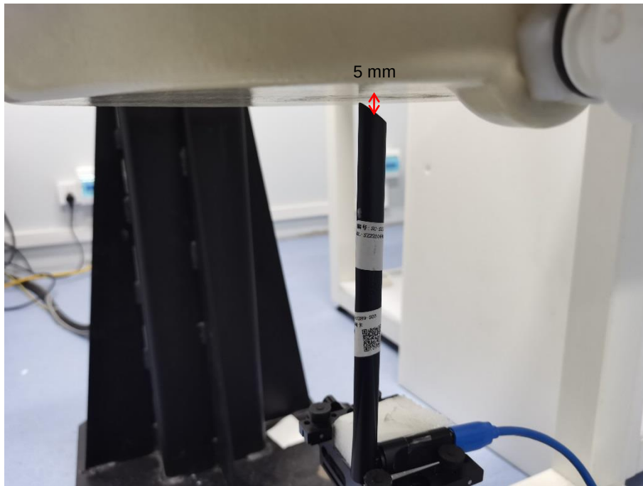
Vertical-Front-fold (5mm)
