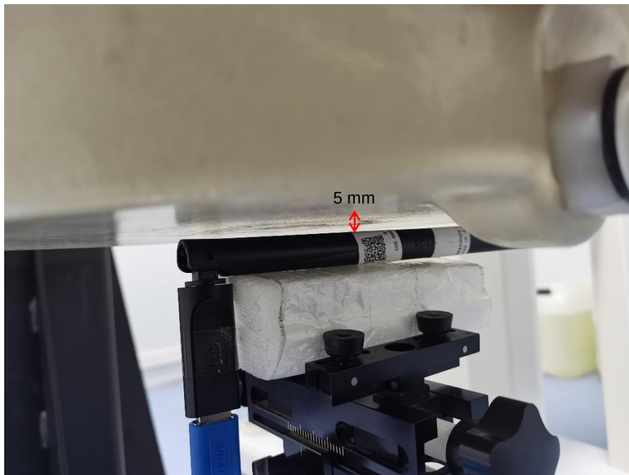
Tip-fold (5mm)
