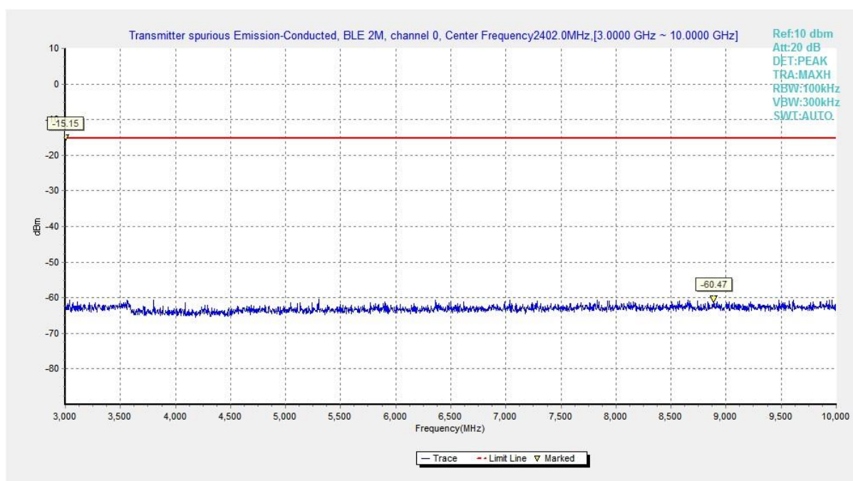
Fig.26 Conducted Spurious Emission (Ch0, 3 GHz-10 GHz), LE 2M
