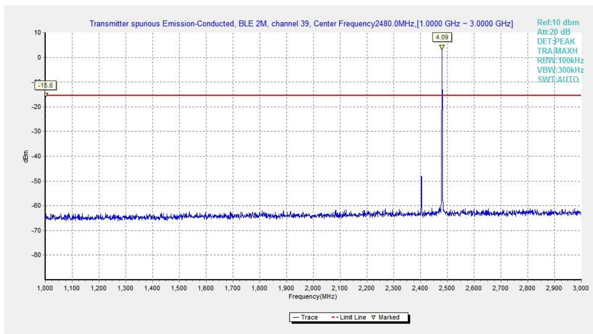
Fig.29 Conducted Spurious Emission (Ch39, 1 GHz-3 GHz), LE 2M
