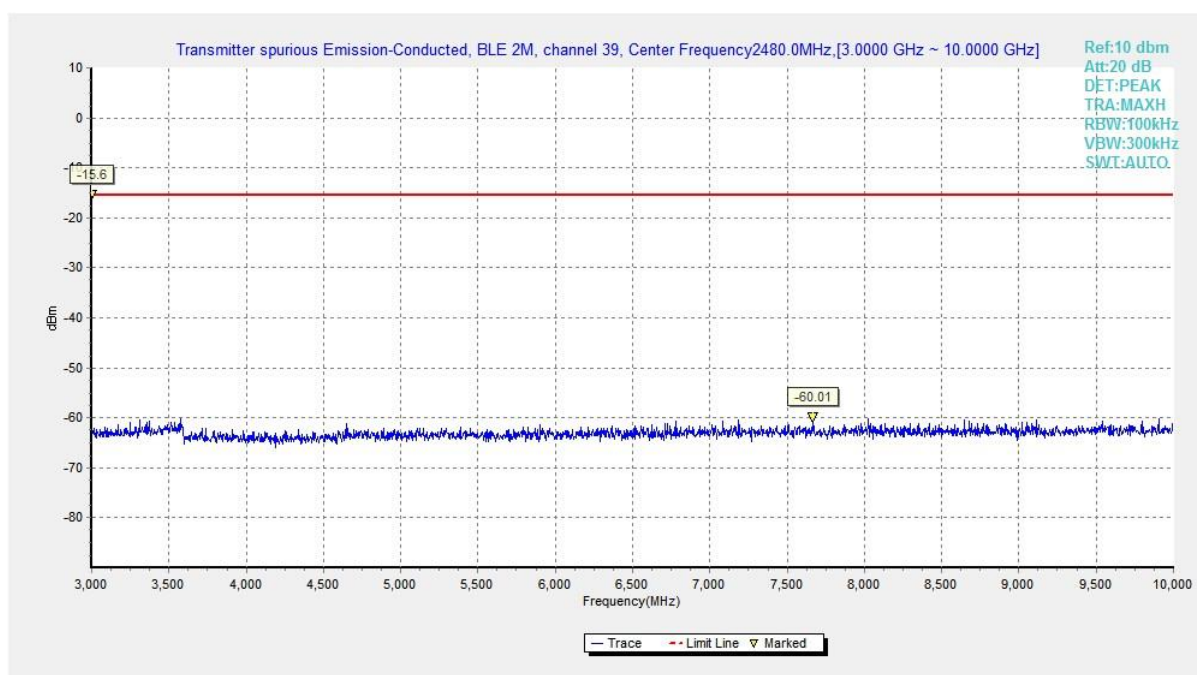
Fig.30 Conducted Spurious Emission (Ch39, 3 GHz-10 GHz), LE 2M
