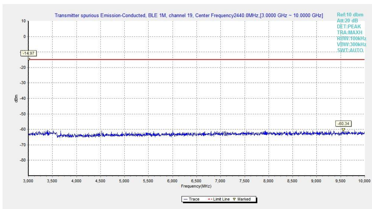
Fig.20 Conducted Spurious Emission (Ch19, 3 GHz-10 GHz), LE 1M
