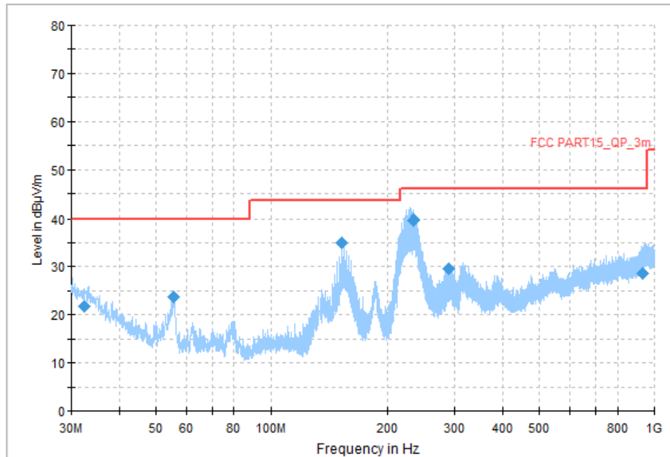
Fig.43 Radiated Spurious Emission (Ch19, 30 MHz - 1 GHz), 2M
