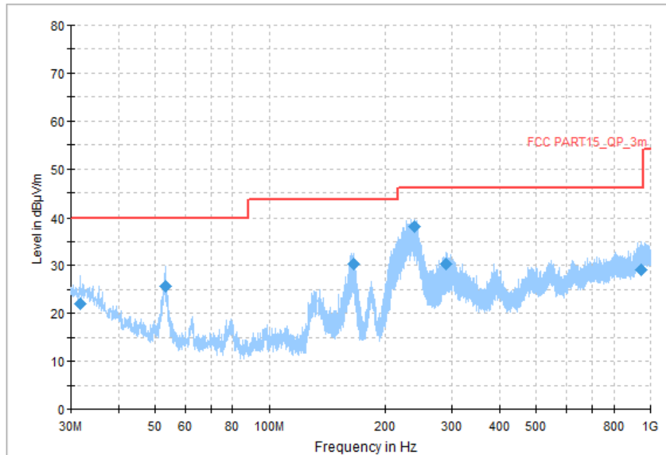
Fig.35 Radiated Spurious Emission (Ch19, 30 MHz - 1 GHz), 1M
