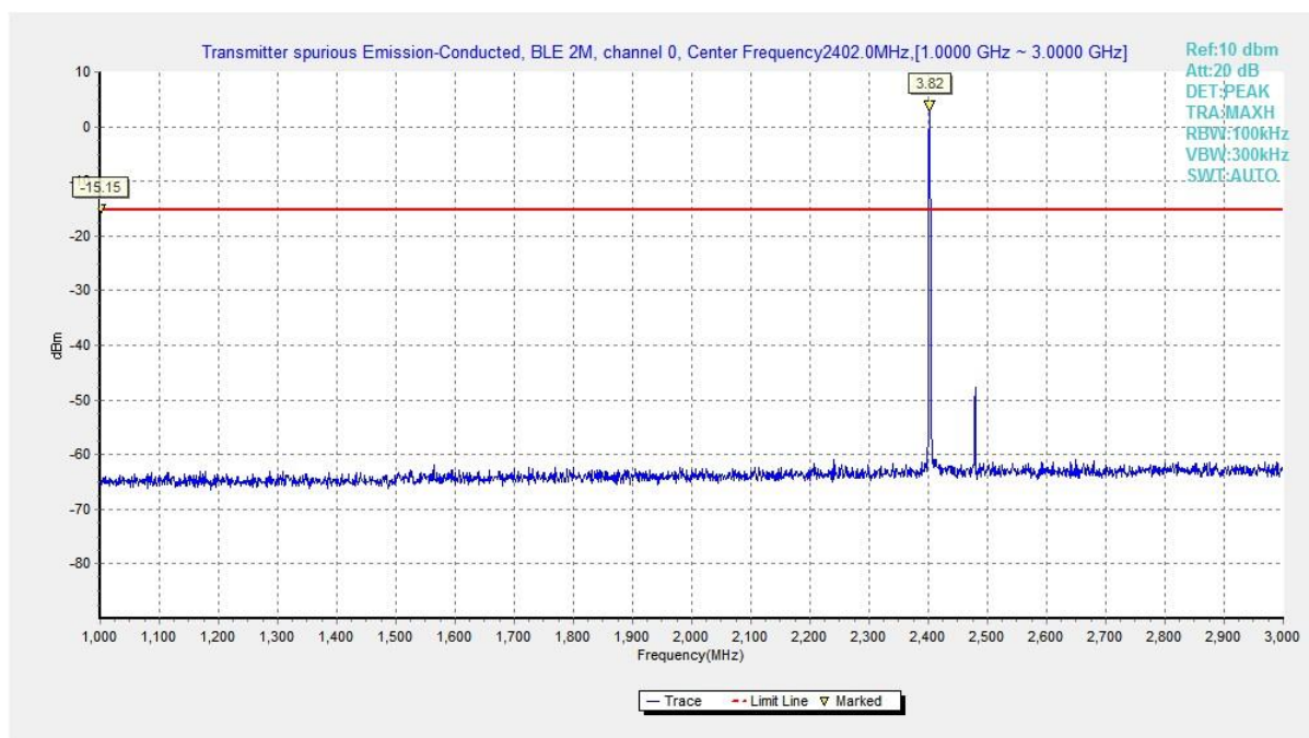
Fig.25 Conducted Spurious Emission (Ch0, 1 GHz-3 GHz), LE 2M
