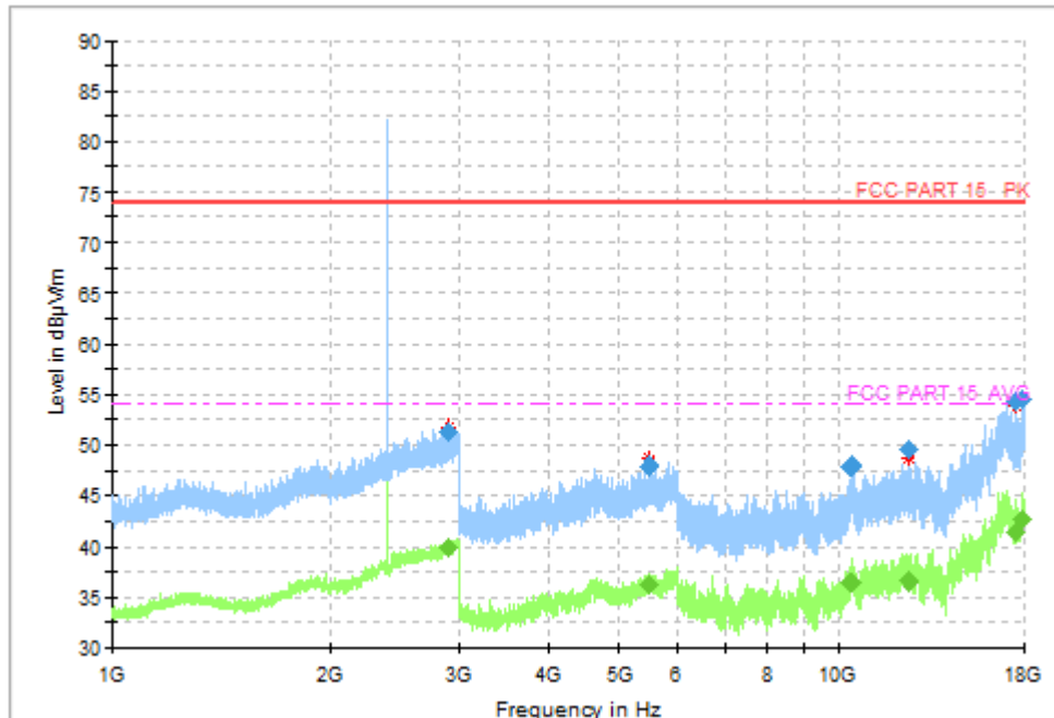
Fig.33 Radiated Spurious Emission (Ch0, 1 GHz - 18 GHz), 1M
