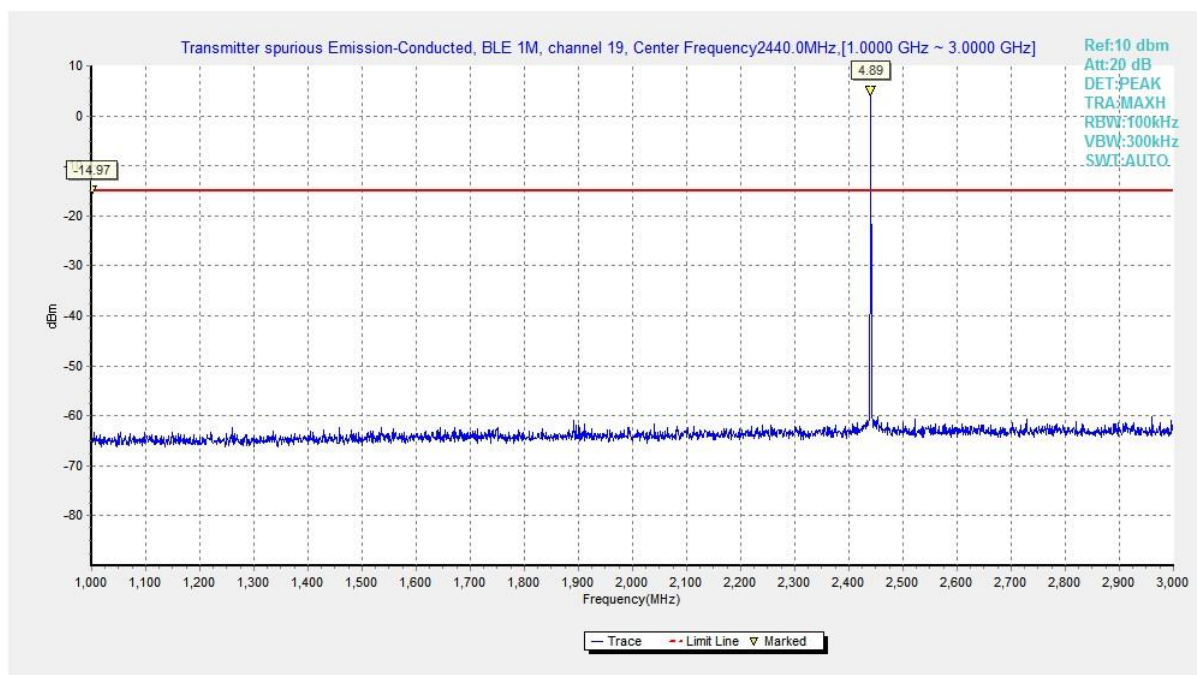
Fig.19 Conducted Spurious Emission (Ch19, 1 GHz-3 GHz), LE 1M
