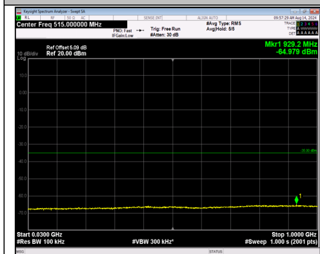
7-7-10MHz-20MHz-QPSK-QPSK-21206-21350-1RB#0-1 RB#99-30~1000MHz-PASS
