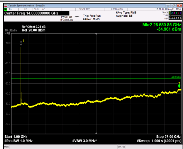
7-7-10MHz-20MHz-64QAM-64QAM-20805-20949-50RB#0- 100RB#0-1000~27000MHz-PASS
