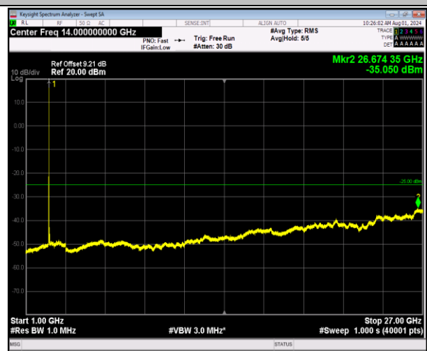
7-7-10MHz-20MHz-64QAM-64QAM-20805-20949-1RB#49- 0RB#0-1000~27000MHz-PASS
