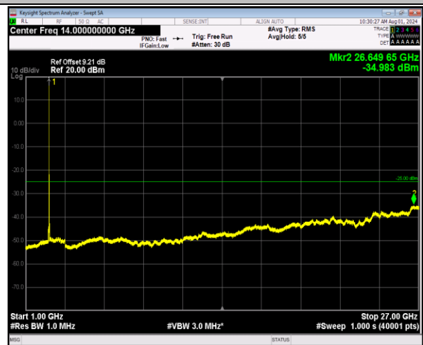
7-7-10MHz-20MHz-64QAM-64QAM-21206-21350-1RB#0-0 RB#0-1000~27000MHz-PASS
