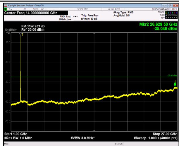
7-7-10MHz-20MHz-64QAM-64QAM-20805-20949-1RB#0-0 RB#0-1000~27000MHz-PASS
