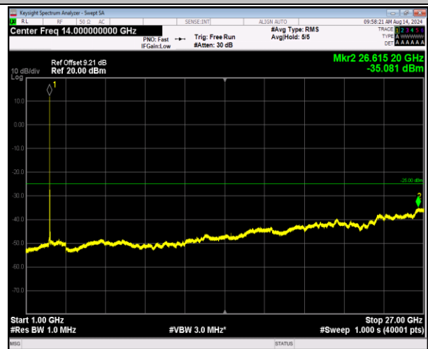
7-7-10MHz-20MHz-16QAM-16QAM-21206-21350-1RB#0-1-1000~27000MHz-PASS
