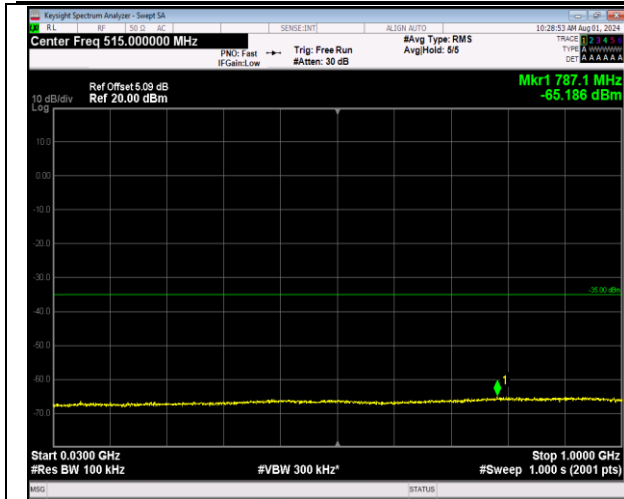
7-7-10MHz-20MHz-64QAM-64QAM-21006-21150-1RB#0 -1RB#99-30~1000MHz-PASS
