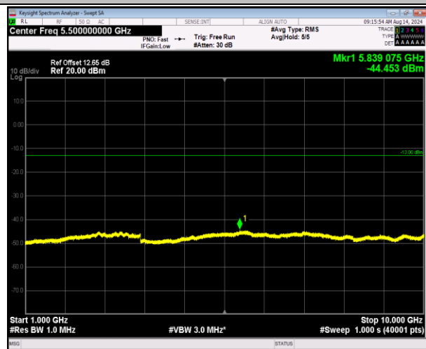
5-5-10MHz-10MHz-16QAM-16QAM-20501-20600-1RB#0-1RB#49-1000~10000MHz-PASS
