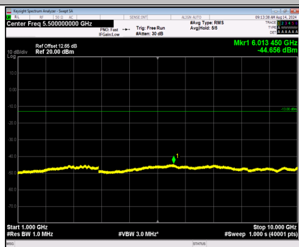
5-5-10MHz-10MHz-16QAM-16QAM-20501-20600-1RB#0-0RB#0-1000~10000MHz-PASS
