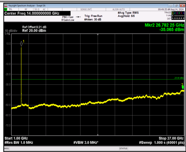
7-7-10MHz-20MHz-16QAM-16QAM-20805-20949-50RB#0- 100RB#0-1000~27000MHz-PASS
