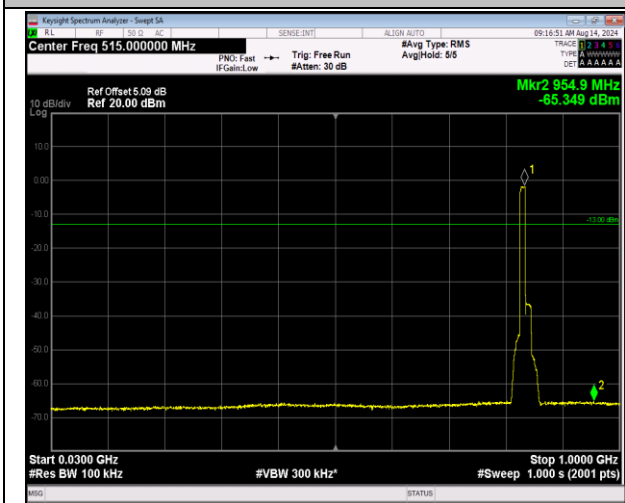
5-5-10MHz-10MHz-16QAM-16QAM-20501-20600-50RB#- 0-50RB#0-30~1000MHz-PASS
