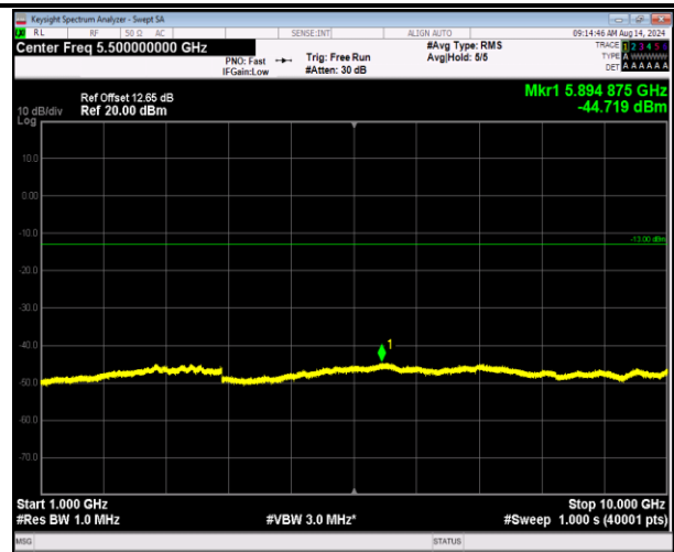
5-5-10MHz-10MHz-16QAM-16QAM-20501-20600-1RB#49- 0RB#0-1000~10000MHz-PASS
