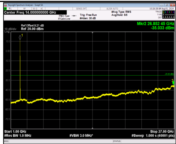
7-7-10MHz-20MHz-64QAM-64QAM-20805-20949-1RB#0-1 RB#99-1000~27000MHz-PASS
