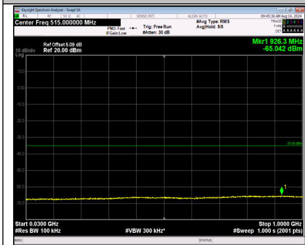
7-7-10MHz-20MHz-16QAM-16QAM-20805-20949-1RB#0-0-30~1000MHz-PASS
