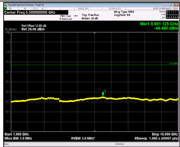
5-5-10MHz-10MHz-64QAM-64QAM-20501-20600-50RB#0- 50RB#0-1000~10000MHz-PASS
