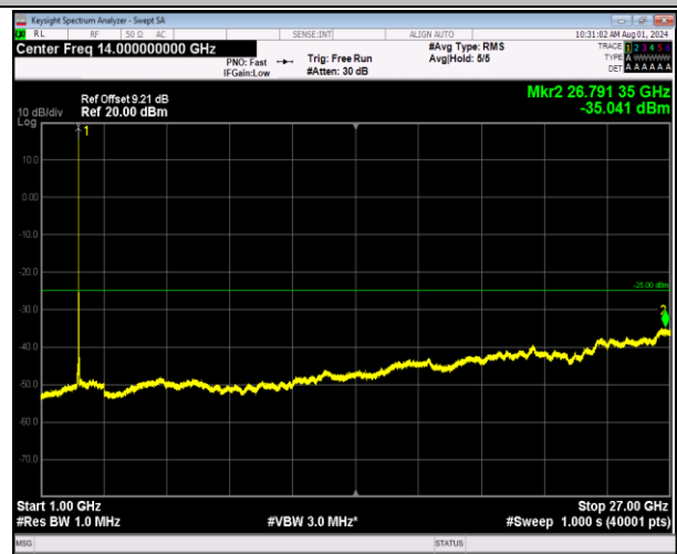
7-7-10MHz-20MHz-64QAM-64QAM-21206-21350-1RB#49- 0RB#0-1000~27000MHz-PASS
