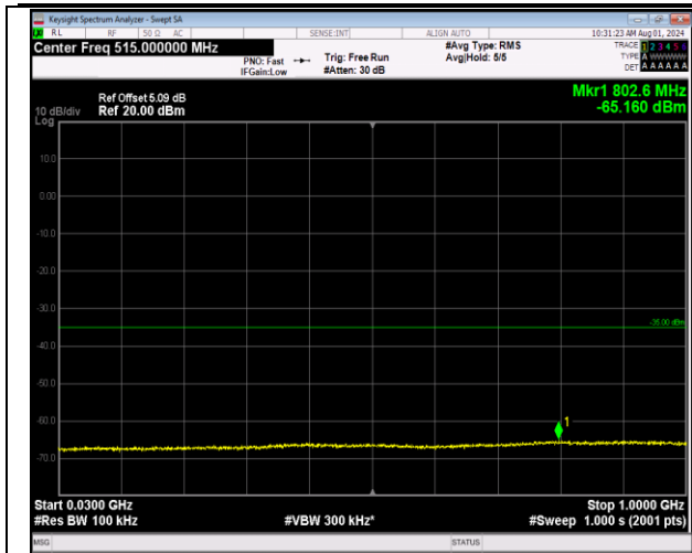
7-7-10MHz-20MHz-64QAM-64QAM-21206-21350-1RB#0 -1RB#99-30~1000MHz-PASS
