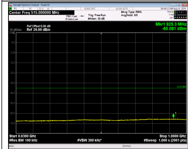
7-7-10MHz-20MHz-QPSK-QPSK-20805-20949-1RB#49-4 ORB#0-30~1000MHz-PASS
