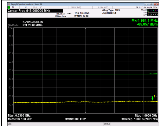
7-7-10MHz-20MHz-QPSK-QPSK-21006-21150-1RB#49-0 ORB#0-30~1000MHz-PASS
