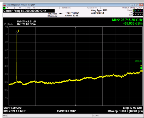
7-7-10MHz-20MHz-16QAM-16QAM-21206-21350-50RB#0- 100RB#0-1000~27000MHz-PASS
