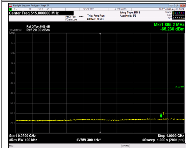
7-7-10MHz-20MHz-64QAM-64QAM-21006-21150-1RB#0 -0RB#0-30~1000MHz-PASS
