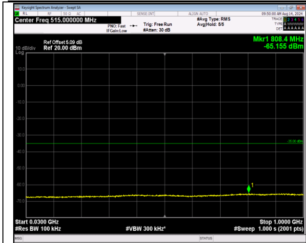
7-7-10MHz-20MHz-QPSK-QPSK-21006-21150-1RB#0-0 RB#0-30~1000MHz-PASS
