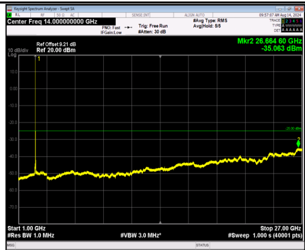
7-7-10MHz-20MHz-16QAM-16QAM-21206-21350-1RB#49- 0RB#0-1000~27000MHz-PASS
