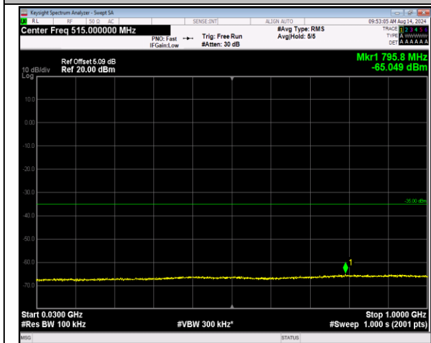
7-7-10MHz-20MHz-16QAM-16QAM-21006-21150-1RB#0-1-99~1000MHz-PASS
