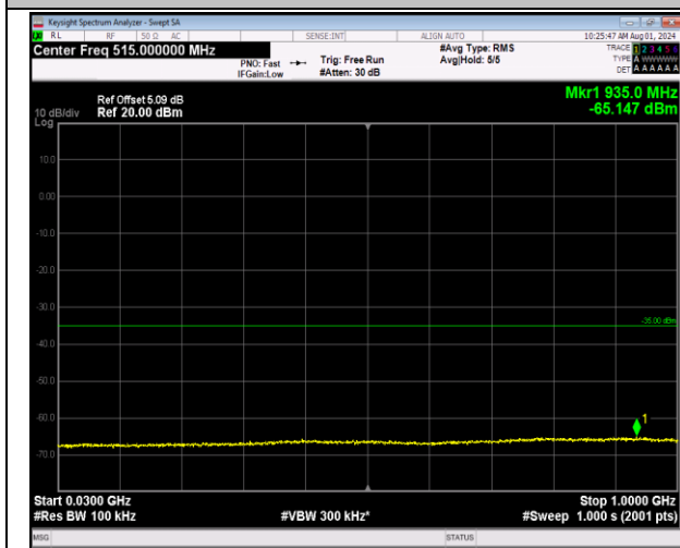
7-7-10MHz-20MHz-64QAM-64QAM-20805-20949-1RB#4 9-0RB#0-30~1000MHz-PASS
