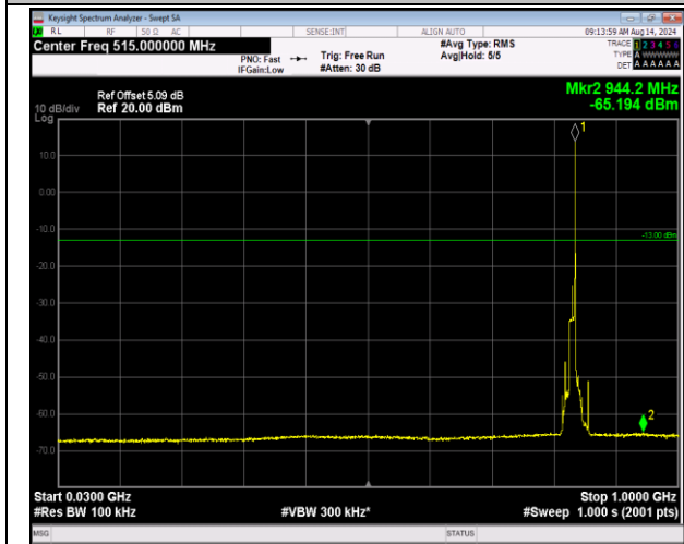
5-5-10MHz-10MHz-QPSK-QPSK-20501-20600-1RB#49-49 ORB#0-30~1000MHz-PASS
