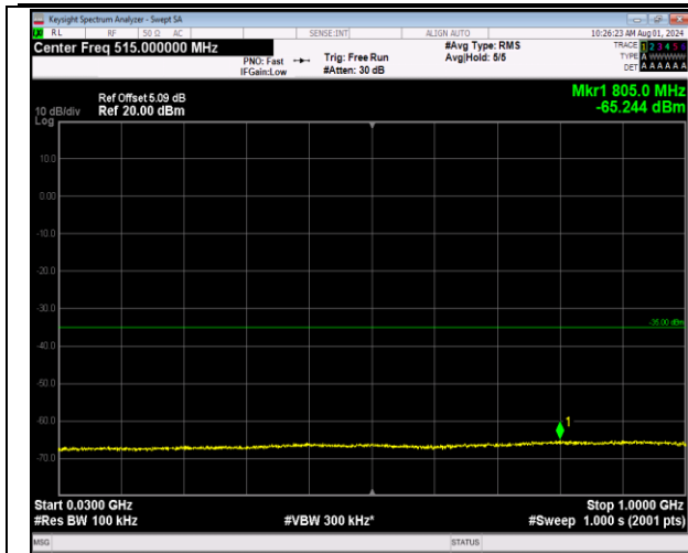
7-7-10MHz-20MHz-64QAM-64QAM-20805-20949-1RB#0 -1RB#99-30~1000MHz-PASS
