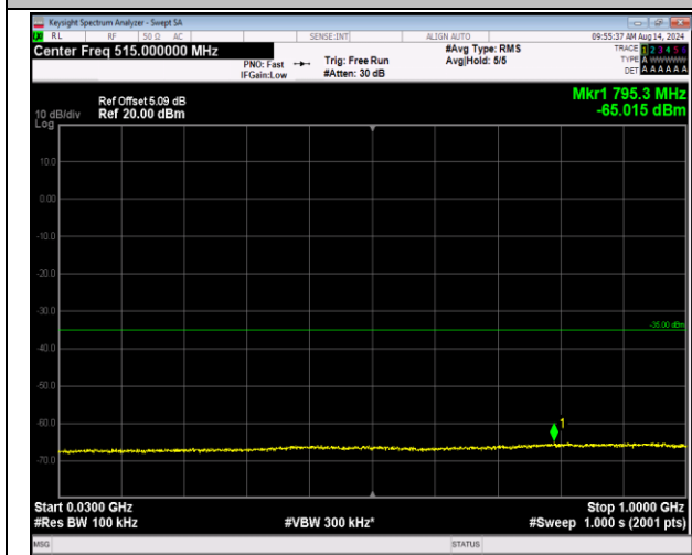
7-7-10MHz-20MHz-16QAM-16QAM-21206-21350-1RB#0-0-30~1000MHz-PASS
