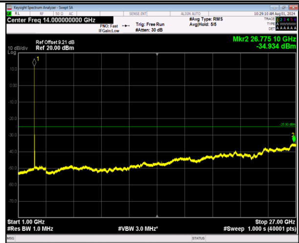
7-7-10MHz-20MHz-64QAM-64QAM-21006-21150-1RB#0-1 RB#99-1000~27000MHz-PASS
