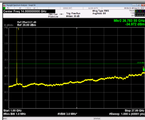
7-7-10MHz-20MHz-QPSK-QPSK-21206-21350-1RB#49-0RB B#0-1000~27000MHz-PASS
