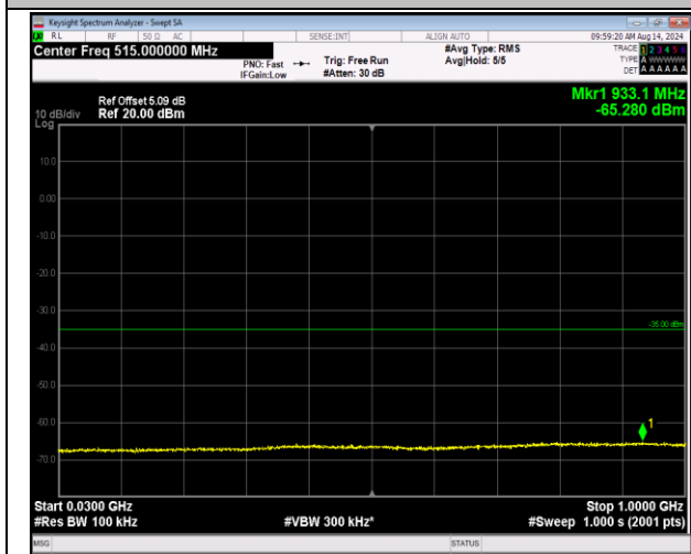
7-7-10MHz-20MHz-16QAM-16QAM-21206-21350-50RB#- 0-100RB#0-30~1000MHz-PASS
