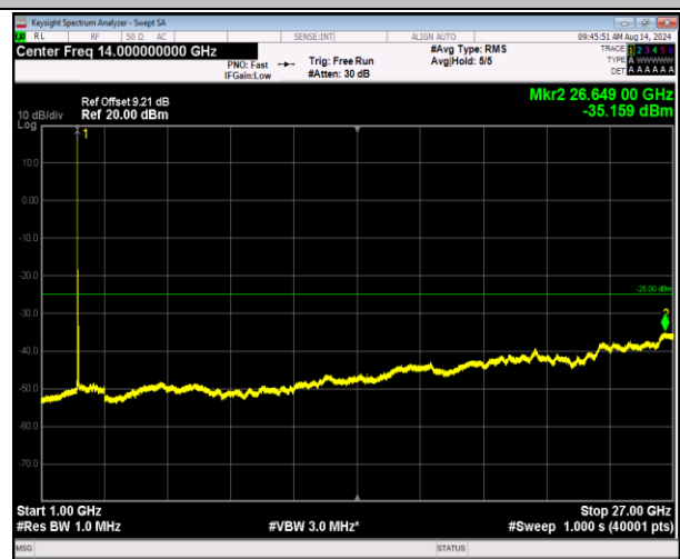
7-7-10MHz-20MHz-16QAM-16QAM-20805-20949-1RB#0-0-1000~27000MHz-PASS
