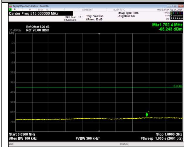
7-7-10MHz-20MHz-16QAM-16QAM-21006-21150-1RB#0-0-30~1000MHz-PASS
