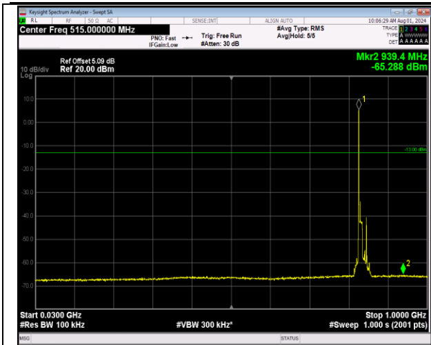
5-5-10MHz-10MHz-64QAM-64QAM-20501-20600-1RB#0 -1RB#49-30~1000MHz-PASS
