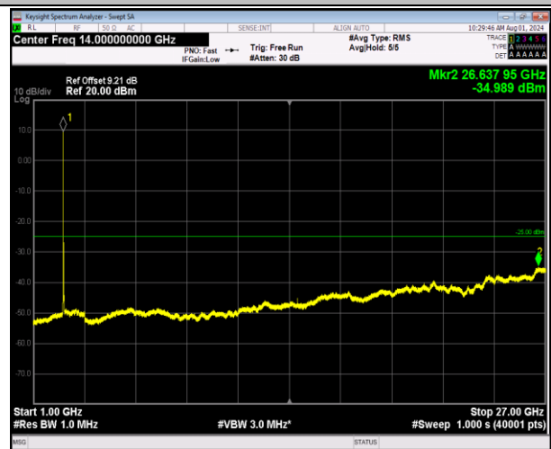
7-7-10MHz-20MHz-64QAM-64QAM-21006-21150-50RB#0- 100RB#0-1000~27000MHz-PASS
