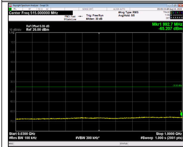
7-7-10MHz-20MHz-16QAM-16QAM-20805-20949-50RB#- 0-100RB#0-30~1000MHz-PASS
