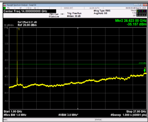
7-7-10MHz-20MHz-16QAM-16QAM-21206-21350-1RB#0-0-1000~27000MHz-PASS
