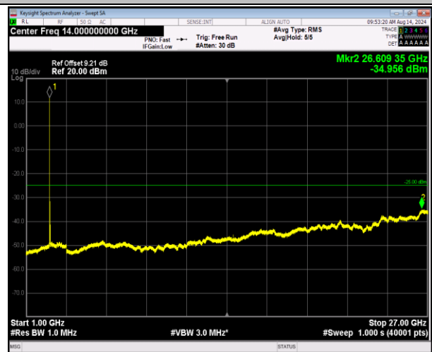
7-7-10MHz-20MHz-16QAM-16QAM-21006-21150-1RB#0-1-99~1000~27000MHz-PASS
