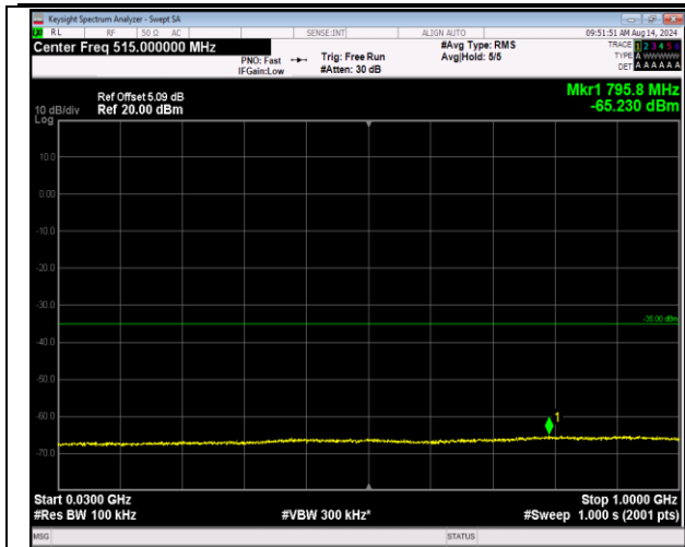
7-7-10MHz-20MHz-16QAM-16QAM-21006-21150-1RB#4 9-0RB#0-30~1000MHz-PASS
