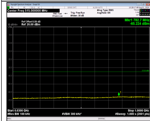
7-7-10MHz-20MHz-64QAM-64QAM-21006-21150-1RB#4 9-0RB#0-30~1000MHz-PASS
