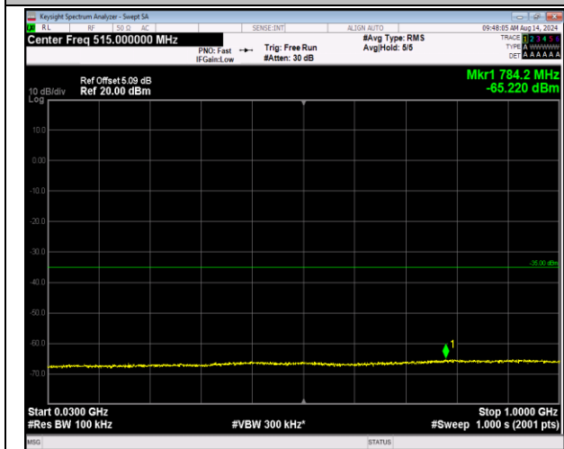
7-7-10MHz-20MHz-16QAM-16QAM-20805-20949-1RB#0-1-99~1000MHz-PASS
