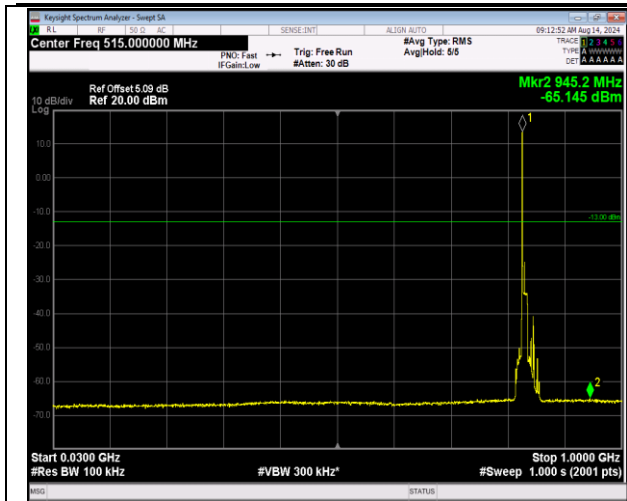
5-5-10MHz-10MHz-QPSK-QPSK-20501-20600-1RB#0-0 RB#0-30~1000MHz-PASS
