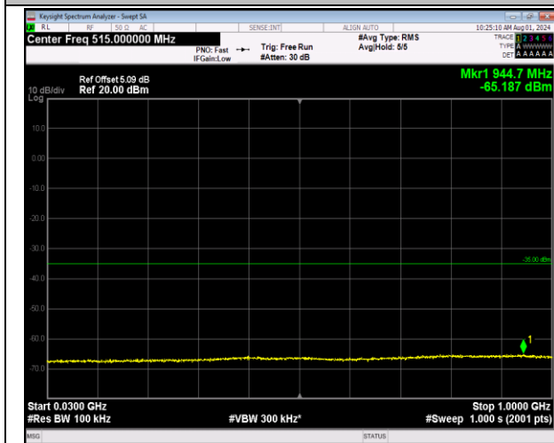
7-7-10MHz-20MHz-64QAM-64QAM-20805-20949-1RB#0- -0RB#0-30~1000MHz-PASS
