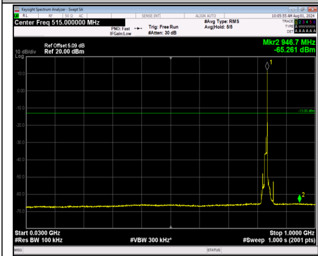
5-5-10MHz-10MHz-64QAM-64QAM-20501-20600-1RB#4 9-0RB#0-30~1000MHz-PASS
