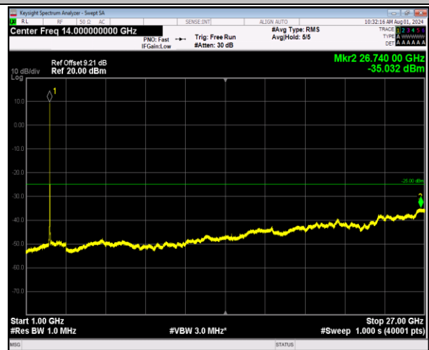
7-7-10MHz-20MHz-64QAM-64QAM-21206-21350-50RB#0- 100RB#0-1000~27000MHz-PASS
