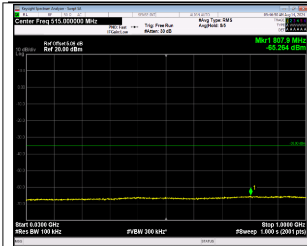
7-7-10MHz-20MHz-16QAM-16QAM-20805-20949-1RB#4 9-0RB#0-30~1000MHz-PASS
