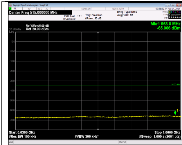
7-7-10MHz-20MHz-16QAM-16QAM-21206-21350-1RB#4 9-0RB#0-30~1000MHz-PASS
