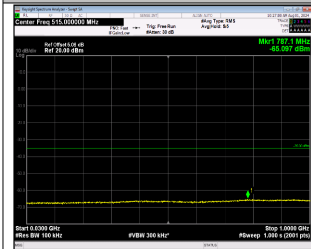
7-7-10MHz-20MHz-64QAM-64QAM-20805-20949-50RB# 0-100RB#0-30~1000MHz-PASS
