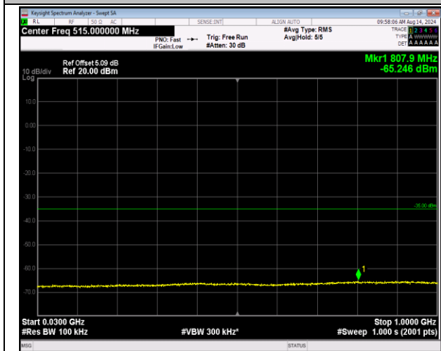
7-7-10MHz-20MHz-16QAM-16QAM-21206-21350-1RB#0-1-99~1000MHz-PASS
