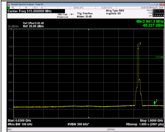
5-5-10MHz-10MHz-64QAM-64QAM-20501-20600-50RB# 0-50RB#0-30~1000MHz-PASS
