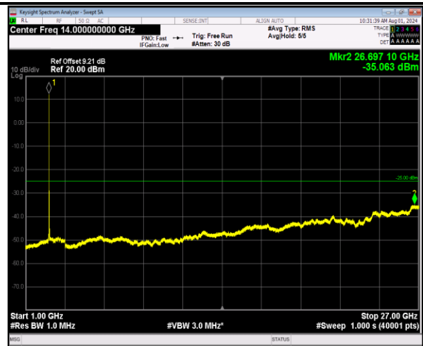
7-7-10MHz-20MHz-64QAM-64QAM-21206-21350-1RB#0-1 RB#99-1000~27000MHz-PASS
