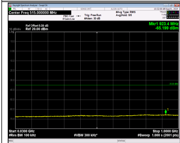
7-7-10MHz-20MHz-64QAM-64QAM-21206-21350-50RB# 0-100RB#0-30~1000MHz-PASS
