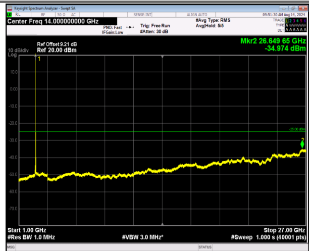
7-7-10MHz-20MHz-QPSK-QPSK-21006-21150-1RB#49-0R B#0-1000~27000MHz-PASS
