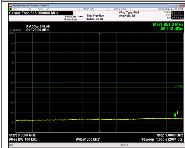
7-7-10MHz-20MHz-64QAM-64QAM-21206-21350-1RB#4 9-0RB#0-30~1000MHz-PASS
