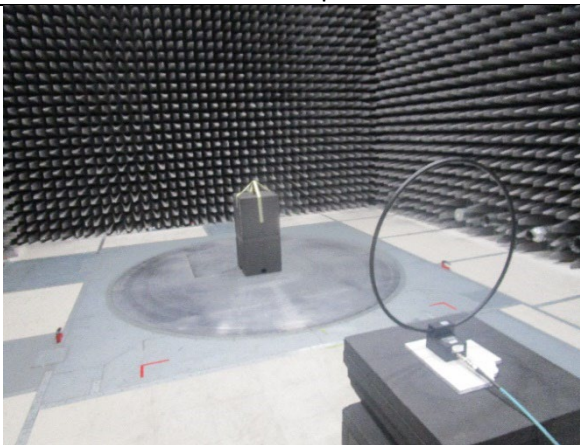
150 kHz – 30 MHz
