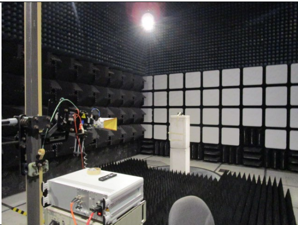
4-18 GHz
