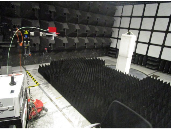
18-40 GHz
