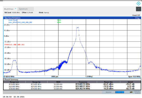
N5-15kHz-10MHz-DFT-QPSK-Low-Edge_1RB_Left--PASS
