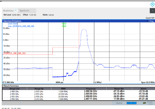
N41-30kHz-40MHz-DFT-QPSK-Low-Edge_1RB_Left---PASS
