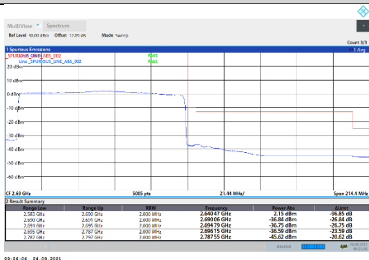
N41-30kHz-100MHz-DFT-QPSK-High-Outer_Full---PASS
