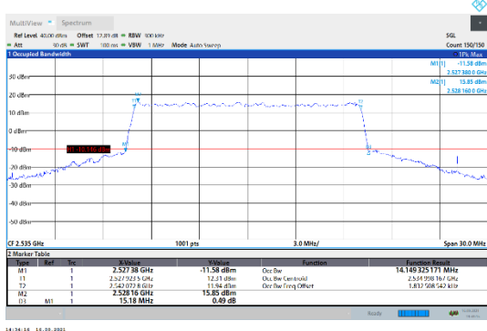
N7-15kHz-15MHz-CP-16QAM-Mid-Outer_Full---PASS
