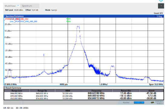
N5-15kHz-5MHz-DFT-QPSK-High-Edge_1RB_Right---PASS
