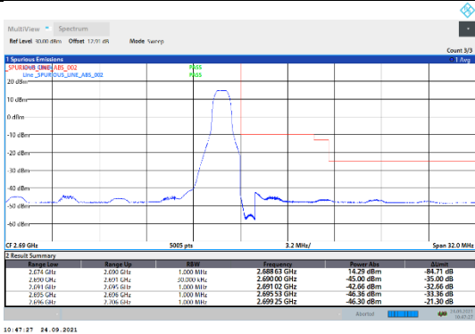
N41-30kHz-50MHz-CP-QPSK-High-Edge_1RB_Right---PASS
