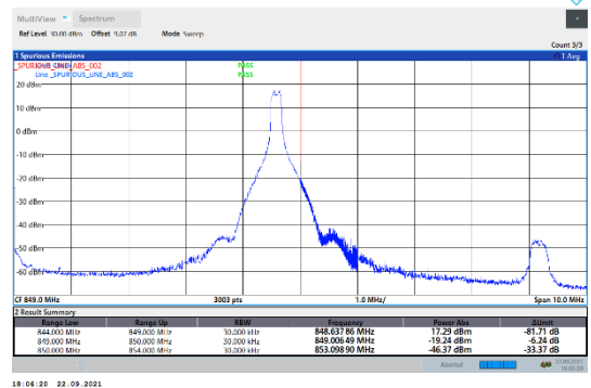
N5-15kHz-10MHz-DFT-QPSK-High-Edge_1RB_Right--PASS
