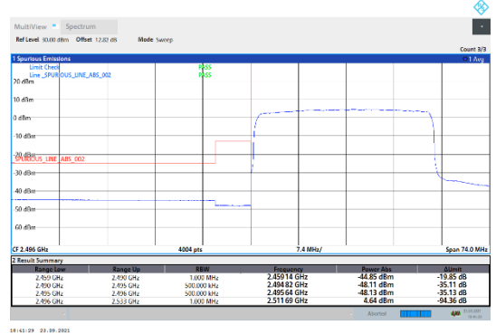
N41-30kHz-30MHz-DFT-QPSK-Low-Outer_Full---PASS
