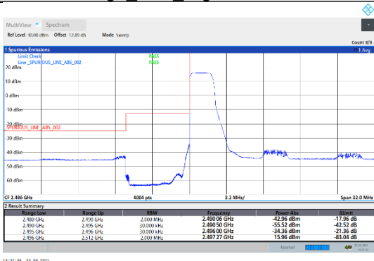
N41-30kHz-60MHz-CP-QPSK-Low-Edge_1RB_Left---PASS
