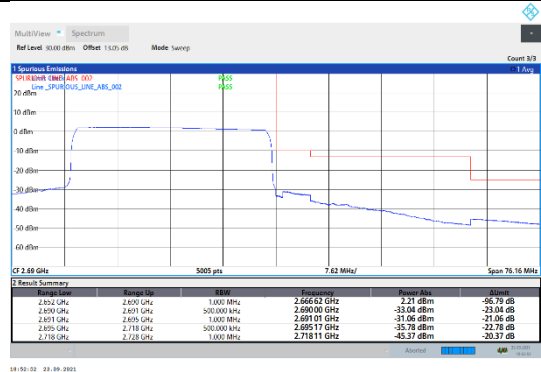
N41-30kHz-30MHz-CP-QPSK-High-Outer_Full---PASS
