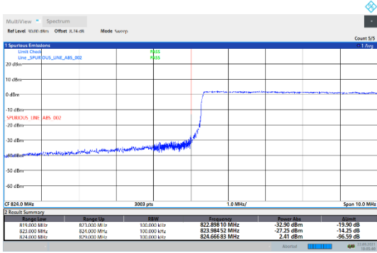
N5-15kHz-10MHz-CP-QPSK-Low-Outer_Full---PASS
