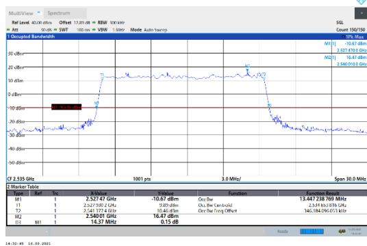
N7-15kHz-15MHz-DFT-256QAM-Mid-Outer_Full---PASS
