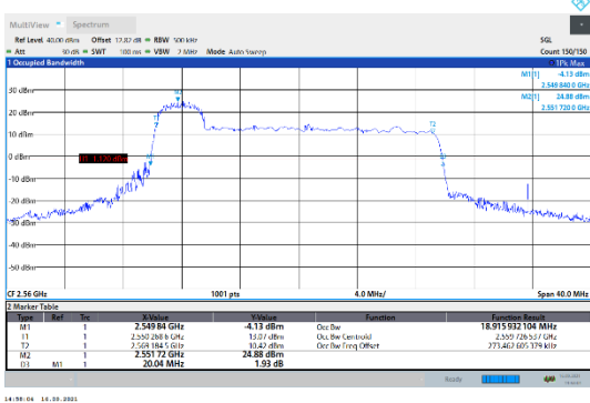
N7-15kHz-20MHz-CP-256QAM-High-Outer_Full---PASS
