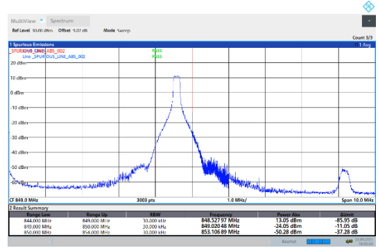
N5-15kHz-10MHz-CP-QPSK-High-Edge_1RB_Right--PASS
