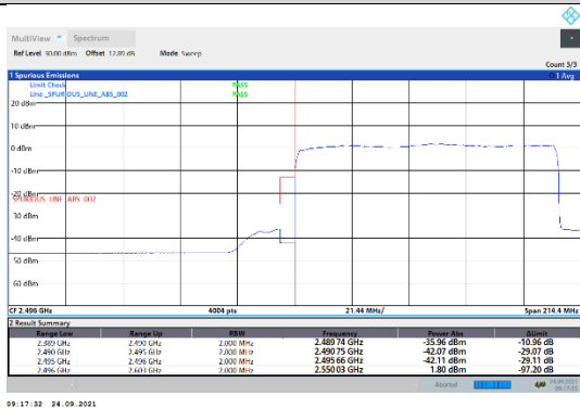
N41-30kHz-100MHz-DFT-QPSK-Low-Outer_Full---PASS
