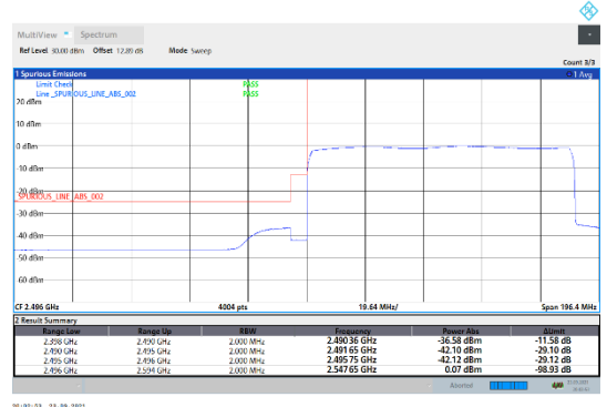
N41-30kHz-90MHz-CP-QPSK-Low-Outer_Full---PASS
