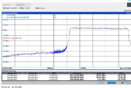
N5-15kHz-5MHz-DFT-QPSK-Low-Outer_Full---PASS
