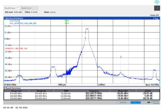
N5-15kHz-5MHz-DFT-QPSK-Low-Edge_1RB_Left---PASS
