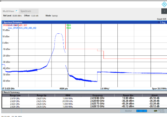
N38-30kHz-20MHz-CP-QPSK-High-Edge_1RB_Right---PASS
