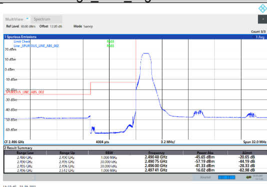
N41-30kHz-50MHz-CP-QPSK-Low-Edge_1RB_Left---PASS
