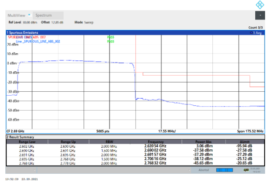
N41-30kHz-80MHz-DFT-QPSK-High-Outer_Full---PASS
