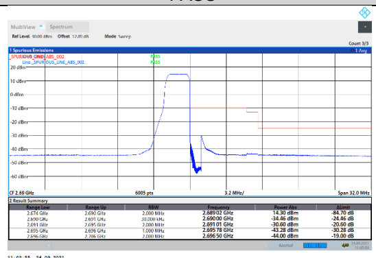
N41-30kHz-100MHz-CP-QPSK-High-Edge_1RB_Right---PASS
