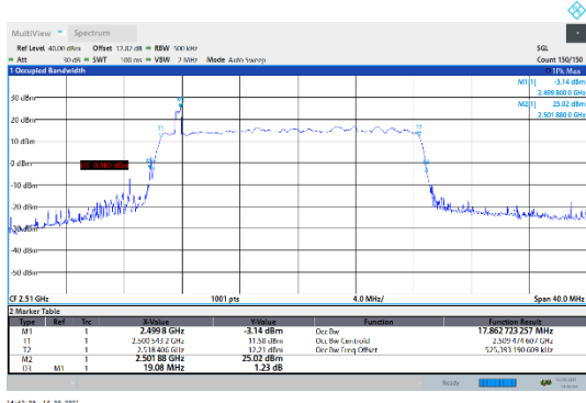
N7-15kHz-20MHz-DFT-256QAM-Low-Outer_Full--- PASS
