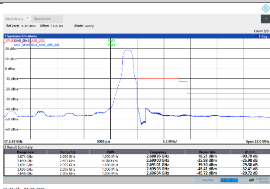
N41-30kHz-40MHz-DFT-QPSK-High-Edge_1RB_Right---PASS
