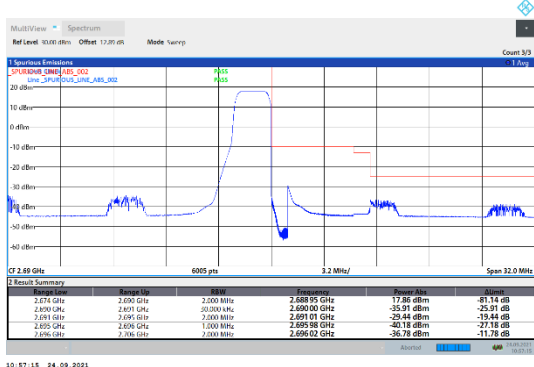
N41-30kHz-90MHz-DFT-QPSK-High-Edge_1RB_Right---PASS
