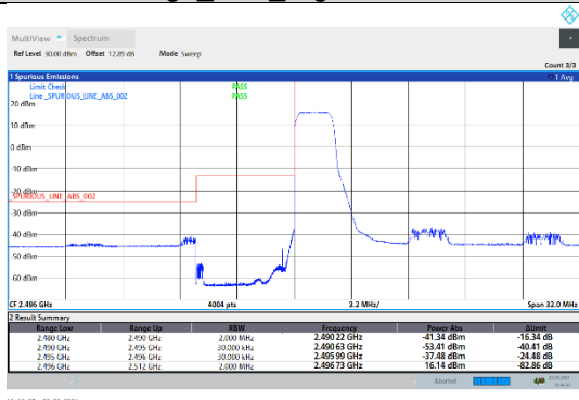
N41-30kHz-80MHz-CP-QPSK-Low-Edge_1RB_Left---PASS
