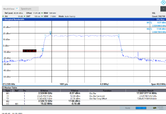
N7-15kHz-20MHz-DFT-64QAM-Mid-Outer_Full--- PASS
