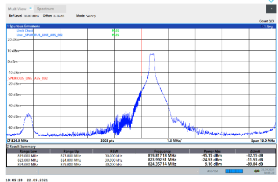
N5-15kHz-10MHz-CP-QPSK-Low-Edge_1RB_Left--PASS
