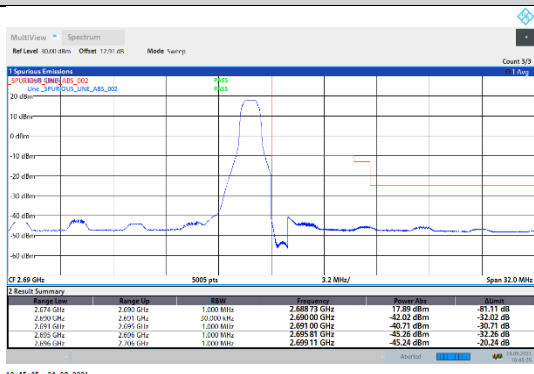
N41-30kHz-50MHz-DFT-QPSK-High-Edge_1RB_Right---PASS
