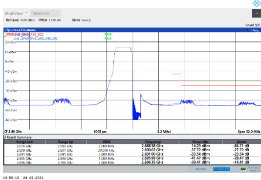
N41-30kHz-80MHz-CP-QPSK-High-Edge_1RB_Right---PASS
