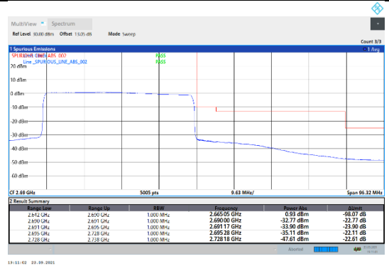
N41-30kHz-40MHz-CP-QPSK-High-Outer_Full---PASS
