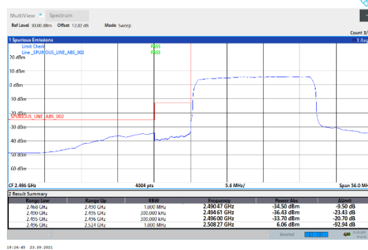
N41-30kHz-20MHz-DFT-QPSK-Low-Outer_Full---PASS
