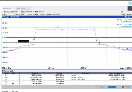
N7-15kHz-20MHz-DFT-16QAM-Low-Outer_Full--- PASS
