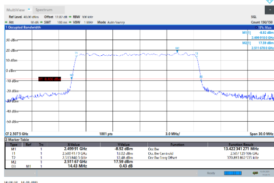
N7-15kHz-15MHz-DFT-64QAM-Low-Outer_Full---PASS
