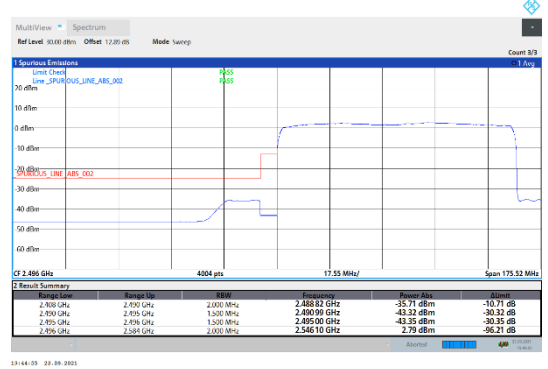
N41-30kHz-80MHz-DFT-QPSK-Low-Outer_Full---PASS
