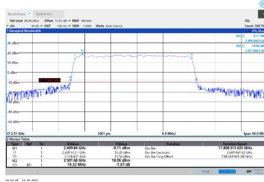
N7-15kHz-20MHz-DFT-64QAM-Low-Outer_Full--- PASS
