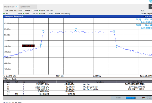
N7-15kHz-15MHz-CP-16QAM-Low-Outer_Full---PASS
