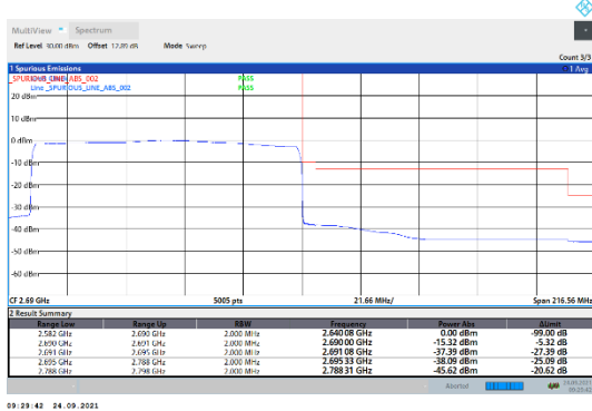
N41-30kHz-100MHz-CP-QPSK-High-Outer_Full---PASS
