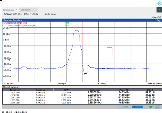
N41-30kHz-30MHz-CP-QPSK-High-Edge_1RB_Right---PASS
