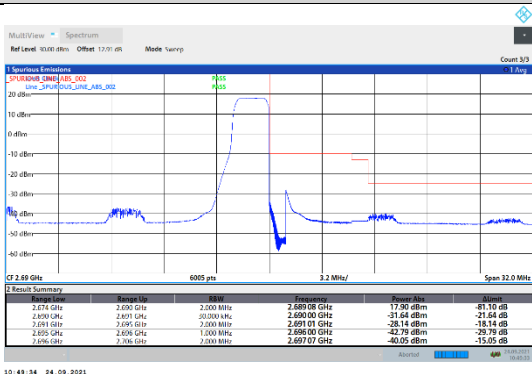
N41-30kHz-60MHz-DFT-QPSK-High-Edge_1RB_Right---PASS
