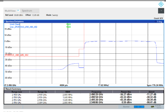
N41-30kHz-80MHz-CP-QPSK-Low-Outer_Full---PASS
