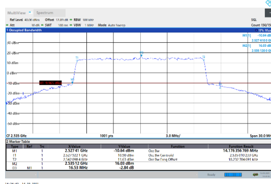
N7-15kHz-15MHz-CP-64QAM-Mid-Outer_Full---PASS
