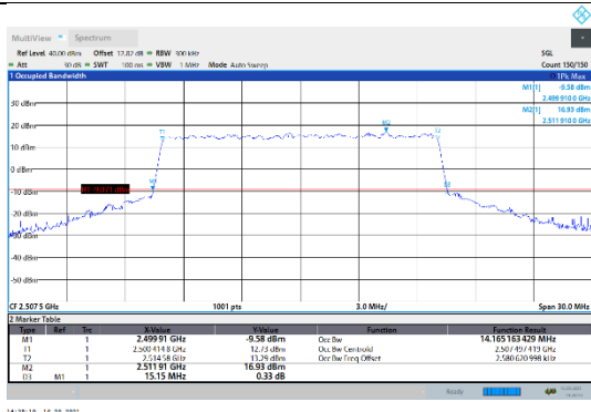
N7-15kHz-15MHz-CP-QPSK-Low-Outer_Full---PASS
