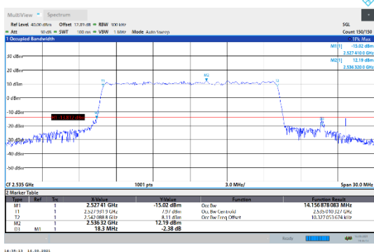
N7-15kHz-15MHz-CP-256QAM-Mid-Outer_Full---PASS
