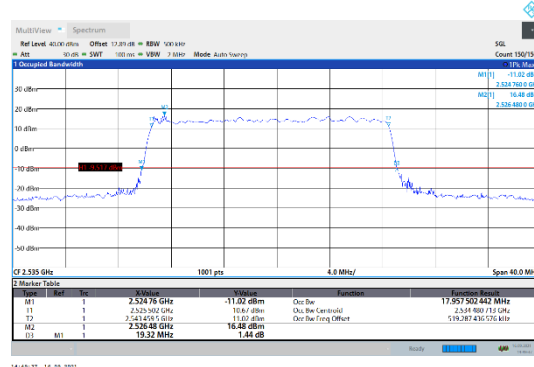
N7-15kHz-20MHz-DFT-256QAM-Mid-Outer_Full--- PASS
