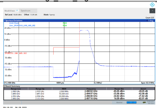
N41-30kHz-100MHz-CP-QPSK-Low-Edge_1RB_Left--PASS
