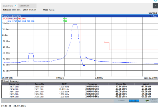
N41-30kHz-20MHz-DFT-QPSK-High-Edge_1RB_Right---PASS
