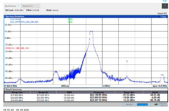
N5-15kHz-5MHz-CP-QPSK-Low-Edge_1RB_Left---PASS
