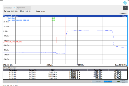
N41-30kHz-30MHz-CP-QPSK-Low-Outer_Full---PASS
