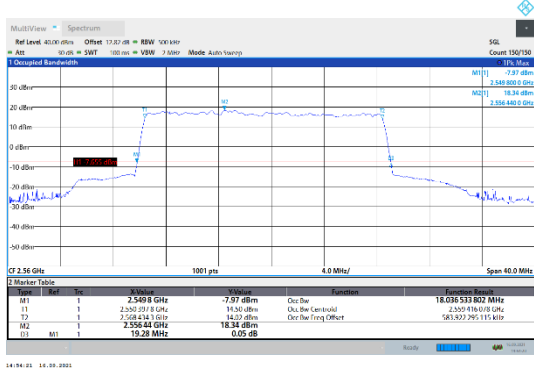
N7-15kHz-20MHz-DFT-16QAM-High-Outer_Full--- PASS
