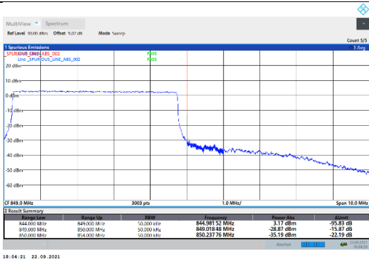
N5-15kHz-5MHz-CP-QPSK-High-Outer_Full---PASS
