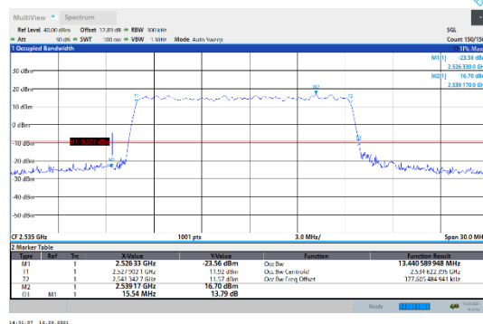
N7-15kHz-15MHz-DFT-64QAM-Mid-Outer_Full---PASS
