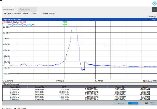
N41-30kHz-30MHz-DFT-QPSK-High-Edge_1RB_Right---PASS
