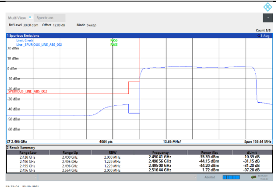
N41-30kHz-60MHz-CP-QPSK-Low-Outer_Full---PASS
