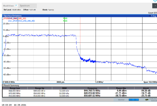
N5-15kHz-5MHz-DFT-QPSK-High-Outer_Full---PASS
