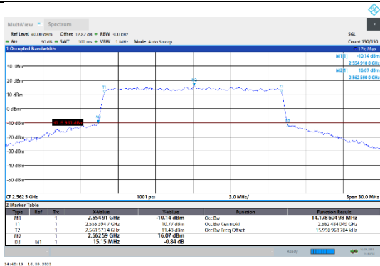
N7-15kHz-15MHz-CP-64QAM-High-Outer_Full---PASS
