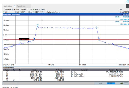
N7-15kHz-15MHz-CP-16QAM-High-Outer_Full---PASS
