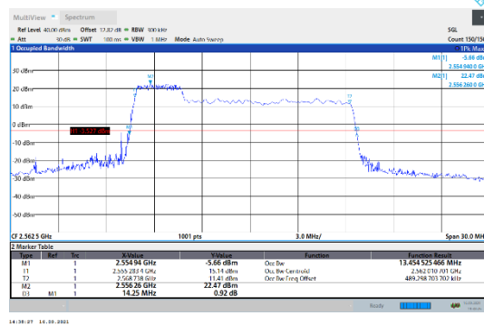
N7-15kHz-15MHz-DFT-256QAM-High-Outer_Full---PASS
