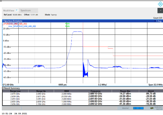
N41-30kHz-60MHz-CP-QPSK-High-Edge_1RB_Right--PASS
