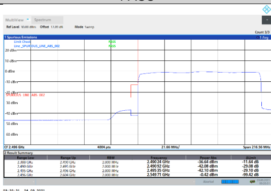
N41-30kHz-100MHz-CP-QPSK-Low-Outer_Full---PASS
