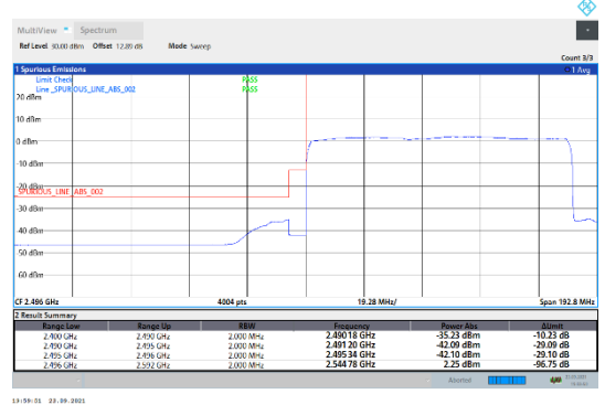
N41-30kHz-90MHz-DFT-QPSK-Low-Outer_Full---PASS
