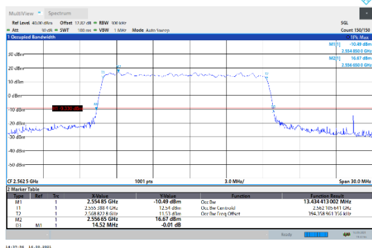
N7-15kHz-15MHz-DFT-64QAM-High-Outer_Full---PASS
