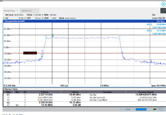
N7-15kHz-15MHz-DFT-16QAM-Mid-Outer_Full---PASS
