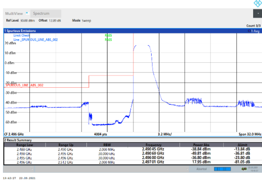
N41-30kHz-80MHz-DFT-QPSK-Low-Edge_1RB_Left---PASS
