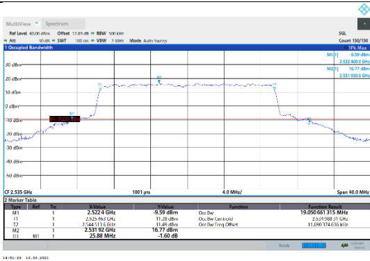
N7-15kHz-20MHz-CP-64QAM-Mid-Outer_Full---PASS
