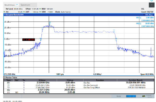
N7-15kHz-20MHz-CP-256QAM-Mid-Outer_Full---PASS
