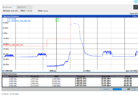
N41-30kHz-90MHz-DFT-QPSK-Low-Edge_1RB_Left---PASS
