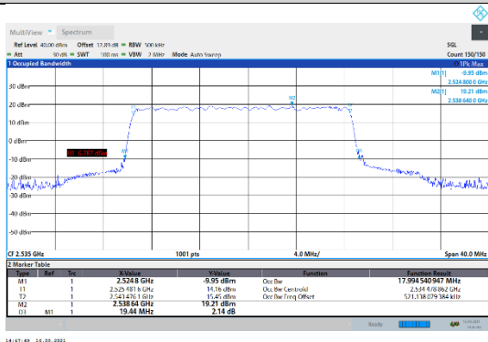
N7-15kHz-20MHz-DFT-QPSK-Mid-Outer_Full---PASS
