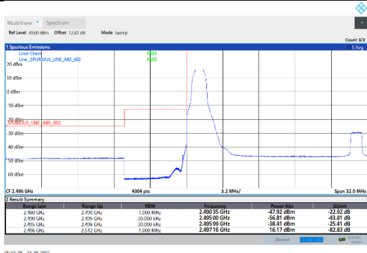
N41-30kHz-30MHz-CP-QPSK-Low-Edge_1RB_Left---PASS
