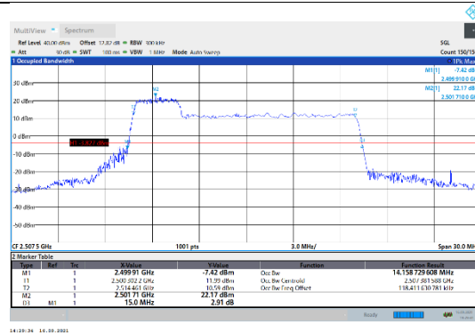
N7-15kHz-15MHz-CP-256QAM-Low-Outer_Full---PASS
