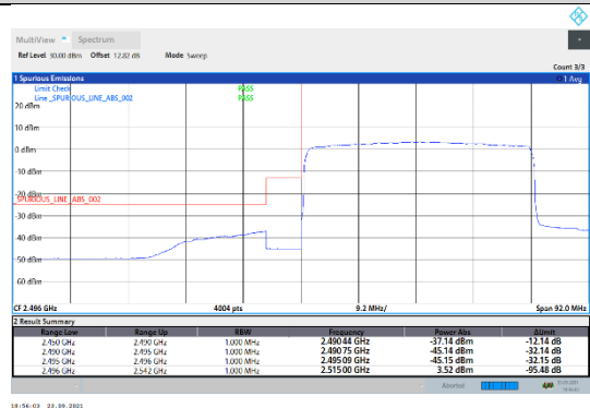
N41-30kHz-40MHz-DFT-QPSK-Low-Outer_Full---PASS
