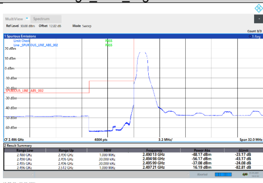
N41-30kHz-40MHz-CP-QPSK-Low-Edge_1RB_Left---PASS
