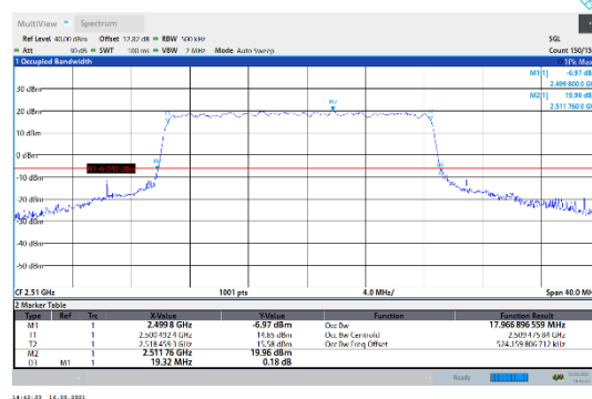
N7-15kHz-20MHz-DFT-QPSK-Low-Outer_Full---PASS
