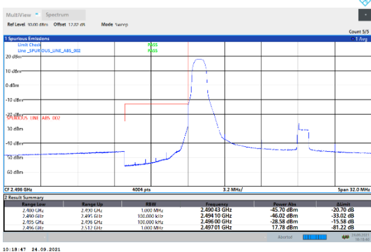
N41-30kHz-20MHz-DFT-QPSK-Low-Edge_1RB_Left---PASS
