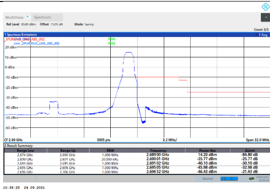
N41-30kHz-20MHz-CP-QPSK-High-Edge_1RB_Right---PASS
