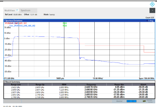
N41-30kHz-60MHz-DFT-QPSK-High-Outer_Full---PASS
