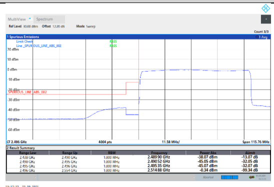
N41-30kHz-50MHz-CP-QPSK-Low-Outer_Full---PASS
