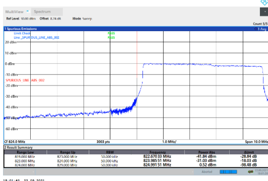
N5-15kHz-5MHz-CP-QPSK-Low-Outer_Full---PASS
