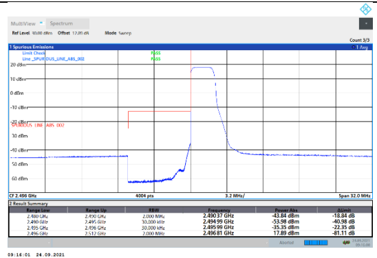
N41-30kHz-100MHz-DFT-QPSK-Low-Edge_1RB_Left--PASS
