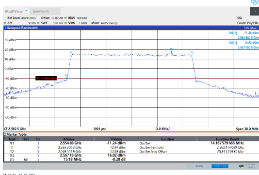
N7-15kHz-15MHz-CP-QPSK-High-Outer_Full---PASS
