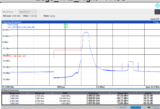
N41-30kHz-20MHz-CP-QPSK-Low-Edge_1RB_Left---PASS
