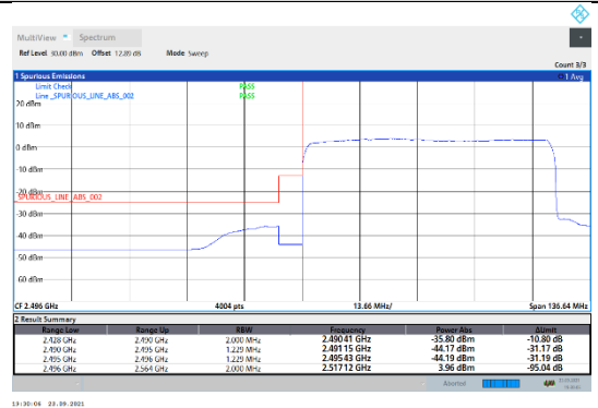
N41-30kHz-60MHz-DFT-QPSK-Low-Outer_Full---PASS
