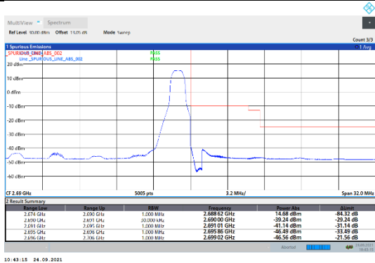
N41-30kHz-40MHz-CP-QPSK-High-Edge_1RB_Right--PASS
