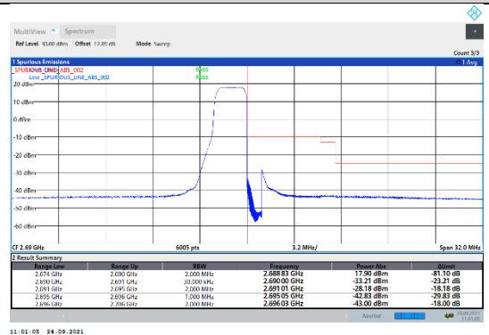
N41-30kHz-100MHz-DFT-QPSK-High-Edge_1RB_Right---PASS
