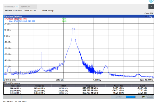
N5-15kHz-5MHz-CP-QPSK-High-Edge_1RB_Right---PASS
