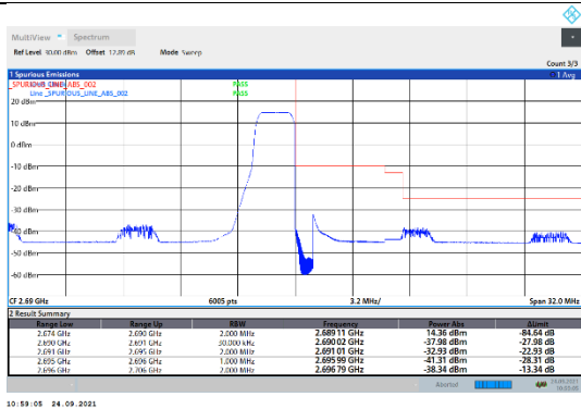
N41-30kHz-90MHz-CP-QPSK-High-Edge_1RB_Right--PASS
