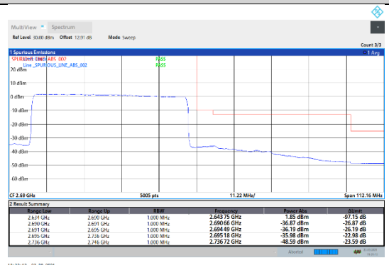
N41-30kHz-50MHz-DFT-QPSK-High-Outer_Full---PASS
