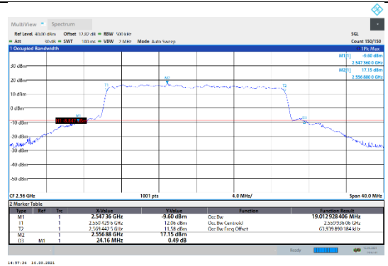
N7-15kHz-20MHz-CP-64QAM-High-Outer_Full---PASS
