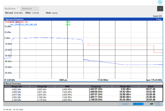
N41-30kHz-80MHz-CP-QPSK-High-Outer_Full---PASS
