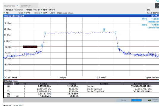
N7-15kHz-15MHz-DFT-256QAM-Low-Outer_Full---PASS
