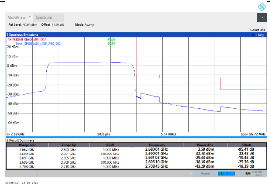
N41-30kHz-20MHz-CP-QPSK-High-Outer_Full---PASS
