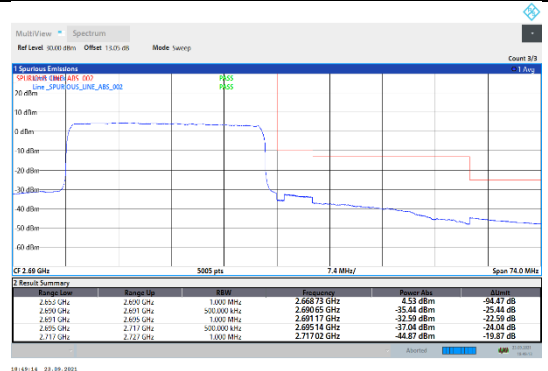
N41-30kHz-30MHz-DFT-QPSK-High-Outer_Full---PASS
