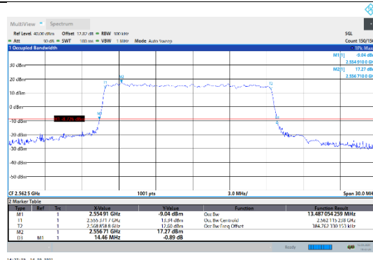
N7-15kHz-15MHz-DFT-16QAM-High-Outer_Full---PASS
