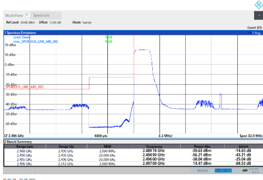
N41-30kHz-90MHz-CP-QPSK-Low-Edge_1RB_Left---PASS
