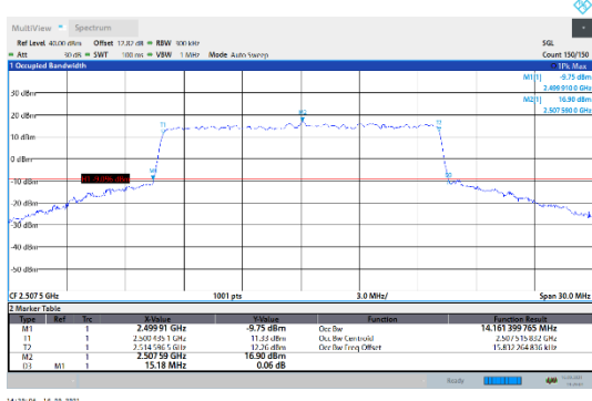
N7-15kHz-15MHz-CP-64QAM-Low-Outer_Full---PASS
