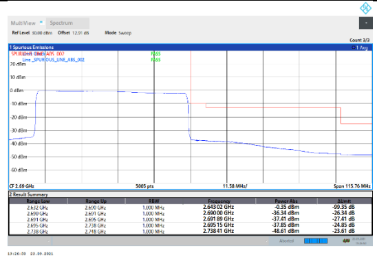
N41-30kHz-50MHz-CP-QPSK-High-Outer_Full---PASS
