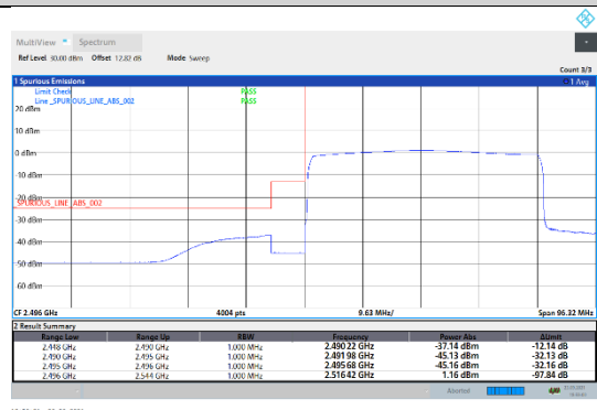
N41-30kHz-40MHz-CP-QPSK-Low-Outer_Full---PASS
