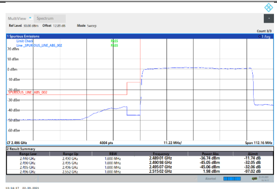
N41-30kHz-50MHz-DFT-QPSK-Low-Outer_Full---PASS
