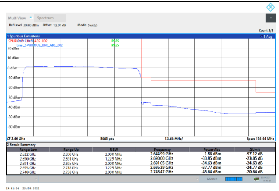
N41-30kHz-60MHz-CP-QPSK-High-Outer_Full---PASS
