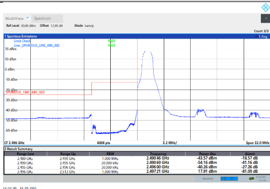
N41-30kHz-50MHz-DFT-QPSK-Low-Edge_1RB_Left---PASS
