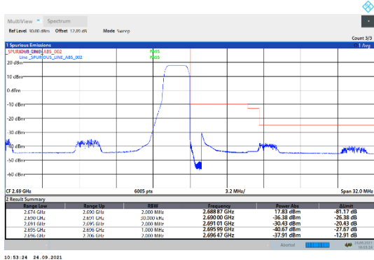
N41-30kHz-80MHz-DFT-QPSK-High-Edge_1RB_Right---PASS
