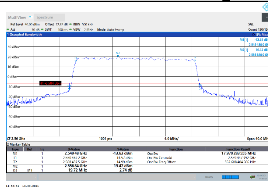
N7-15kHz-20MHz-DFT-QPSK-High-Outer_Full---PASS
