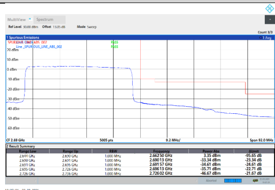
N41-30kHz-40MHz-DFT-QPSK-High-Outer_Full---PASS
