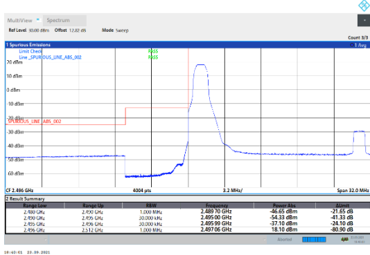
N41-30kHz-30MHz-DFT-QPSK-Low-Edge_1RB_Left---PASS
