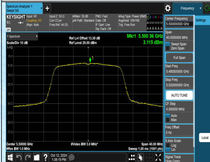
11AC20MIMO-Ant1-5500-PASS
