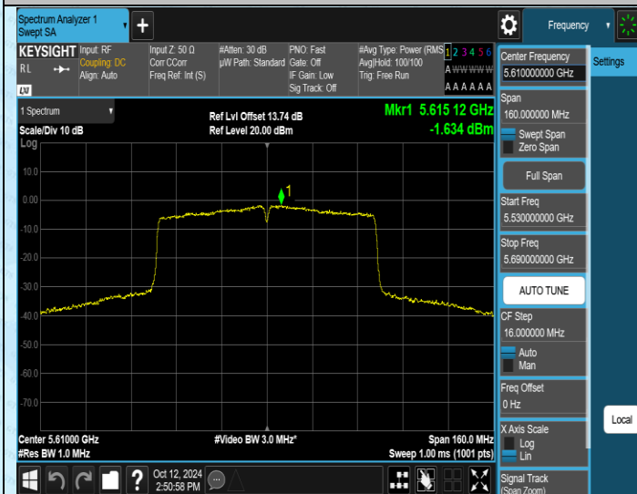
11AC80MIMO-Ant1-5610-PASS
