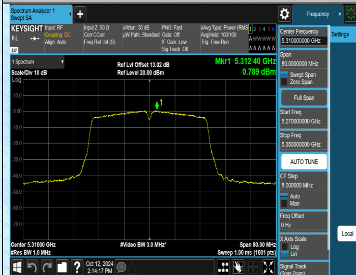
11AC40MIMO-Ant1-5310-PASS
