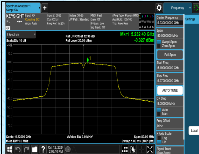
11AC40MIMO-Ant1-5230-PASS
