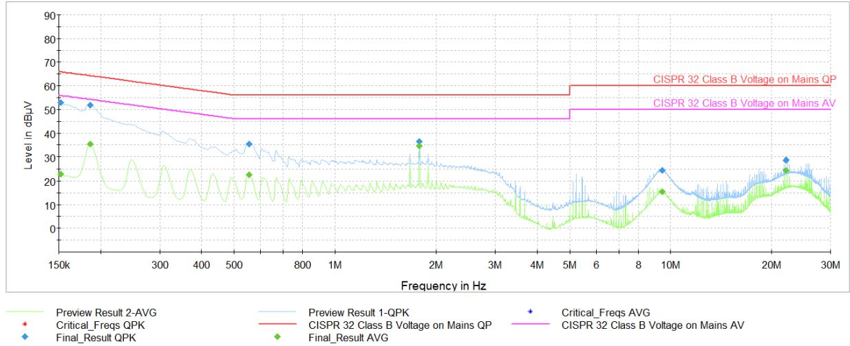
Plot 6-14. AC Line Conducted Plot (N - Mode 1, with Magnetic Charger & Laptop)
