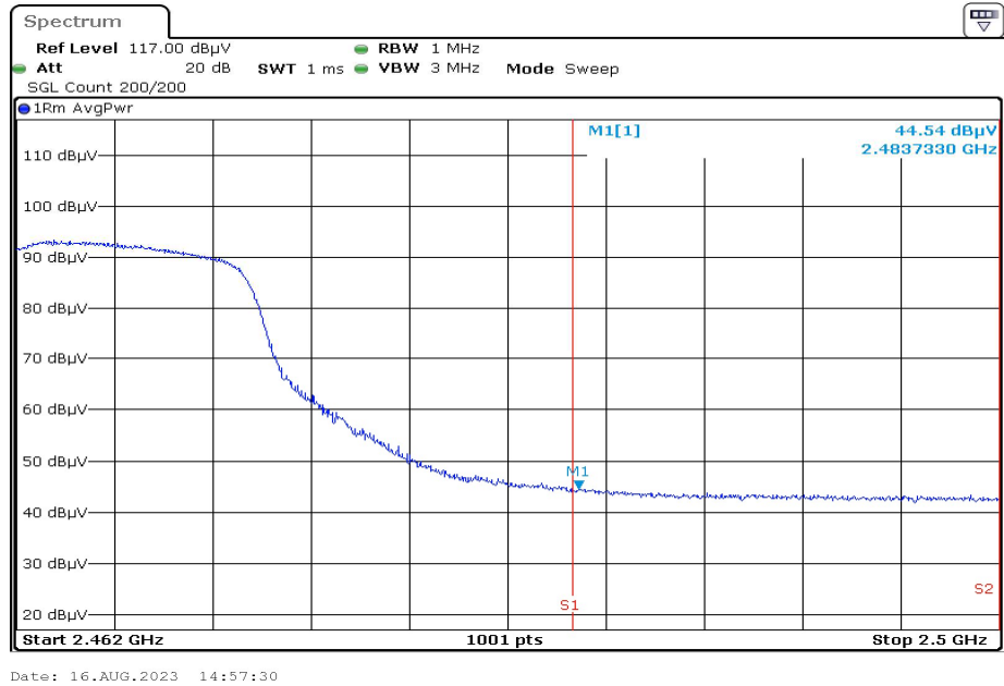
2462.0 F3 RestrictedBand Horizontal AVG
