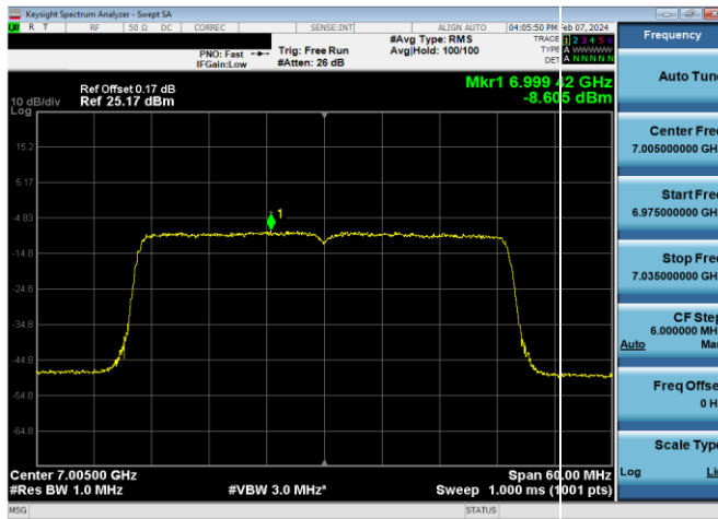
Plot 7-624. Power Spectral Density Plot SDM Diversity Antenna 2a LPI (40MHz 802.11ax (UNII Band 8) – Ch. 211, MCS4)
