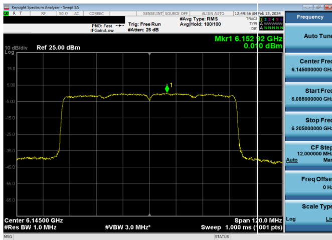
Plot 7-661. Power Spectral Density Plot SDM Diversity Antenna 2a Standard Power (80MHz 802.11ax (UNII Band 5) – Ch. 39, MCS11)
