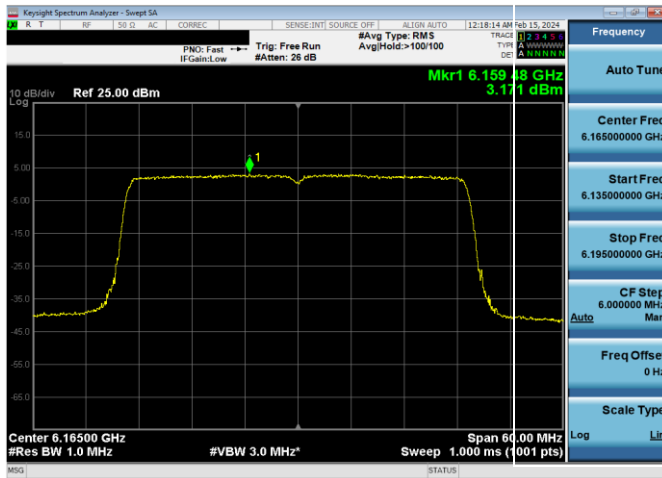
Plot 7-644. Power Spectral Density Plot SDM Diversity Antenna 2a Standard Power (40MHz 802.11ax (UNII Band 5) – Ch. 43, MCS2)
