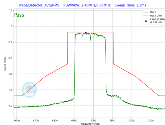
Plot 7-706. LPI In-Band Emission Plot Antenna WF5B (160MHz 802.11ax (UNII Band 8) – Ch. 207, MCS4)
