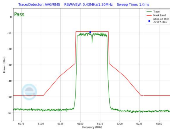
Plot 7-709. LPI In-Band Emission Plot Antenna WF5B (40MHz 802.11ax (UNII Band 5) – Ch. 43, MCS11)
