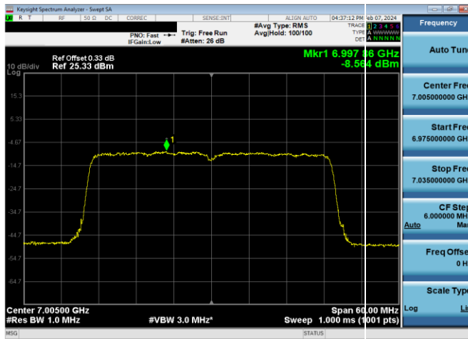
Plot 7-640. Power Spectral Density Plot SDM Diversity Antenna 2a LPI (40MHz 802.11ax (UNII Band 8) – Ch. 211, MCS11)
