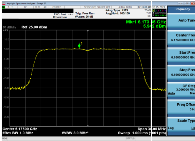
Plot 7-659. Power Spectral Density Plot SDM Diversity Antenna 2a Standard Power (20MHz 802.11ax (UNII Band 5) – Ch. 45, MCS11)
