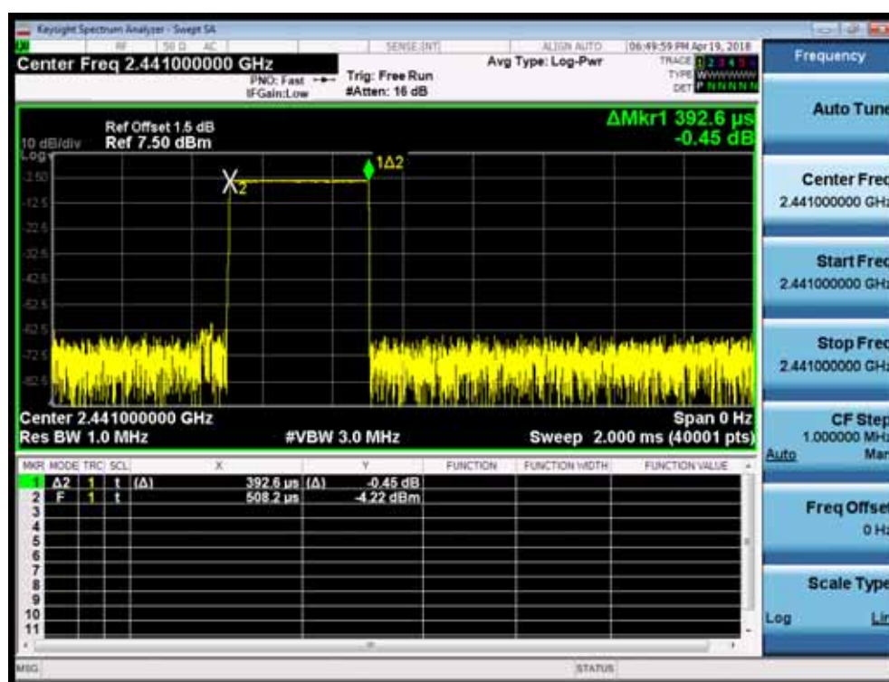
Channel 39 (2441MHz)-(DH1)
