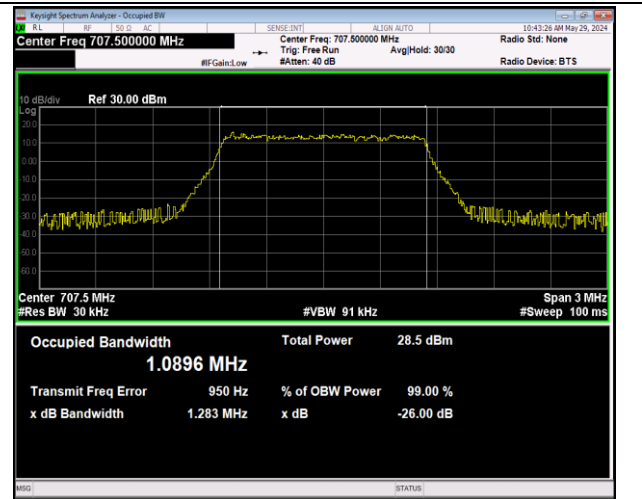
Band12-1.4MHz-64QAM-23095-6RB#0-PASS
