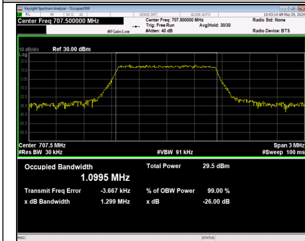
Band12-1.4MHz-16QAM-23095-6RB#0-PASS
