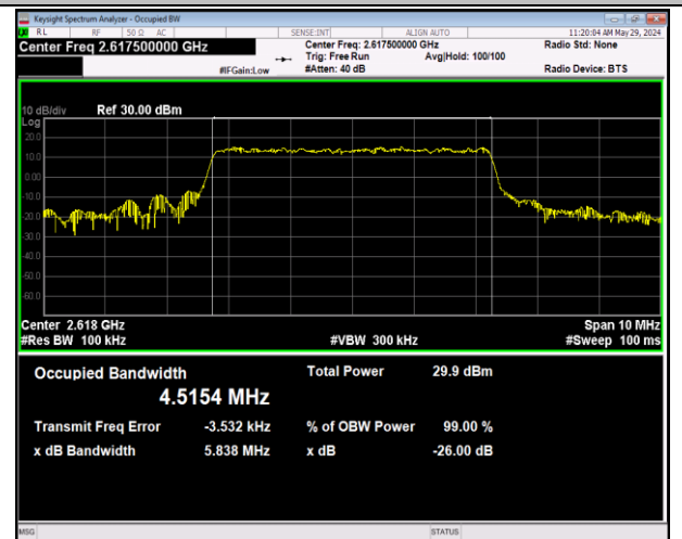
Band38-5MHz-16QAM-38225-25RB#0-PASS
