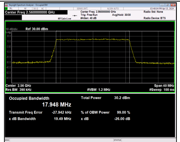
Band7-20MHz-64QAM-21350-100RB#0-PASS
