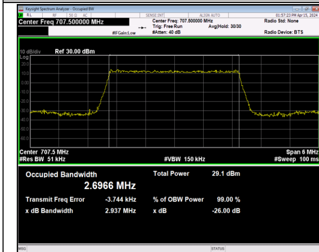
Band12-3MHz-64QAM-23095-15RB#0-PASS
