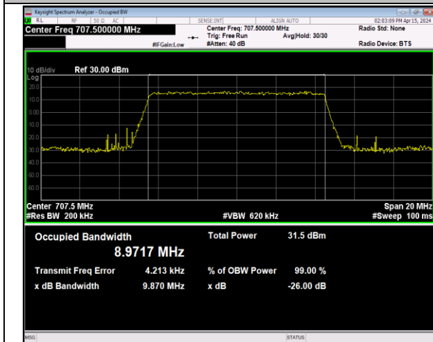
Band12-10MHz-QPSK-23095-50RB#0-PASS
