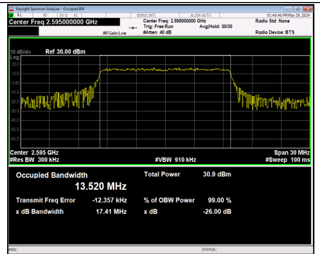
Band38-15MHz-QPSK-38000-75RB#0-PASS
