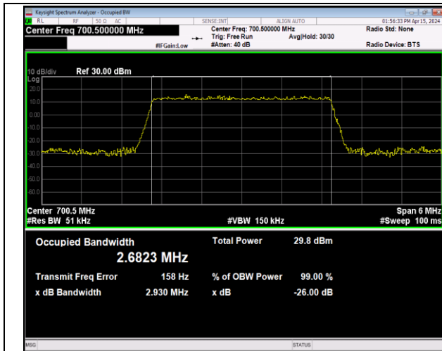
Band12-3MHz-16QAM-23025-15RB#0-PASS
