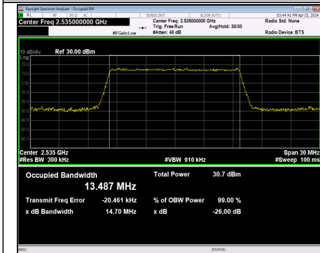
Band7-15MHz-16QAM-21100-75RB#0-PASS
