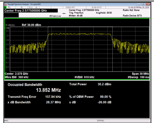
Band38-15MHz-16QAM-37825-75RB#0-PASS
