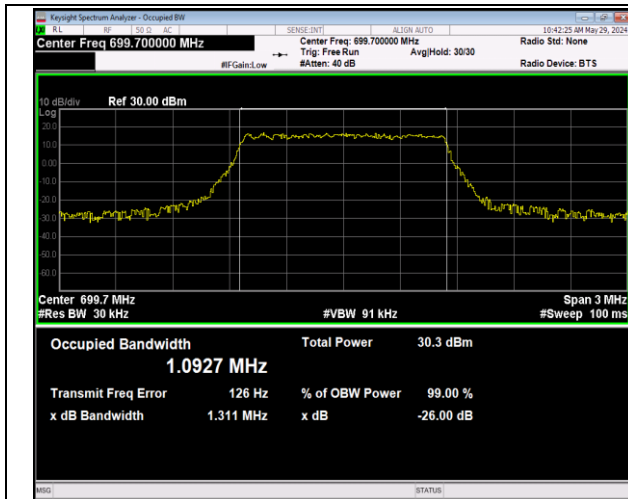
Band12-1.4MHz-QPSK-23017-6RB#0-PASS
