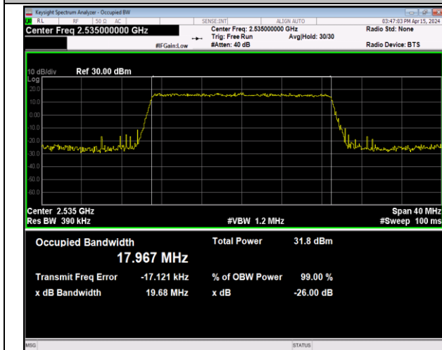
Band7-20MHz-QPSK-21100-100RB#0-PASS
