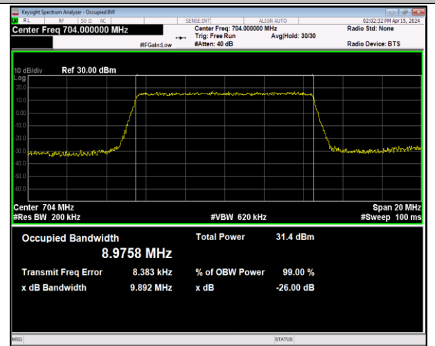
Band12-10MHz-QPSK-23060-50RB#0-PASS
