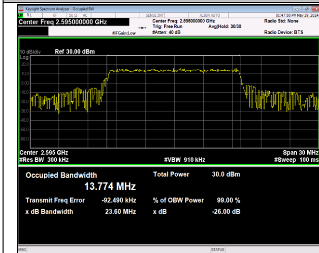
Band38-15MHz-16QAM-38000-75RB#0-PASS
