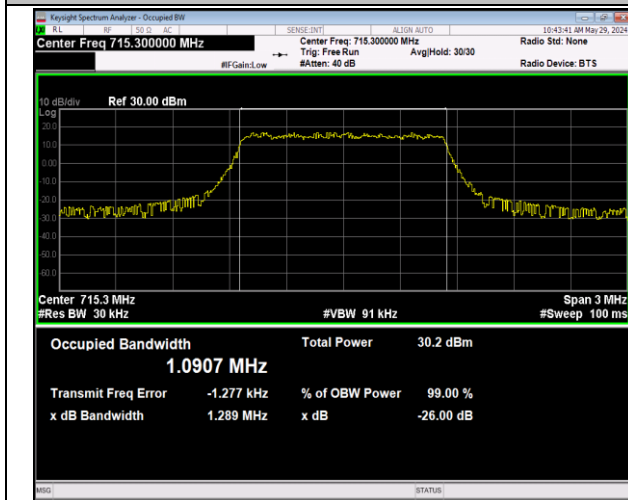
Band12-1.4MHz-QPSK-23173-6RB#0-PASS
