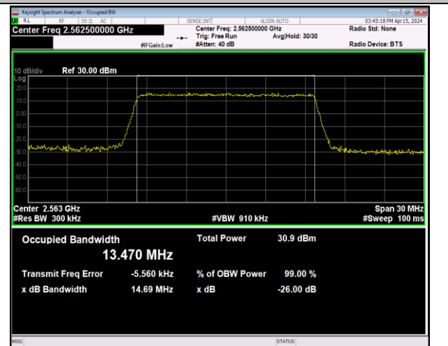
Band7-15MHz-16QAM-21375-75RB#0-PASS
