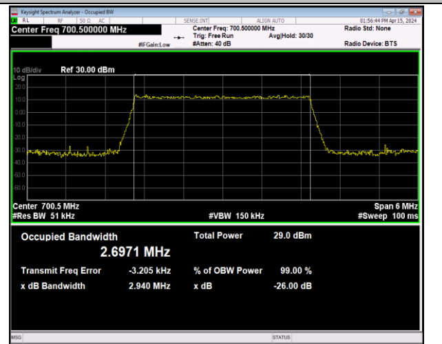
Band12-3MHz-64QAM-23025-15RB#0-PASS
