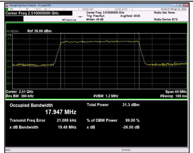
Band7-20MHz-QPSK-20850-100RB#0-PASS
