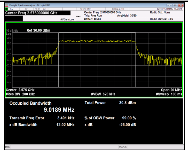
Band38-10MHz-QPSK-37800-50RB#0-PASS
