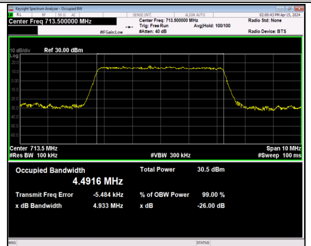
Band12-5MHz-16QAM-23155-25RB#0-PASS
