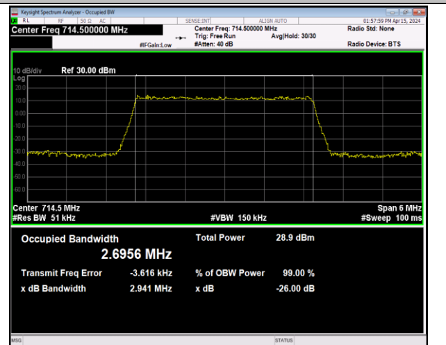
Band12-3MHz-64QAM-23165-15RB#0-PASS
