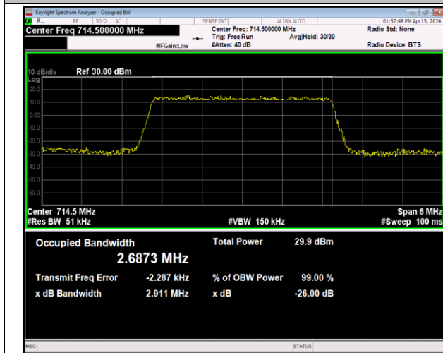
Band12-3MHz-16QAM-23165-15RB#0-PASS
