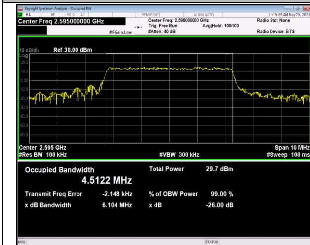
Band38-5MHz-16QAM-38000-25RB#0-PASS
