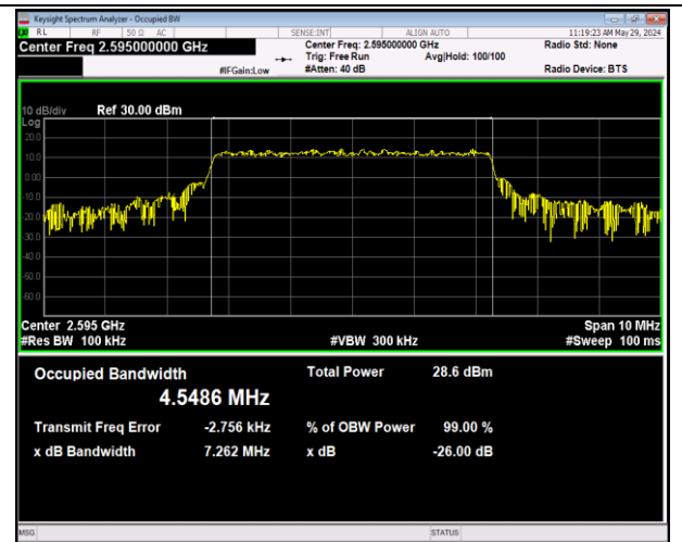
Band38-5MHz-64QAM-38000-25RB#0-PASS
