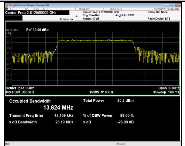
Band38-15MHz-16QAM-38175-75RB#0-PASS
