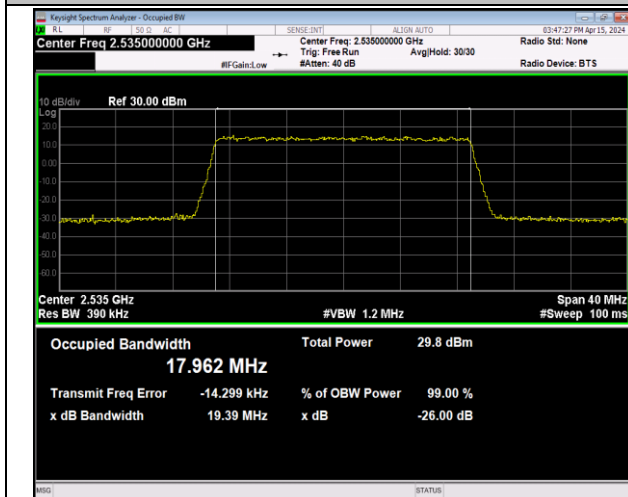
Band7-20MHz-64QAM-21100-100RB#0-PASS
