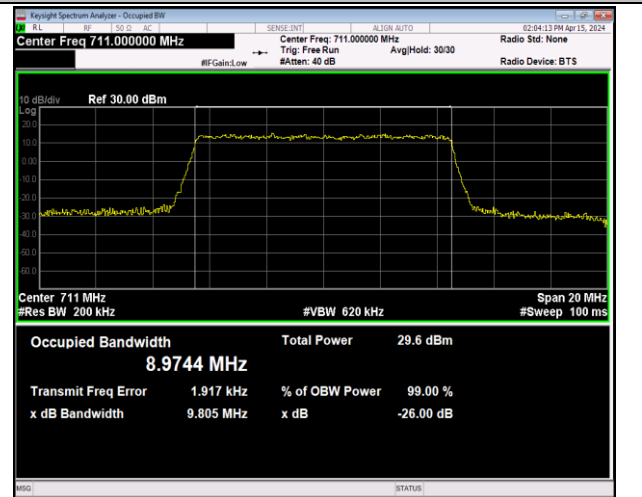
Band12-10MHz-64QAM-23130-50RB#0-PASS
