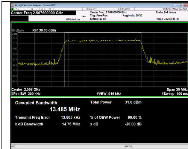
Band7-15MHz-QPSK-20825-75RB#0-PASS
