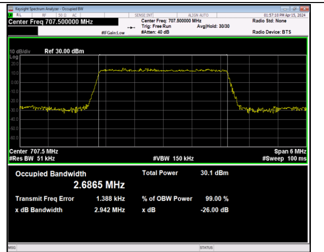
Band12-3MHz-16QAM-23095-15RB#0-PASS
