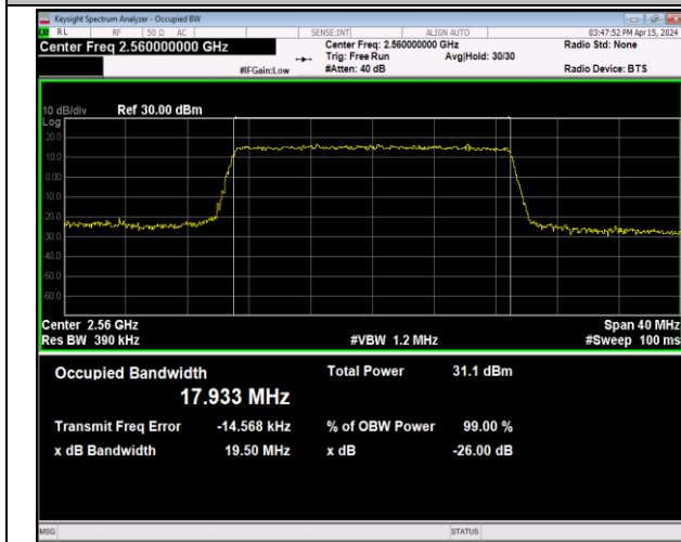
Band7-20MHz-16QAM-21350-100RB#0-PASS
