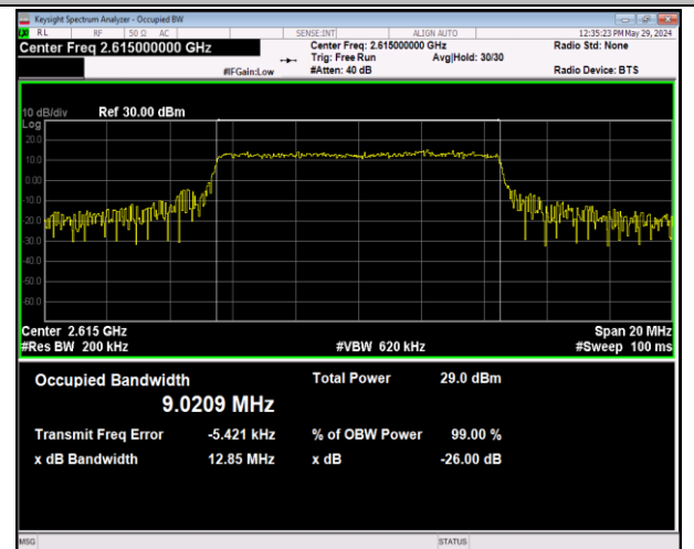
Band38-10MHz-64QAM-38200-50RB#0-PASS
