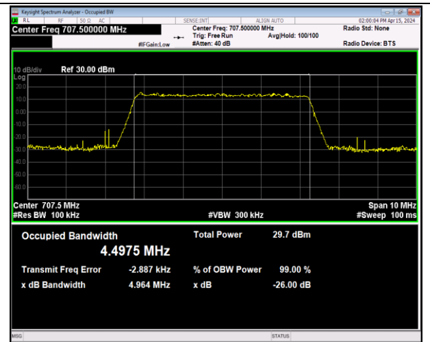
Band12-5MHz-64QAM-23095-25RB#0-PASS
