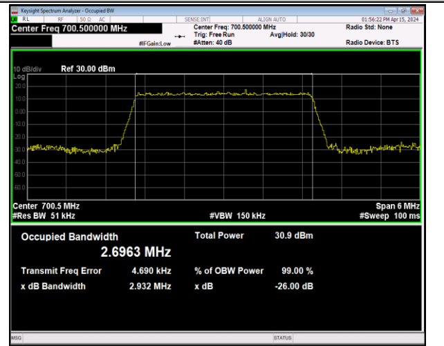
Band12-3MHz-QPSK-23025-15RB#0-PASS
