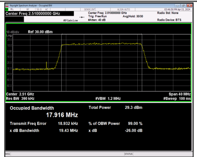
Band7-20MHz-64QAM-20850-100RB#0-PASS
