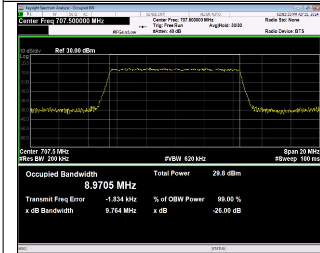
Band12-10MHz-64QAM-23095-50RB#0-PASS
