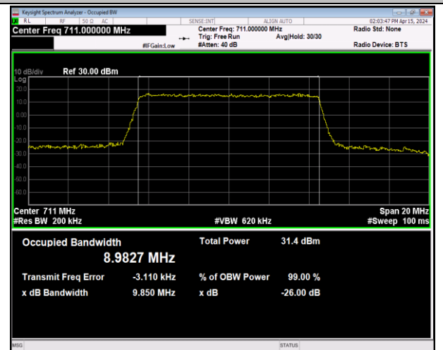
Band12-10MHz-QPSK-23130-50RB#0-PASS
