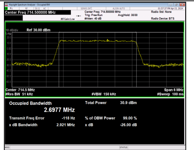
Band12-3MHz-QPSK-23165-15RB#0-PASS
