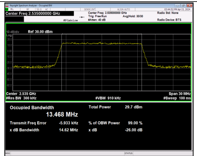
Band7-15MHz-64QAM-21100-75RB#0-PASS
