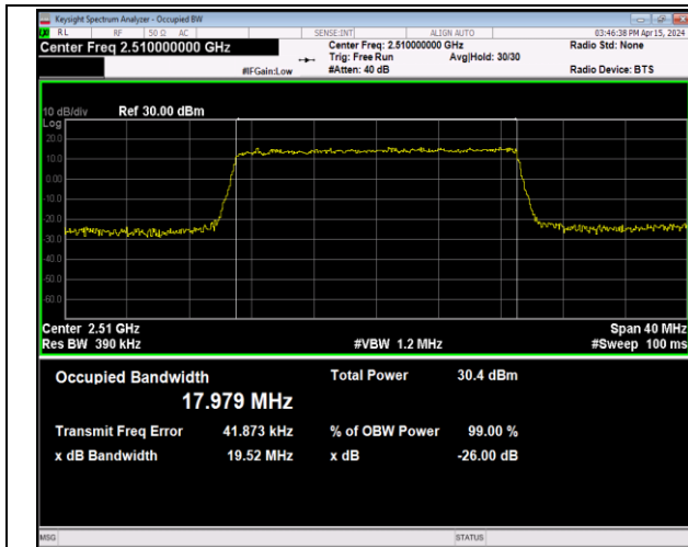
Band7-20MHz-16QAM-20850-100RB#0-PASS
