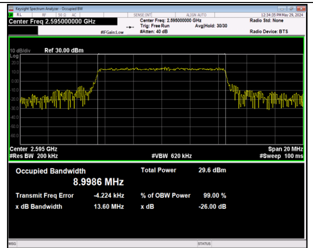
Band38-10MHz-16QAM-38000-50RB#0-PASS
