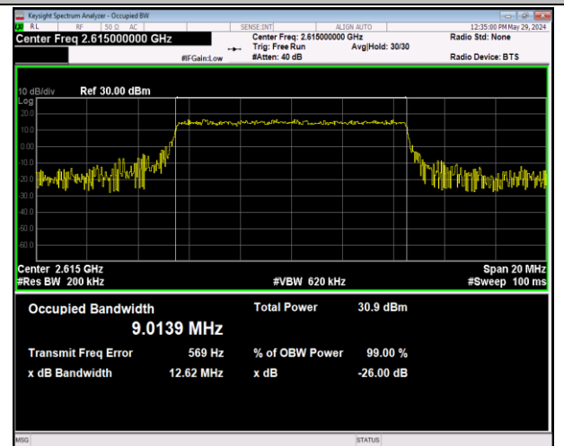
Band38-10MHz-QPSK-38200-50RB#0-PASS
