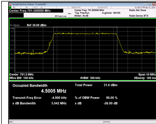
Band12-5MHz-QPSK-23035-25RB#0-PASS
