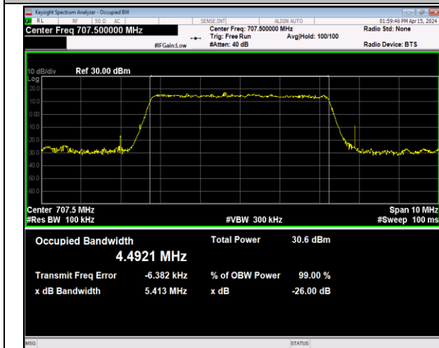
Band12-5MHz-16QAM-23095-25RB#0-PASS
