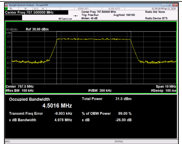
Band12-5MHz-QPSK-23095-25RB#0-PASS
