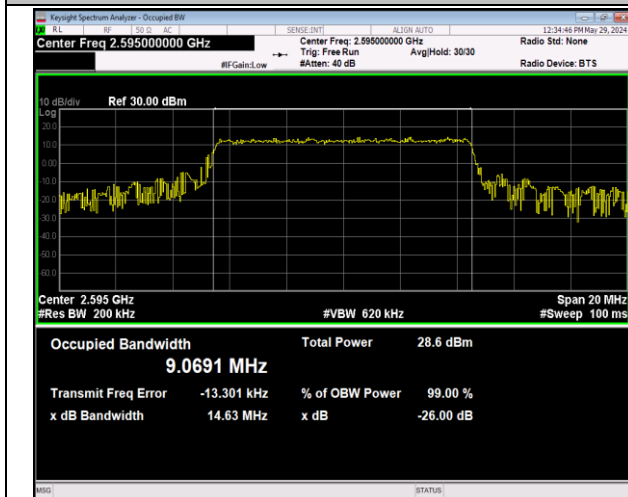
Band38-10MHz-64QAM-38000-50RB#0-PASS
