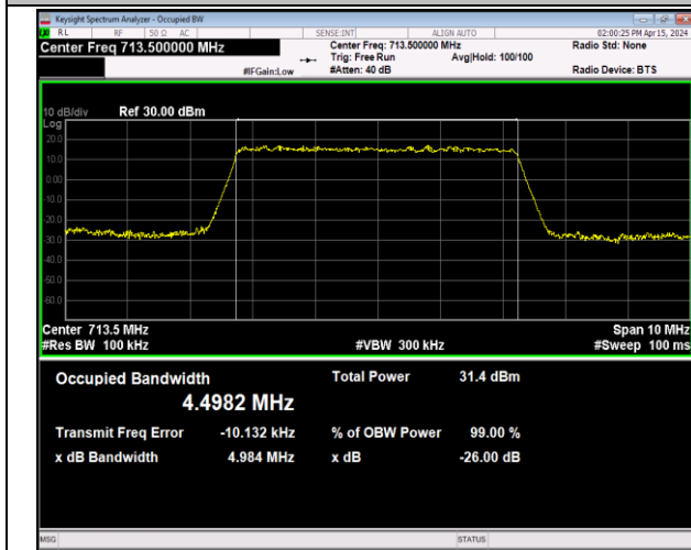
Band12-5MHz-QPSK-23155-25RB#0-PASS
