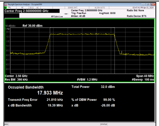
Band7-20MHz-QPSK-21350-100RB#0-PASS
