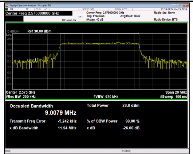
Band38-10MHz-64QAM-37800-50RB#0-PASS
