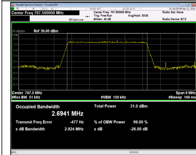
Band12-3MHz-QPSK-23095-15RB#0-PASS
