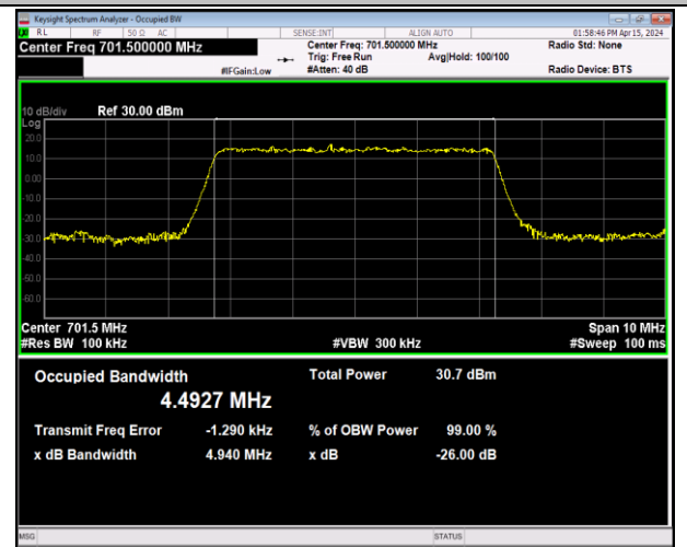
Band12-5MHz-16QAM-23035-25RB#0-PASS
