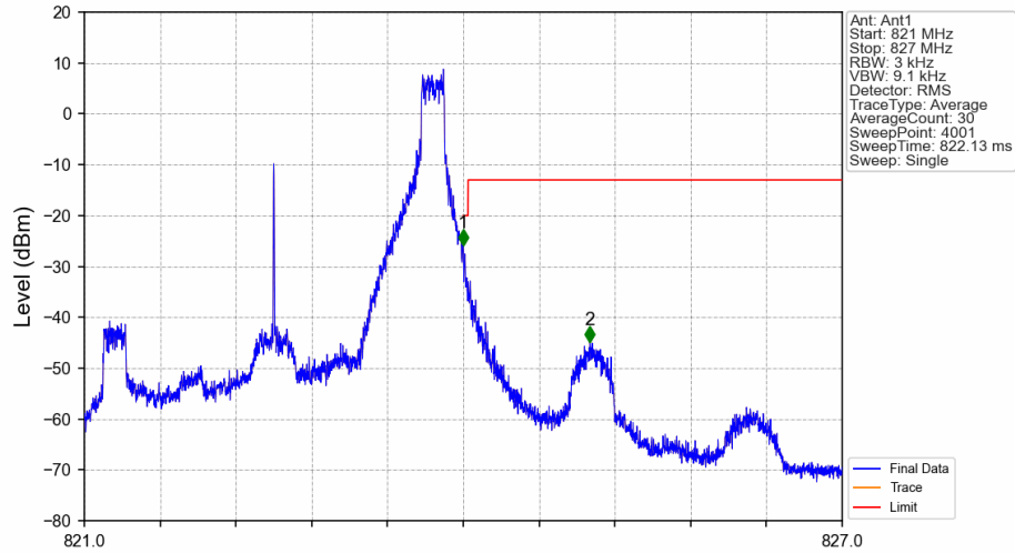
Band26a_3MHz_16QAM_HCH_822.5MHz_RB_1_14_NTNV
