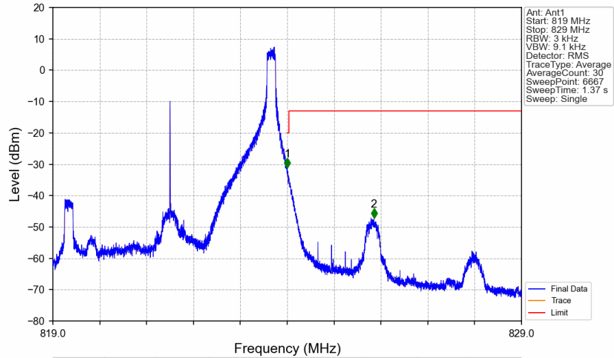
Band26a_5MHz_16QAM_HCH_821.5MHz_RB_1_24_NTNV
