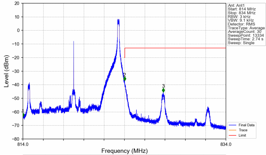
Band26a_10MHz_16QAM_MCH_819MHz_RB_1_49_NTNV
