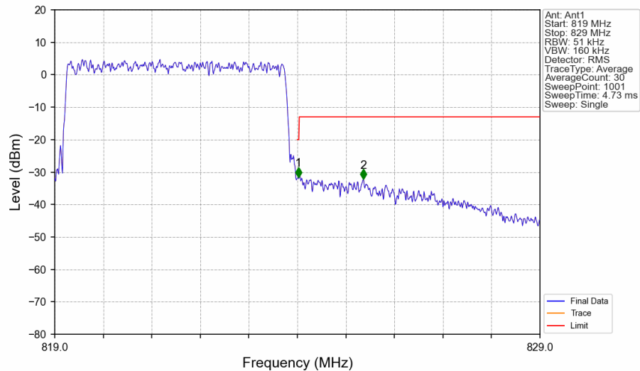
Band26a_5MHz_16QAM_HCH_821.5MHz_RB_25_0_NTNV
