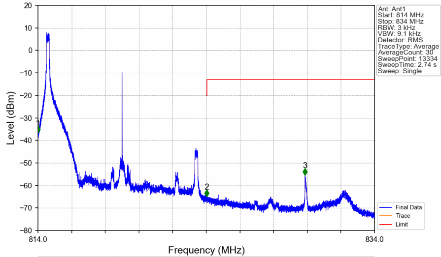
Band26a_10MHz_16QAM_MCH_819MHz_RB_1_0_NTNV
