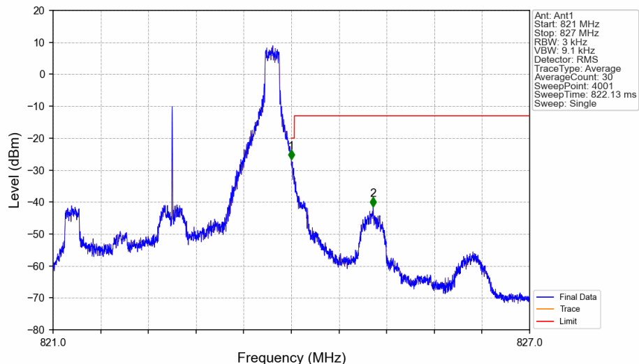
Band26a_3MHz_QPSK_HCH_822.5MHz_RB_1_14_NTNV
