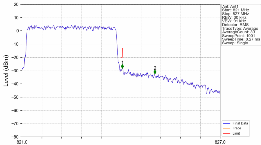
Band26a_3MHz_16QAM_HCH_822.5MHz_RB_15_0_NTNV
