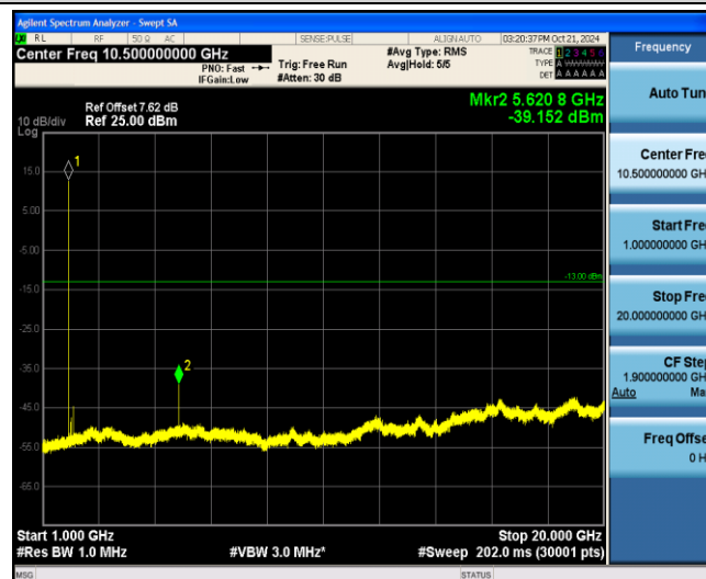
Band2-15MHz-QPSK-18900-1-0-Low-1000-20000--39.15-PASS
