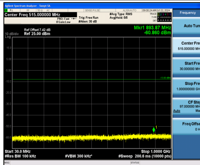
Band2-1.4MHz-16QAM-19193-1-0-Low-30-1000--60.86-PASS
