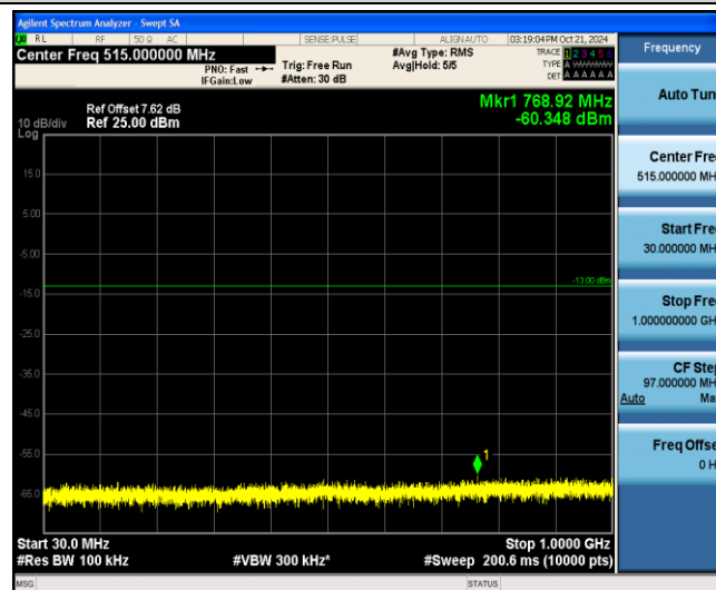
Band2-15MHz-16QAM-18675-1-0-Low-30-1000--60.35-PASS
