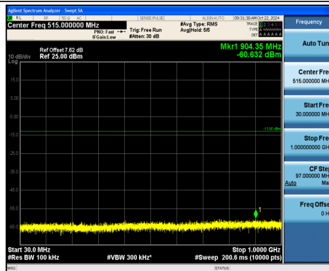
Band2-3MHz-16QAM-18615-1-0-Low-30-1000--60.63-PASS
