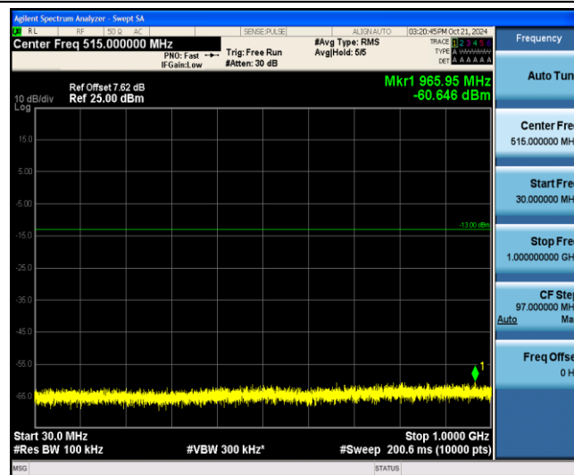
Band2-15MHz-16QAM-18900-1-0-Low-30-1000--60.65-PASS
