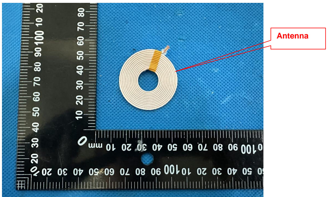
EUT Housing and Board View 10
