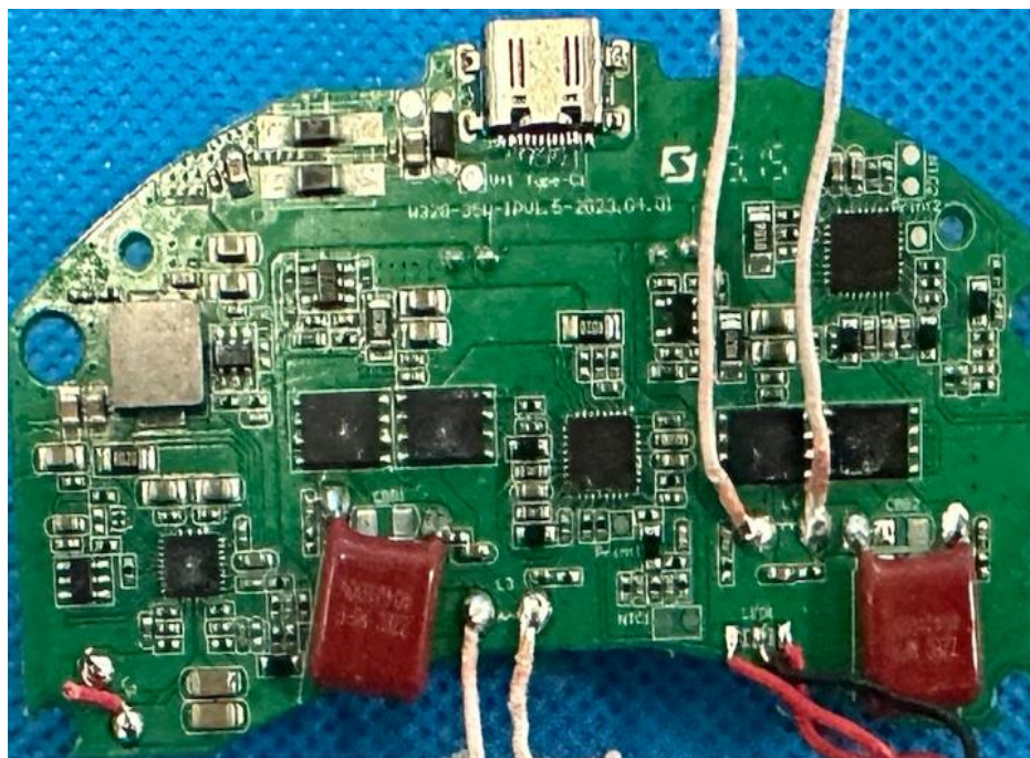
EUT Housing and Board View 6
