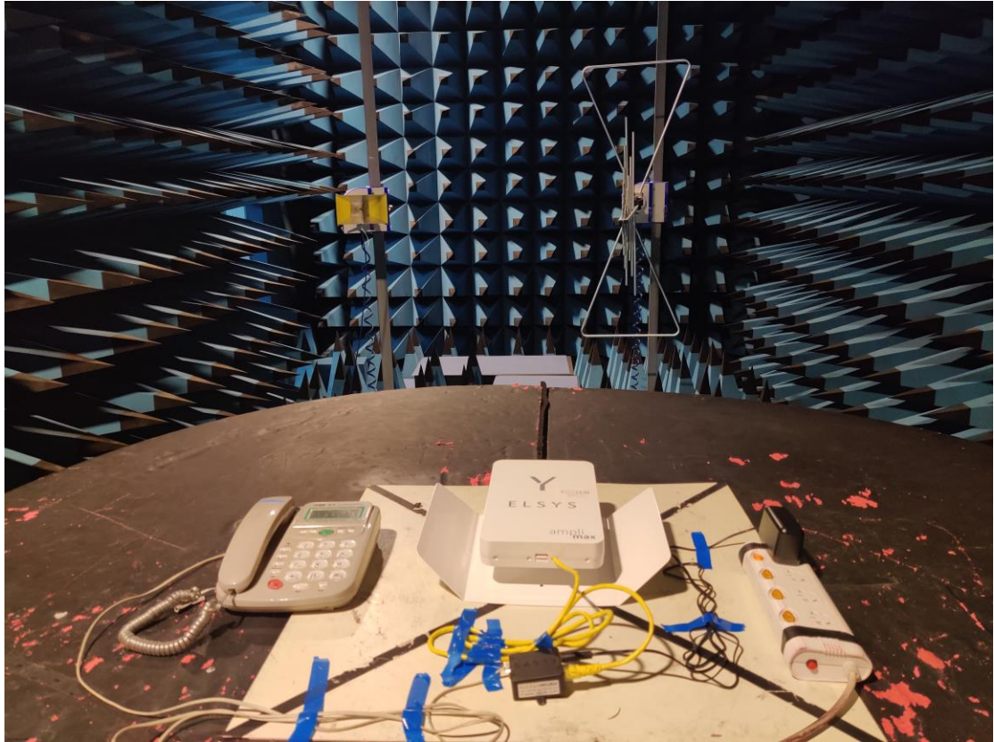
Radiated Emission -Front
