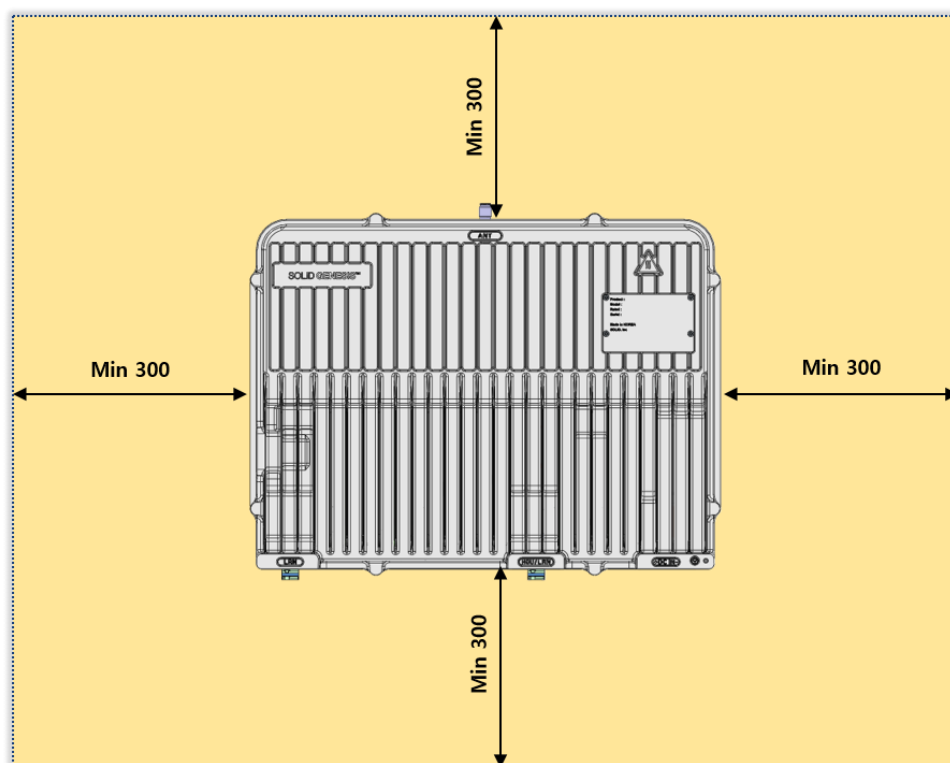
Figure 4.5 LRN Installation Clearance
