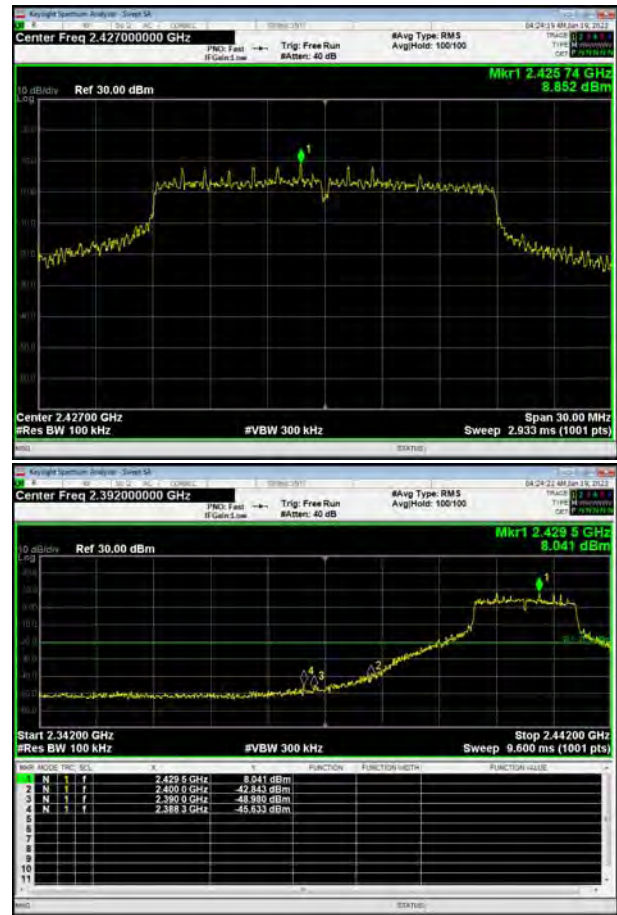
802.11n(HT20), Channel No. 4
