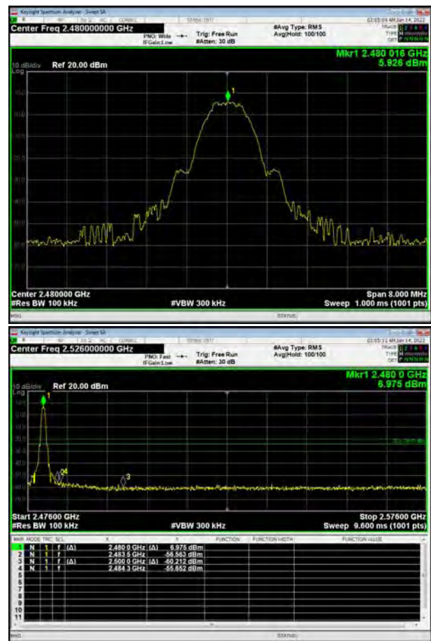
Bluetooth LE, Channel No.: 39
