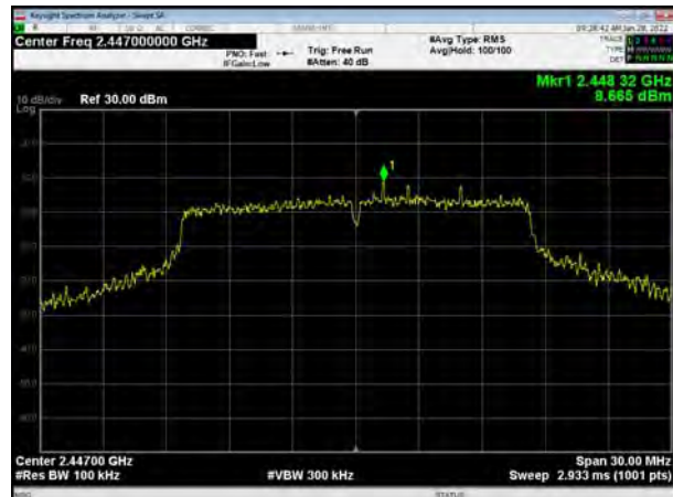
802.11g, Channel No.: 8
