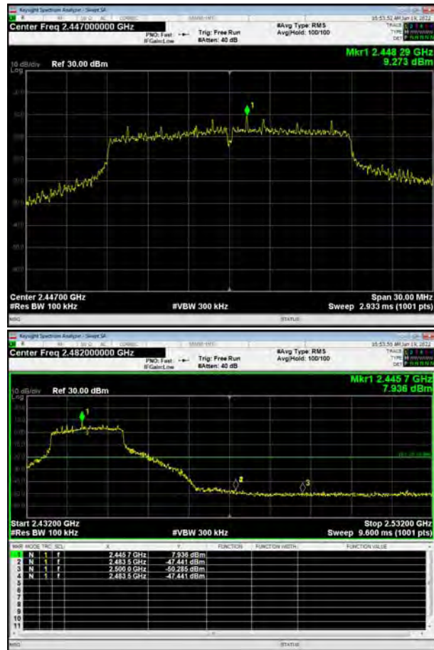
802.11n(HT20), Channel No. 8
