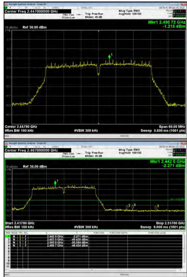
802.11n(HT40), Channel No. 8
