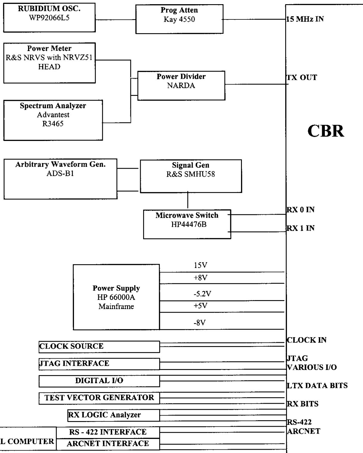
Figure: 12A. Test Configuration For Measurement of Quality Factor “p”
