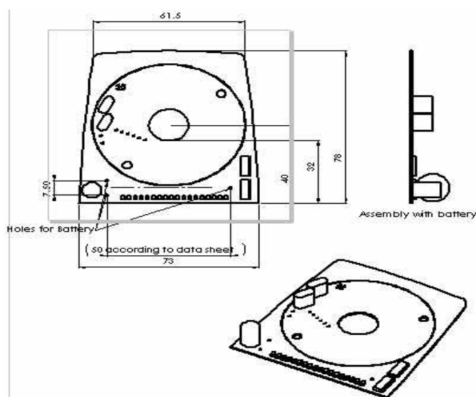
Figure 2: Board Dimension
