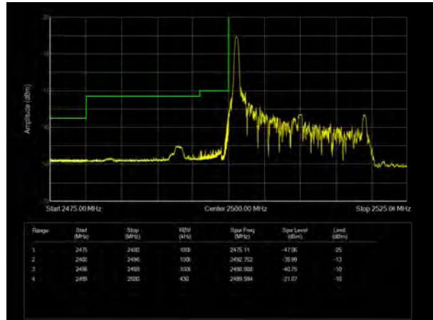
LTE Band 7 QPSK 20MHz CH-Low, 100%RB
