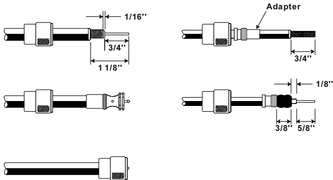
Figure 2.4.0 Installing the VHF antenna
