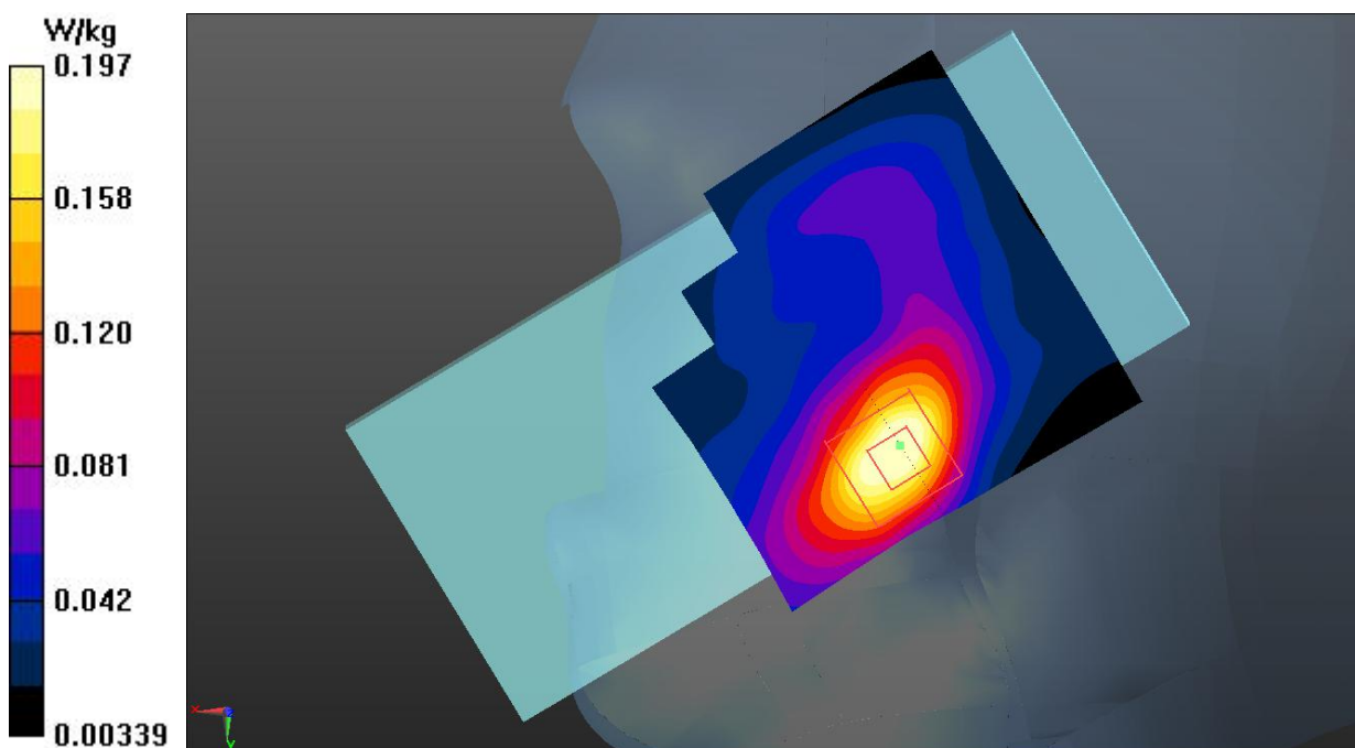
Fig.21 LTE Band 38
