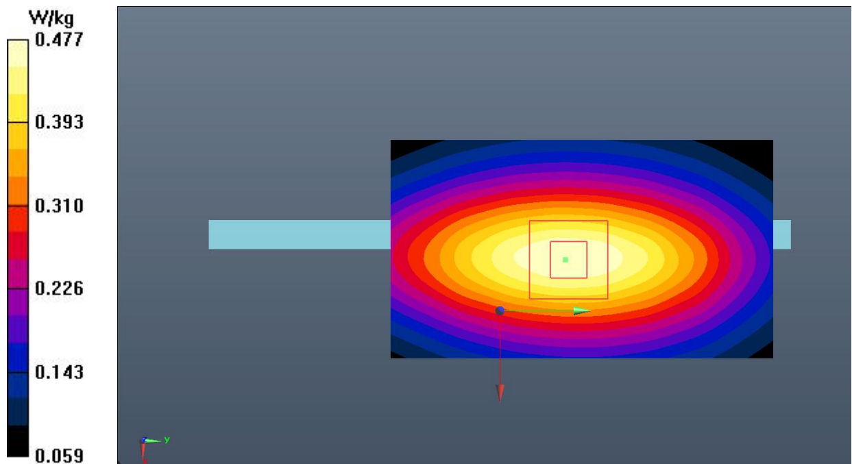
Fig.16 LTE Band 12
