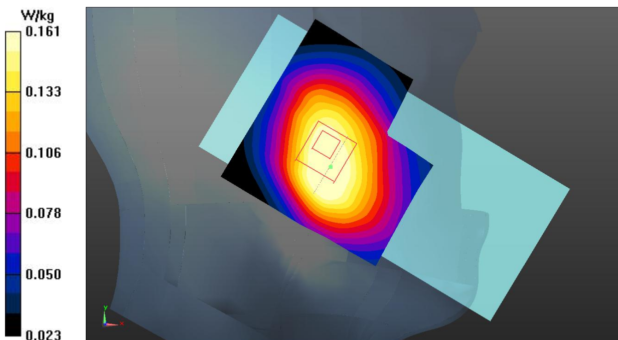
Fig.1 GSM 850
