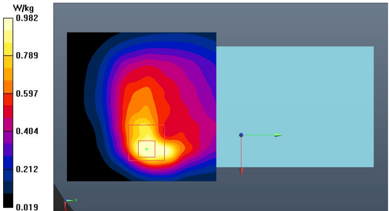
Fig.8 WCDMA Band 4
