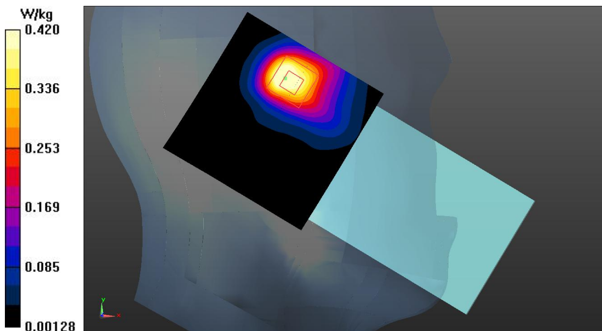
Fig.25 WLAN 2.4G
