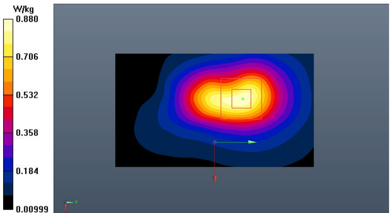
Fig.14 LTE Band 7
