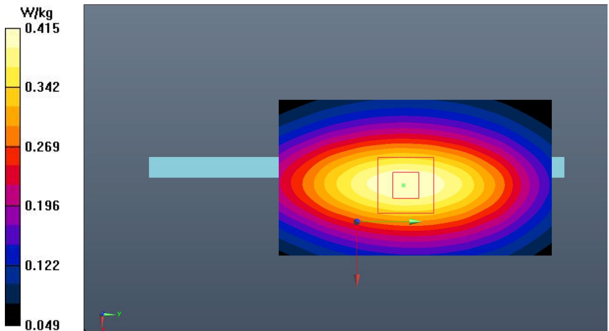
Fig.18 LTE Band 13
