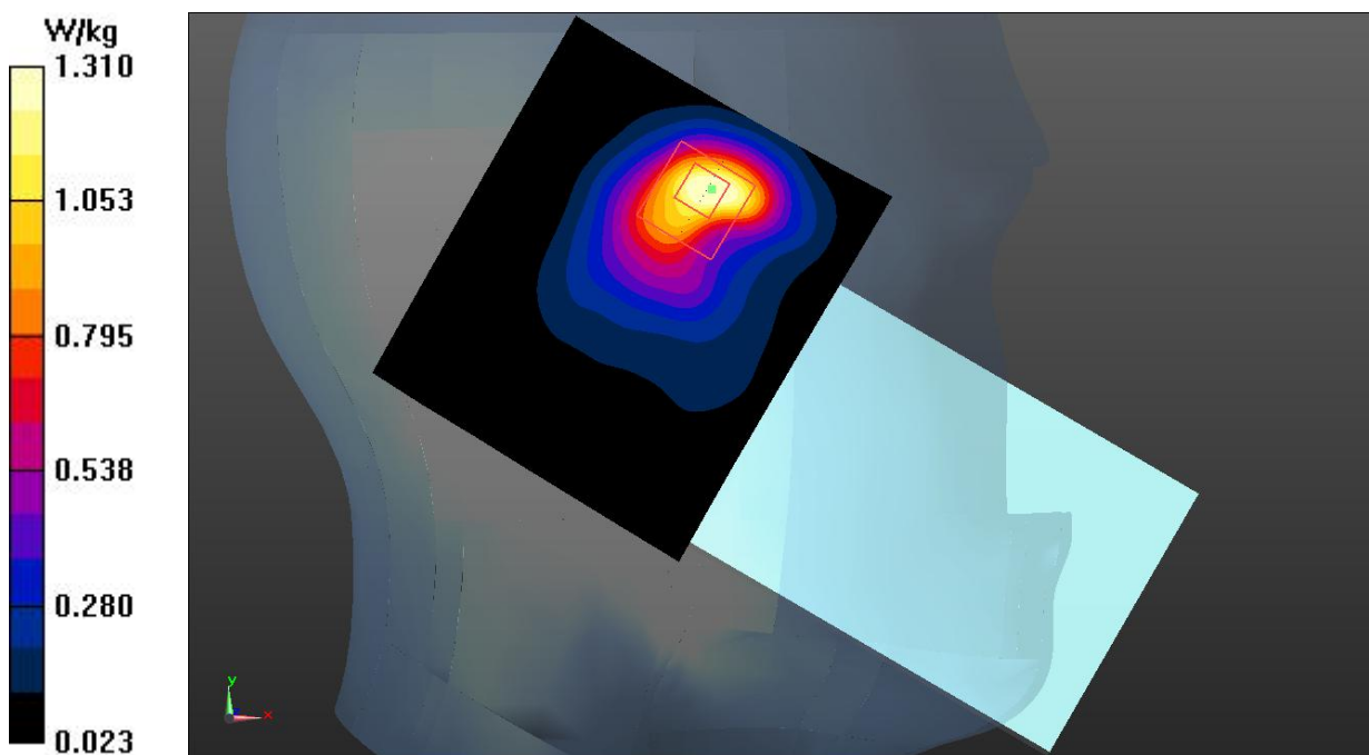
Fig.11 LTE Band 2
