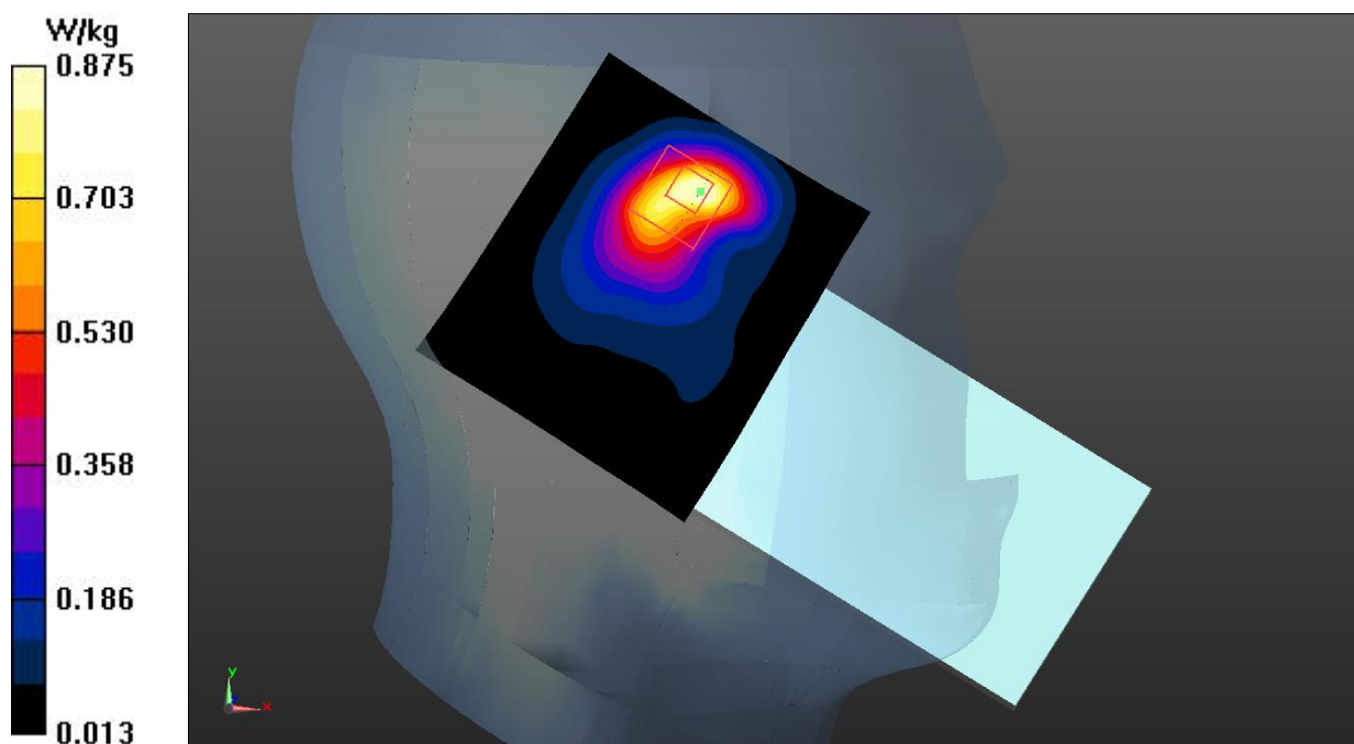
Fig.7 WCDMA Band 4
