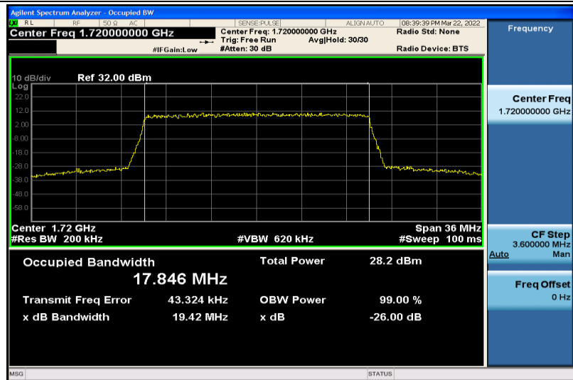
Band4-20MHz-16QAM-20050-100RB#0-17.846
