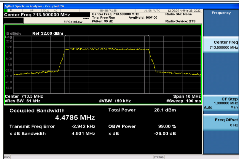
Band17-5MHz-16QAM-23825-25RB#0-4.4785
