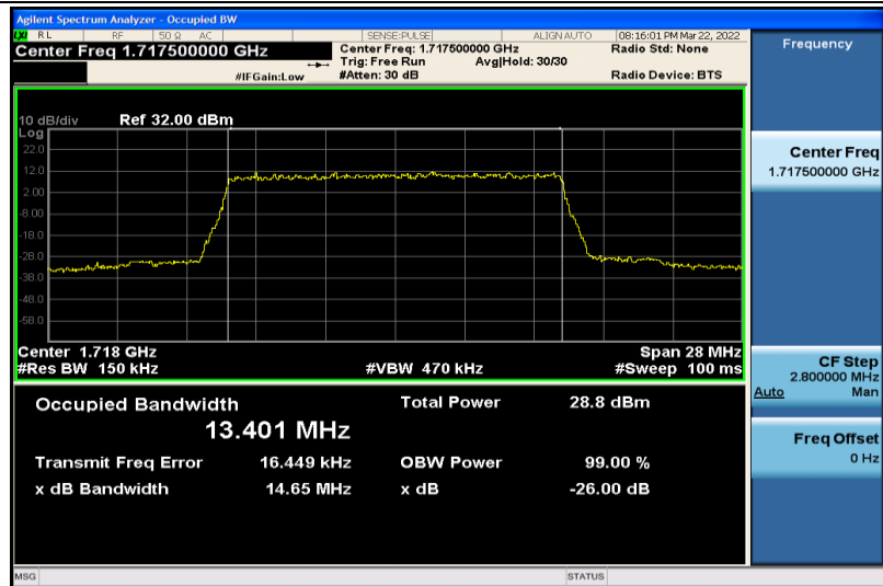
Band4-15MHz-QPSK-20025-75RB#0-13.401
