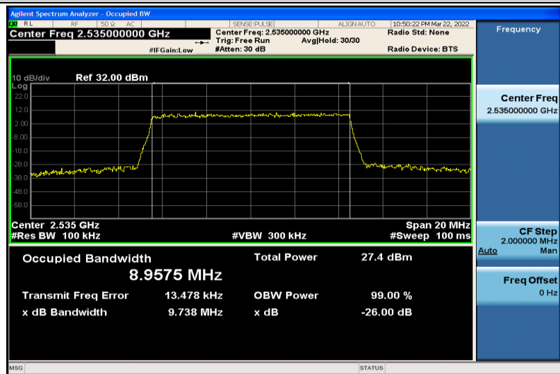
Band7-10MHz-16QAM-21100-50RB#0-8.9575
