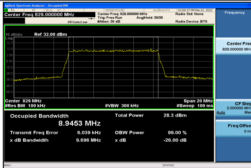
Band5-10MHz-16QAM-20450-50RB#0-8.9453
