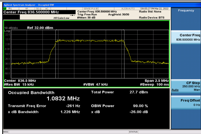
Band5-1.4MHz-16QAM-20525-6RB#0-1.0832
