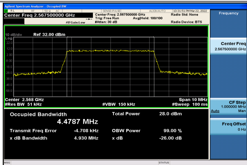
Band7-5MHz-QPSK-21425-25RB#0-4.4787
