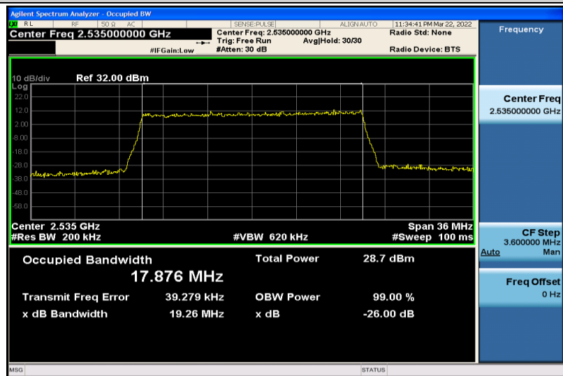
Band7-20MHz-QPSK-21100-100RB#0-17.876
