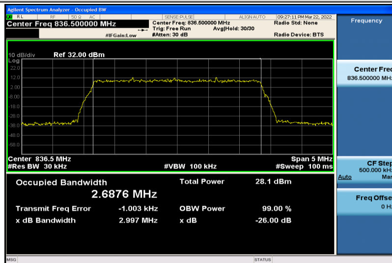
Band5-3MHz-16QAM-20525-15RB#0-2.6876
