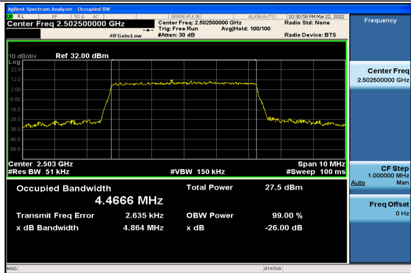
Band7-5MHz-16QAM-20775-25RB#0-4.4666
