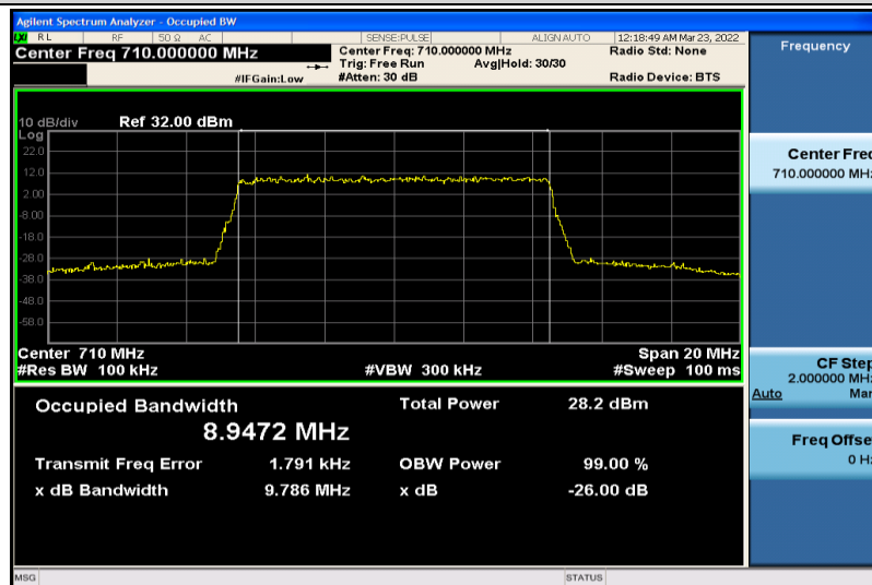
Band17-10MHz-16QAM-23790-50RB#0-8.9472
