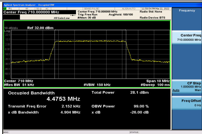
Band17-5MHz-16QAM-23790-25RB#0-4.4753
