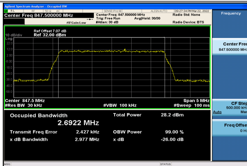
Band5-3MHz-QPSK-20635-15RB#0-2.6922
