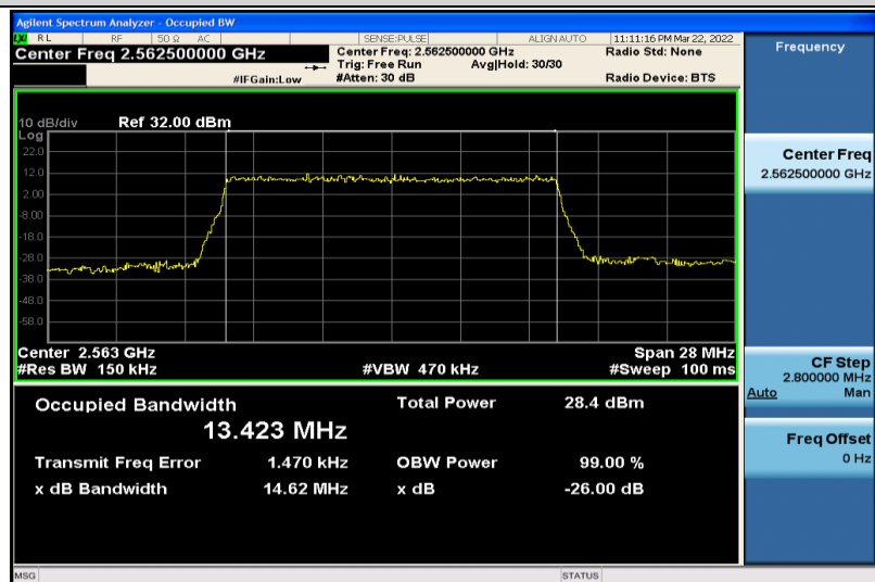
Band7-15MHz-QPSK-21375-75RB#0-13.423
