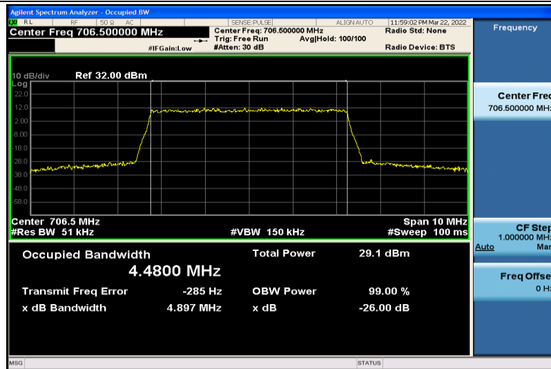
Band17-5MHz-QPSK-23755-25RB#0-4.4800
