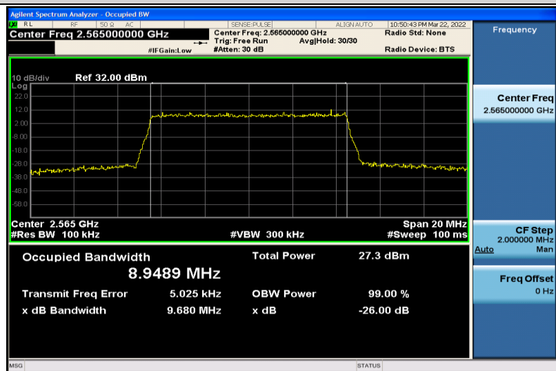
Band7-10MHz-16QAM-21400-50RB#0-8.9489
