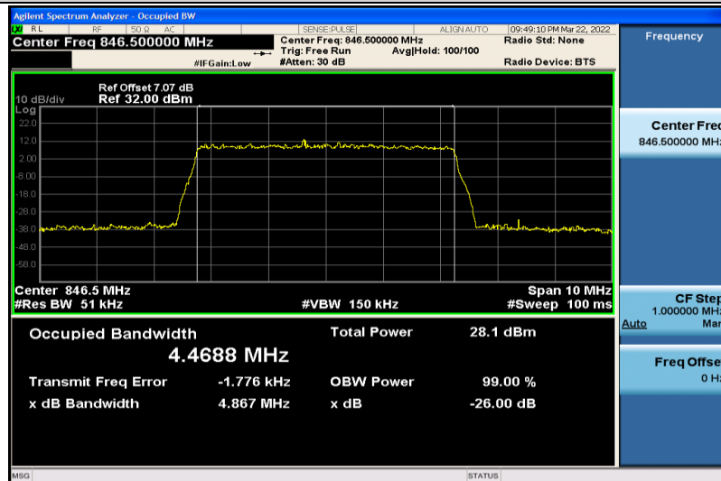
Band5-5MHz-16QAM-20625-25RB#0-4.4688
