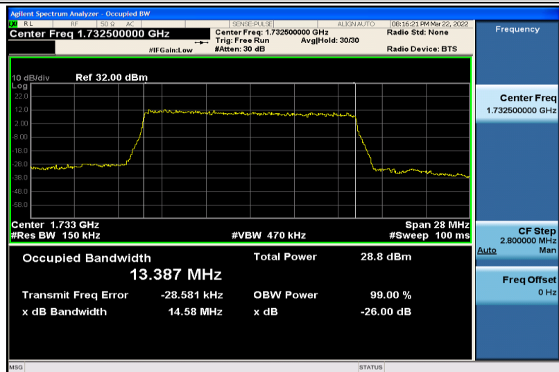
Band4-15MHz-QPSK-20175-75RB#0-13.387
