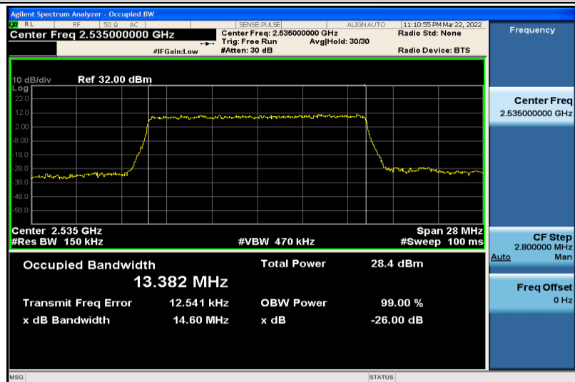
Band7-15MHz-QPSK-21100-75RB#0-13.382
