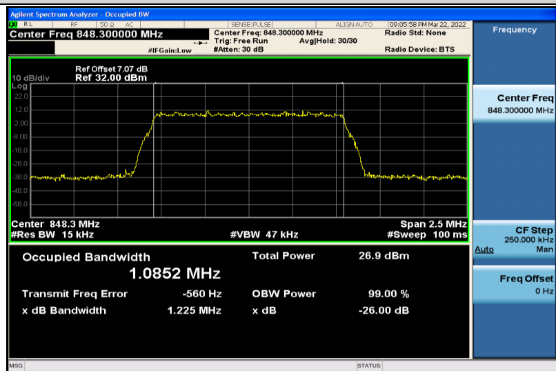
Band5-1.4MHz-16QAM-20643-6RB#0-1.0852
