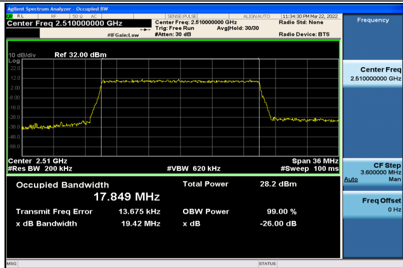
Band7-20MHz-16QAM-20850-100RB#0-17.849
