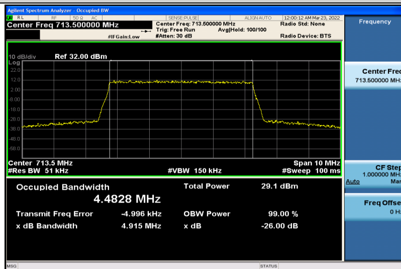
Band17-5MHz-QPSK-23825-25RB#0-4.4828
