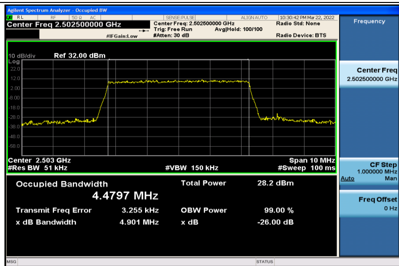
Band7-5MHz-QPSK-20775-25RB#0-4.4797
