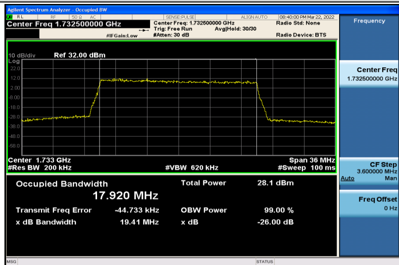
Band4-20MHz-16QAM-20175-100RB#0-17.920
