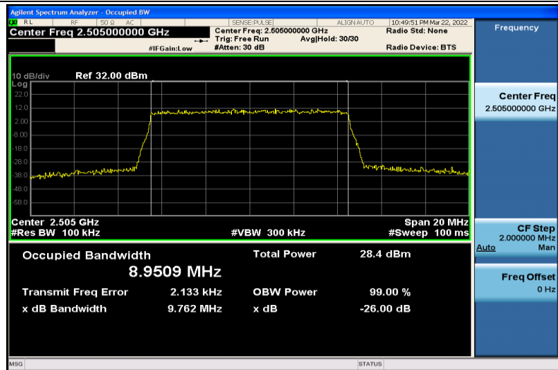
Band7-10MHz-QPSK-20800-50RB#0-8.9509
