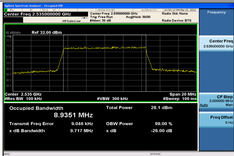
Band7-10MHz-QPSK-21100-50RB#0-8.9351
