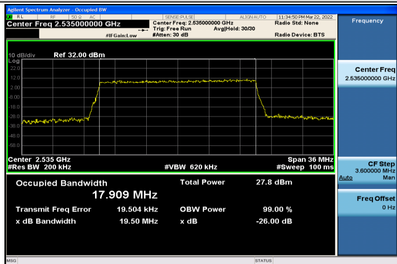
Band7-20MHz-16QAM-21100-100RB#0-17.909
