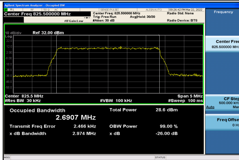
Band5-3MHz-QPSK-20415-15RB#0-2.6907
