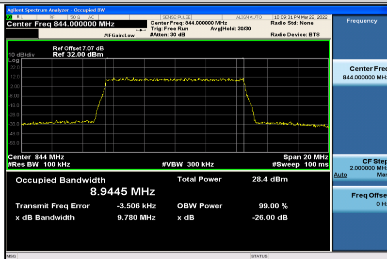
Band5-10MHz-16QAM-20600-50RB#0-8.9445
