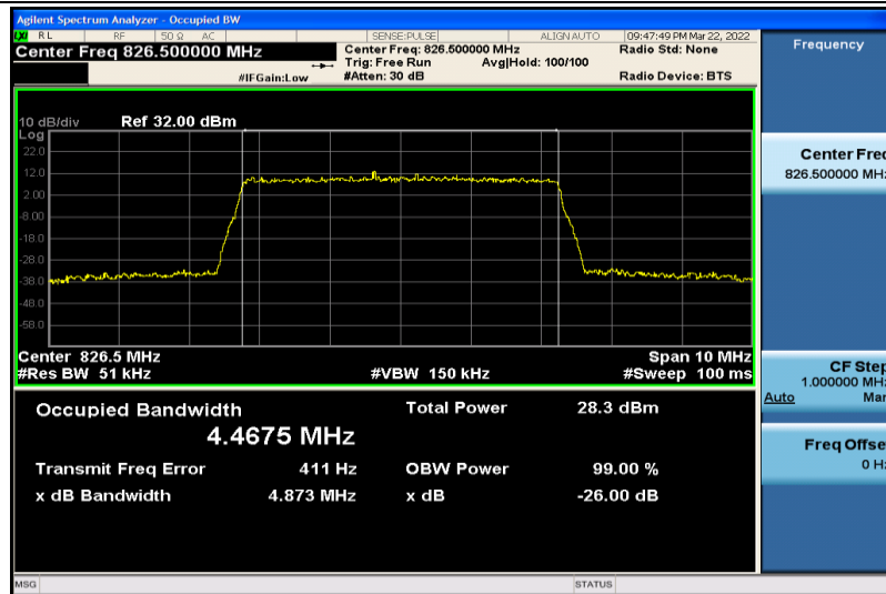
Band5-5MHz-16QAM-20425-25RB#0-4.4675
