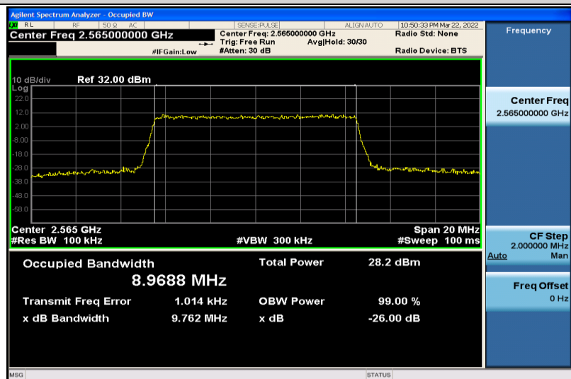
Band7-10MHz-QPSK-21400-50RB#0-8.9688
