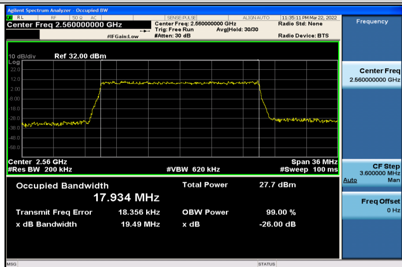
Band7-20MHz-16QAM-21350-100RB#0-17.934
