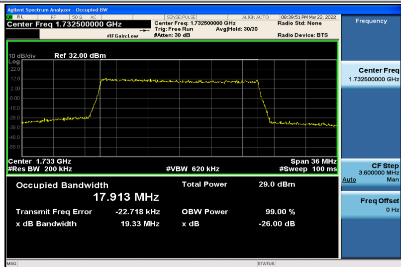
Band4-20MHz-QPSK-20175-100RB#0-17.913
