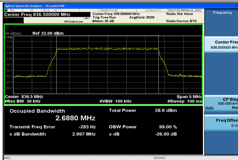
Band5-3MHz-QPSK-20525-15RB#0-2.6880
