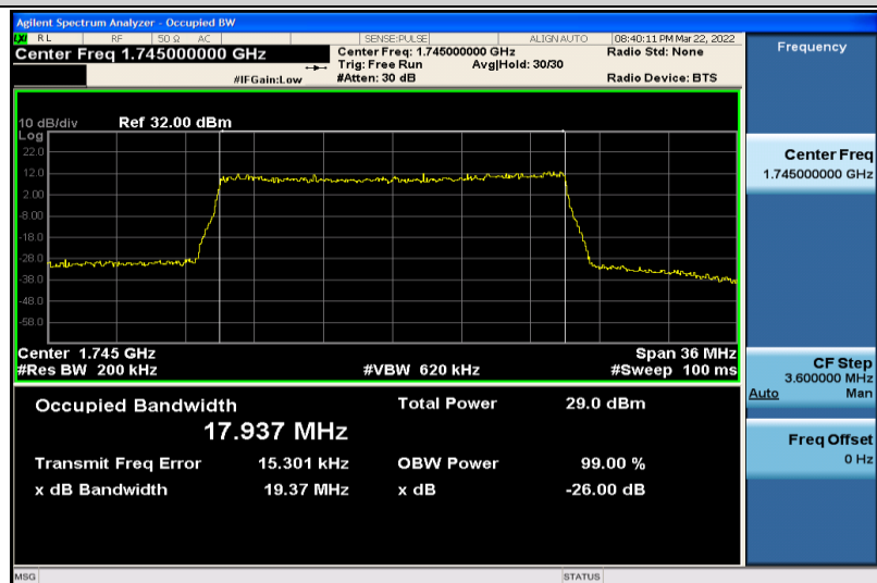
Band4-20MHz-QPSK-20300-100RB#0-17.937
