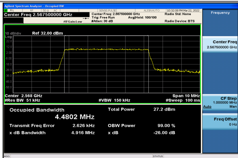
Band7-5MHz-16QAM-21425-25RB#0-4.4802
