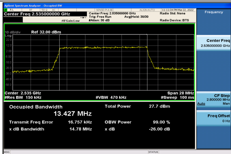
Band7-15MHz-16QAM-21100-75RB#0-13.427
