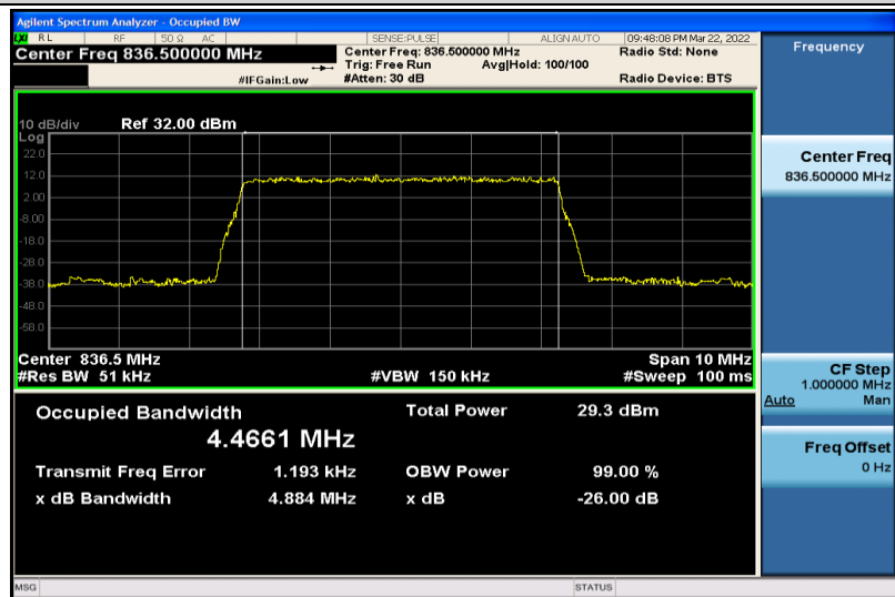
Band5-5MHz-QPSK-20525-25RB#0-4.4661
