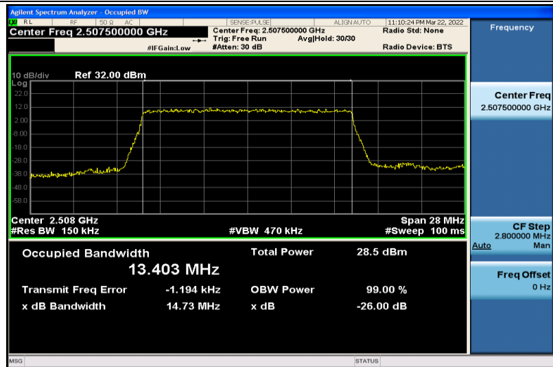
Band7-15MHz-QPSK-20825-75RB#0-13.403
