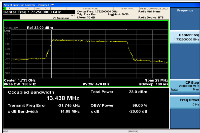
Band4-15MHz-16QAM-20175-75RB#0-13.438
