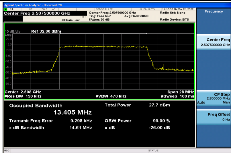
Band7-15MHz-16QAM-20825-75RB#0-13.405
