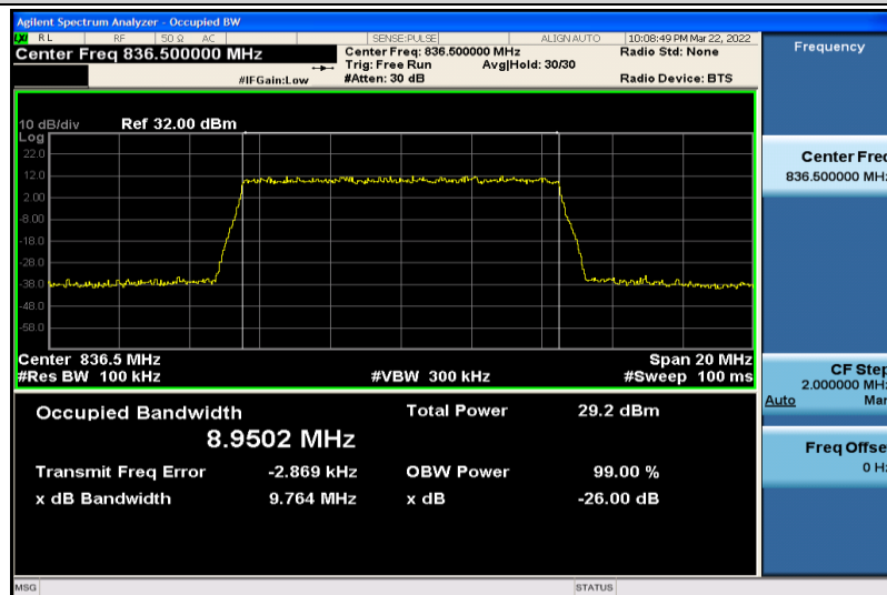
Band5-10MHz-QPSK-20525-50RB#0-8.9502
