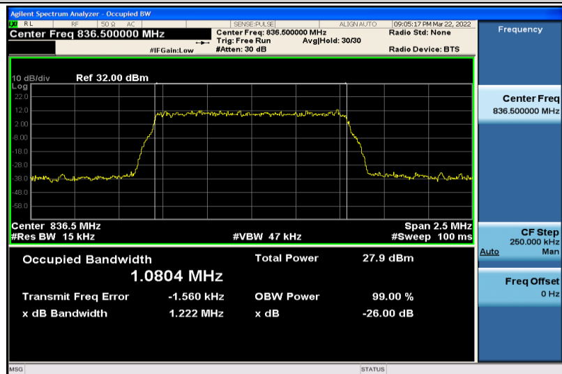
Band5-1.4MHz-QPSK-20525-6RB#0-1.0804
