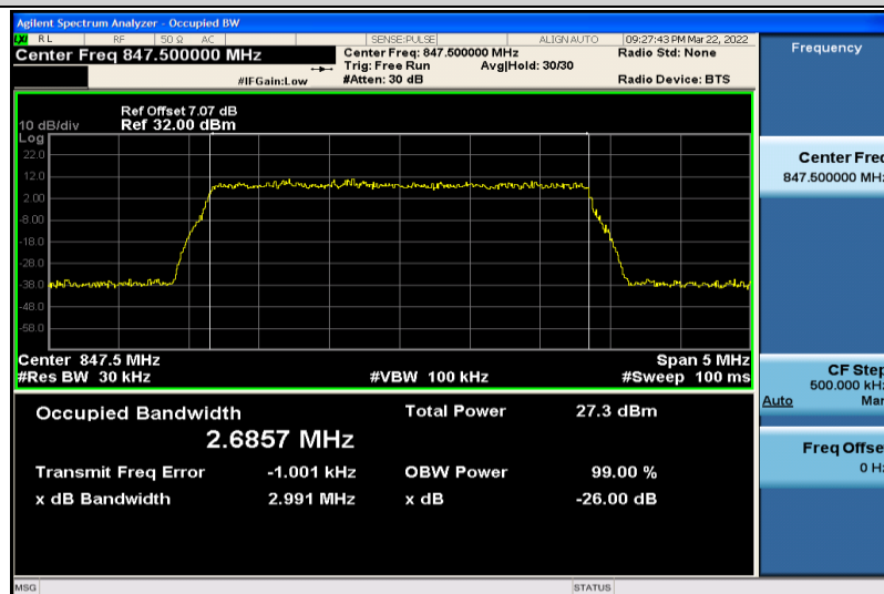
Band5-3MHz-16QAM-20635-15RB#0-2.6857
