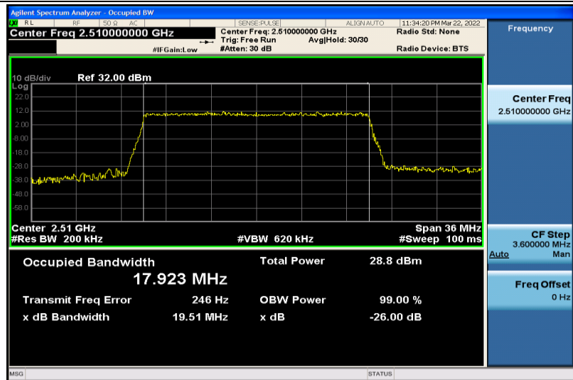
Band7-20MHz-QPSK-20850-100RB#0-17.923
