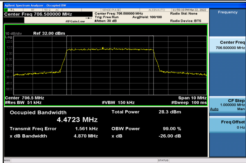
Band17-5MHz-16QAM-23755-25RB#0-4.4723
