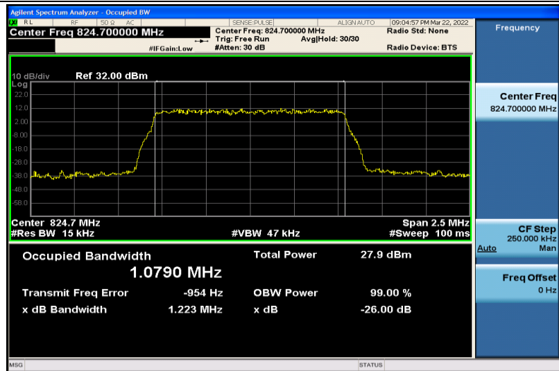
Band5-1.4MHz-QPSK-20407-6RB#0-1.0790
