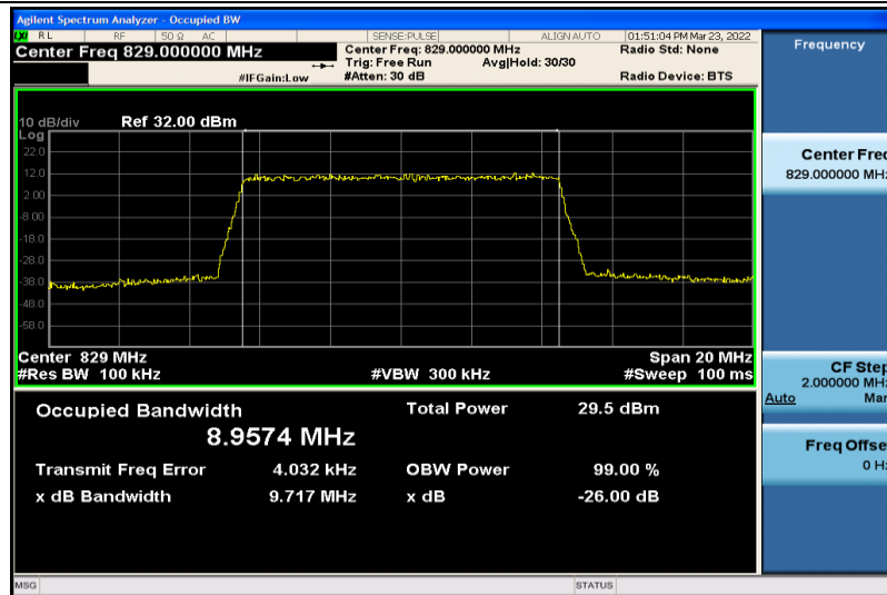
Band5-10MHz-QPSK-20450-50RB#0-8.9574
