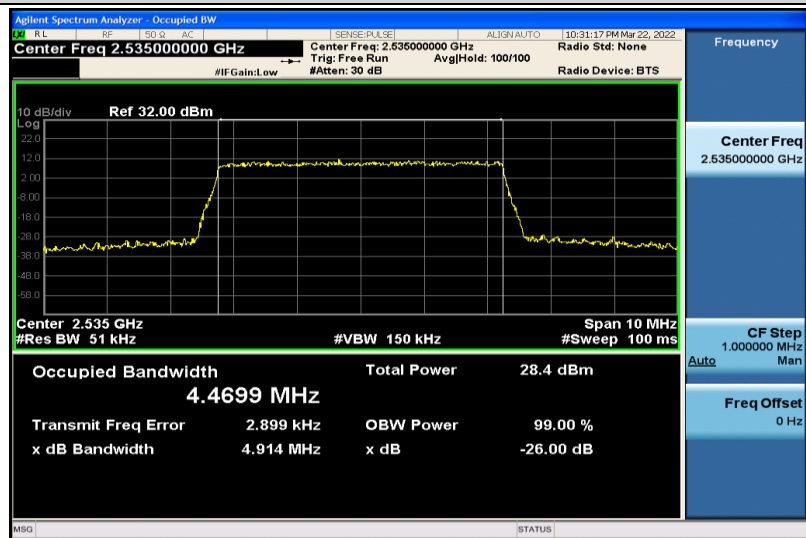
Band7-5MHz-QPSK-21100-25RB#0-4.4699
