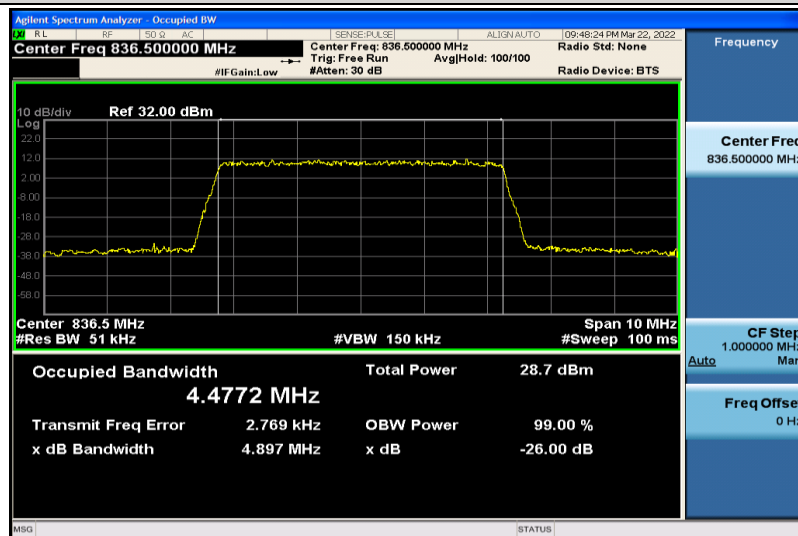
Band5-5MHz-16QAM-20525-25RB#0-4.4772
