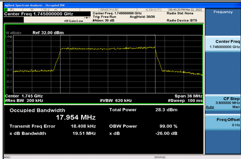
Band4-20MHz-16QAM-20300-100RB#0-17.954
