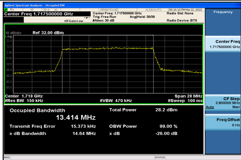
Band4-15MHz-16QAM-20025-75RB#0-13.414
