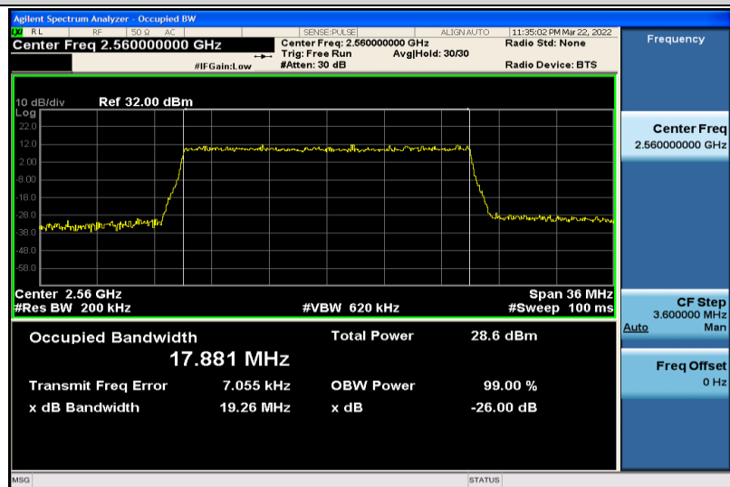
Band7-20MHz-QPSK-21350-100RB#0-17.881
