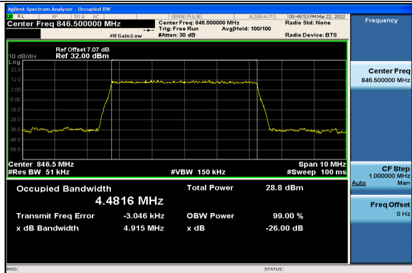
Band5-5MHz-QPSK-20625-25RB#0-4.4816
