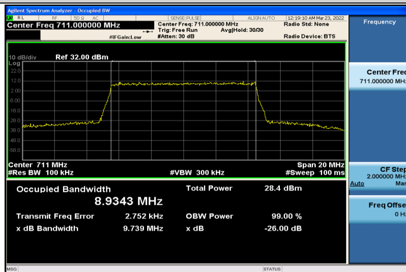
Band17-10MHz-16QAM-23800-50RB#0-8.9343
