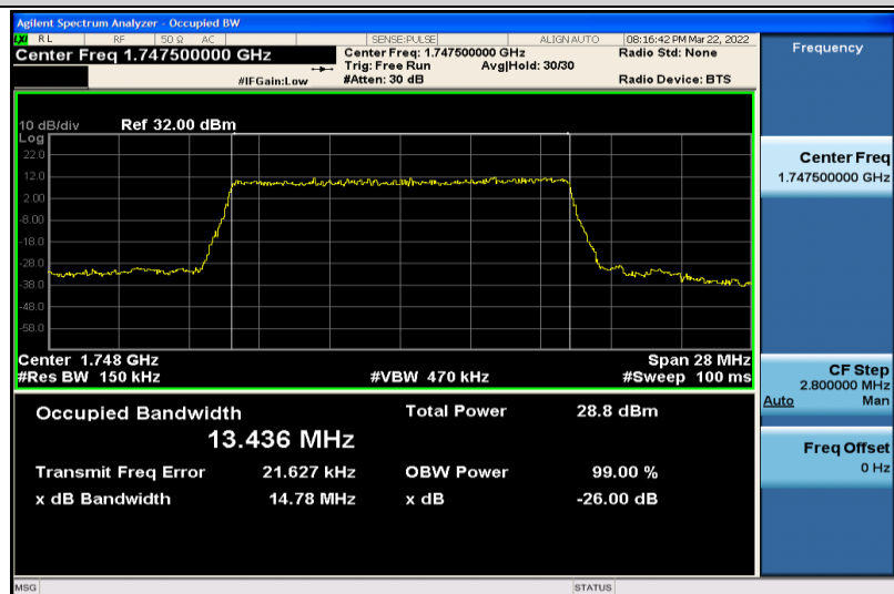
Band4-15MHz-QPSK-20325-75RB#0-13.436
