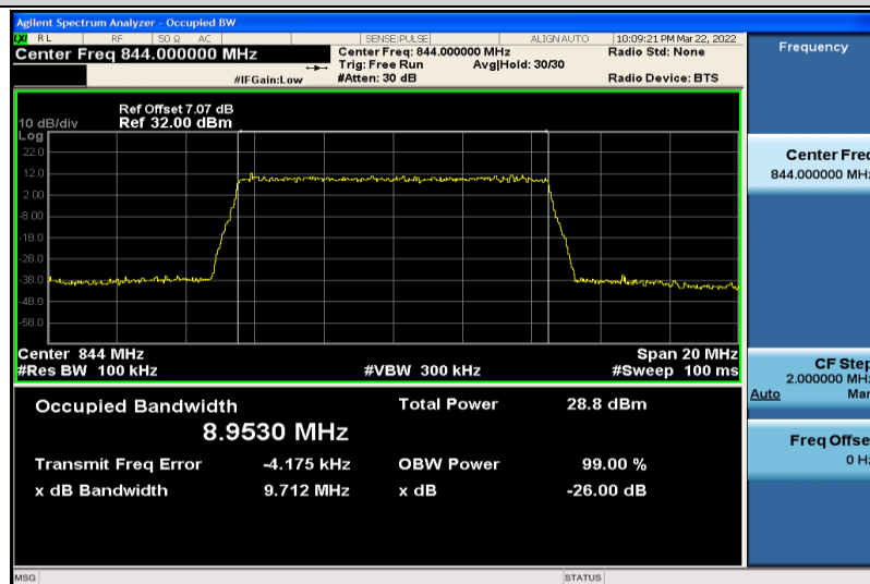
Band5-10MHz-QPSK-20600-50RB#0-8.9530
