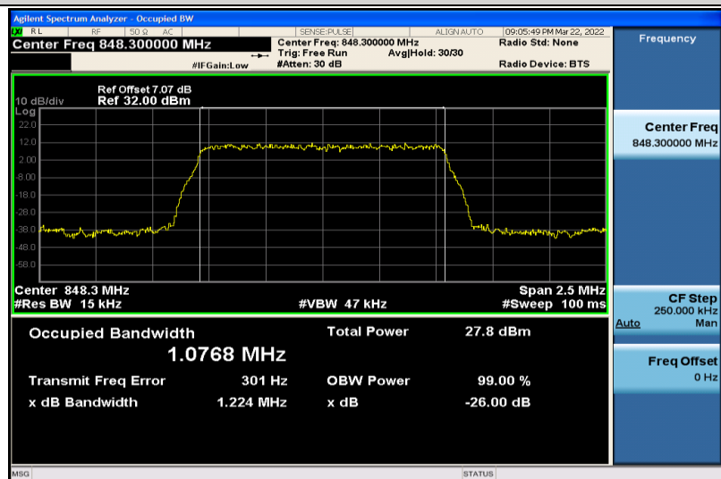
Band5-1.4MHz-QPSK-20643-6RB#0-1.0768
