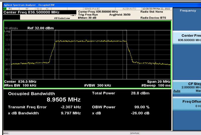
Band5-10MHz-16QAM-20525-50RB#0-8.9505
