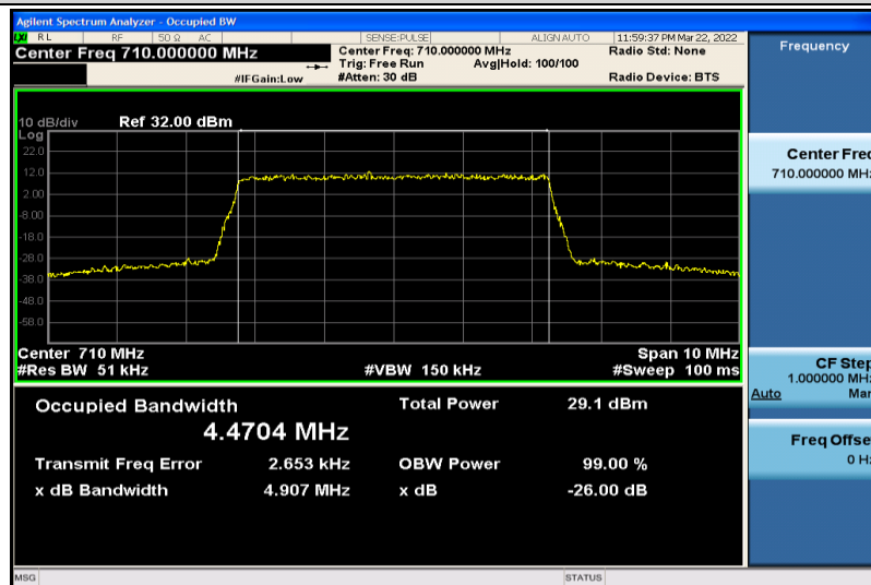
Band17-5MHz-QPSK-23790-25RB#0-4.4704
