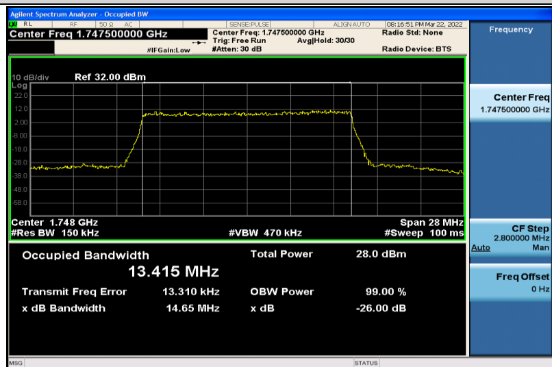
Band4-15MHz-16QAM-20325-75RB#0-13.415
