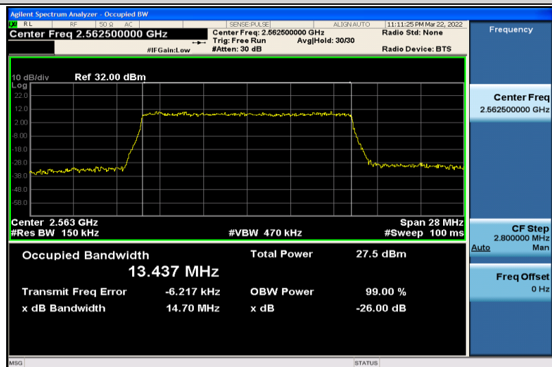
Band7-15MHz-16QAM-21375-75RB#0-13.437
