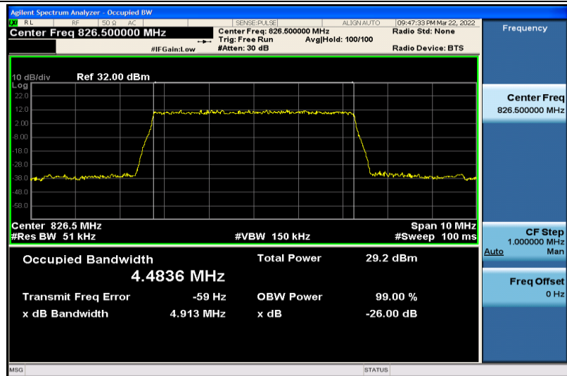
Band5-5MHz-QPSK-20425-25RB#0-4.4836
