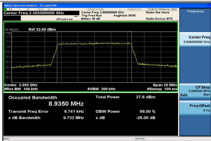
Band7-10MHz-16QAM-20800-50RB#0-8.9350
